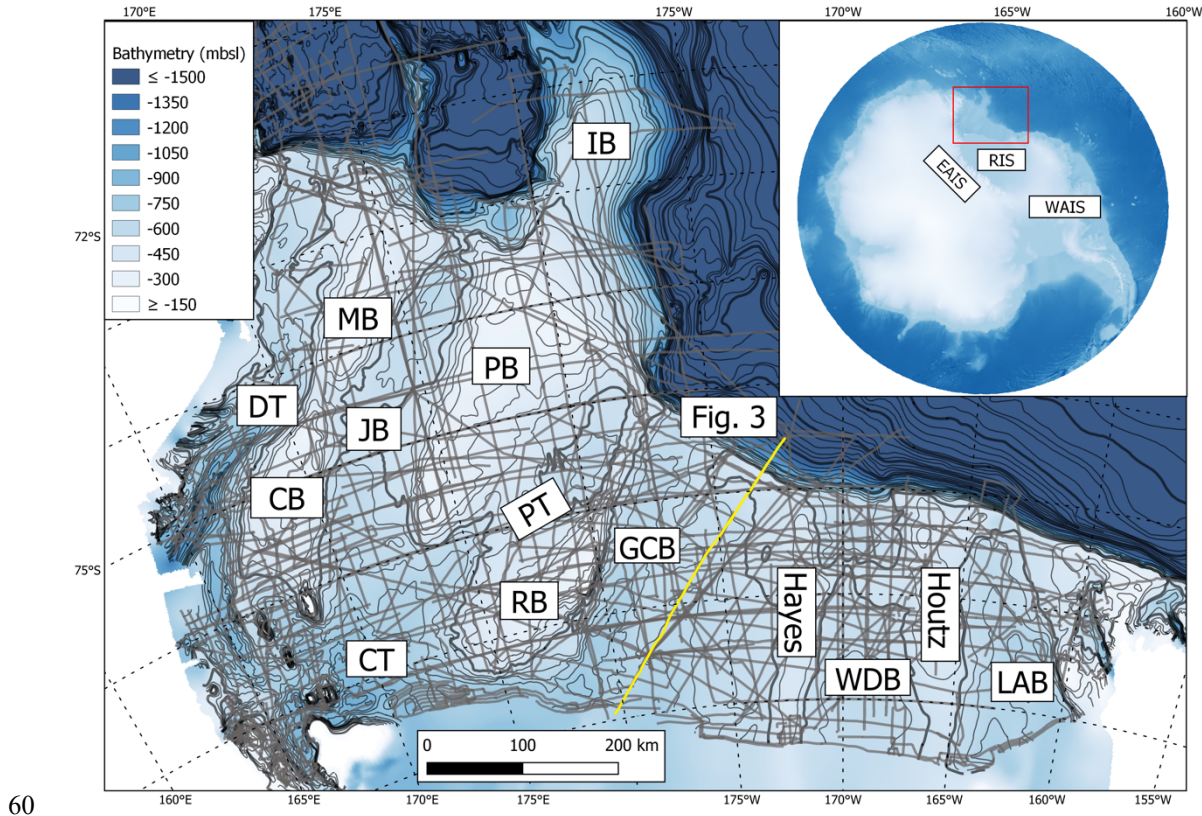
Figure 1: Map of the Ross Sea showing seismic coverage. Bathymetry is from Davey and Nitsche (2013). Inset map of Antarctica using the International Bathymetric Chart of the Southern Ocean ice surface and bathymetry grid showing the locations of the East Antarctic Ice Sheet (EAIS) and the West Antarctic Ice Sheet (WAIS) in addition to the position of the Ross Ice Shelf (RIS) (Dorschel et al., 2022). Main map shows Ross Sea as indicated by the red box on the inset map. Labels of bathymetric troughs on the Ross Sea shelf follow: LAB = Little America Basin, WDB = Whales Deep Basin, GCB = Glomar Challenger Basin, PT = Pennell Trough, CT = Central Trough, JB = JOIDES Basin, DT = Drygalski Trough. Labels of bathymetric banks on the Ross Sea shelf follow: Houtz = Houtz Bank, Hayes = Hayes Bank, RB = Ross Bank, PB = Pennell Bank, IB = Iselin Bank, MB = Mawson Bank, CB = Crary Bank. The position of the Figure 3 seismic profile is indicated with the yellow line.
