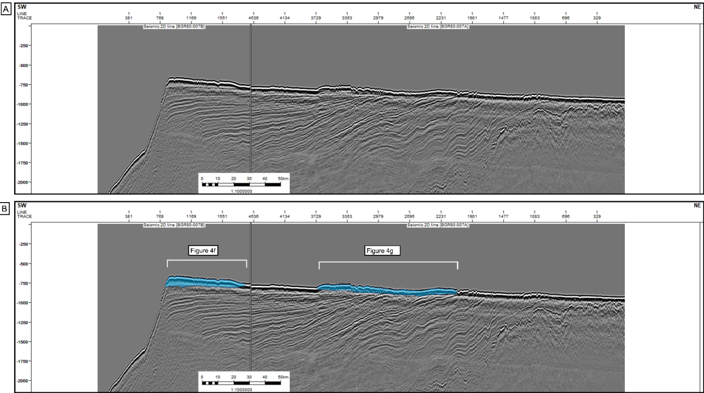
165 Figure 3: Uninterpreted (A) and interpreted (B) seismic line BGR80-007 through GCB. Location of line is indicated with Figure 1. Blue shaded region shows interpreted GZW's. Position of GZW's and thickness map are shown in Figure 4.
