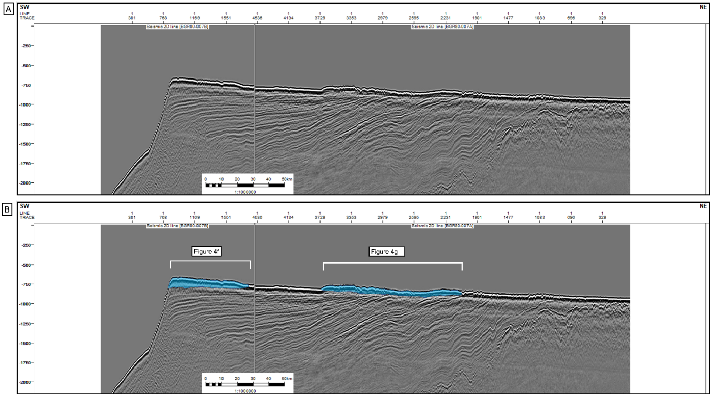
165 Figure 3: Uninterpreted (A) and interpreted (B) seismic line BGR80-007 through GCB. Location of line is indicated with Figure 1. Blue shaded region shows interpreted GZWs. Position of GZWs and thickness map are shown in Figure 4.
