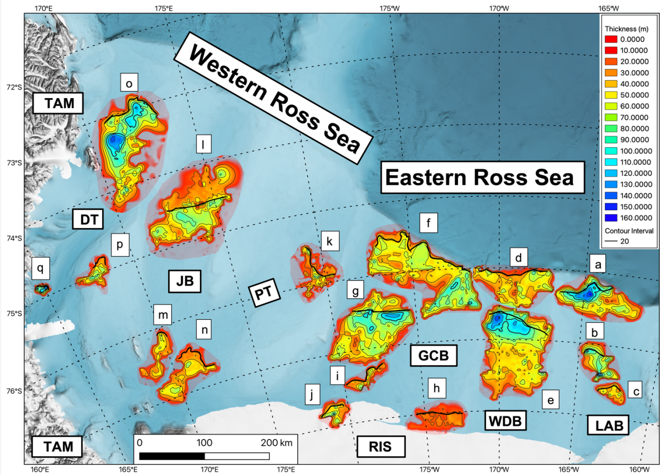
170 Figure 4: Thicknesses contour maps of Ross Sea GZWs. The heavy black line shows the approximate location of boundary between the GZW topset and foreset. GZWs are labeled “a” to “q” starting in the east with LAB outer shelf GZW. Letter labels of GZWs correspond with records in Table 1. Labels of geometric features follow: LAB = Little America Basin, WDB = Whales Deep Basin, GCB = Glomar Challenger Basin, PT = Pennell Trough, CT = Central Trough, JB = JOIDES Basin, DT = Drygalski Trough, TAM = Transantarctic Mountains, RIS = Ross Ice Shelf. Bathymetry shown in the base map is from IBSCO v2 (Dorschel et al., 2022).. Contour interval = 20 m
