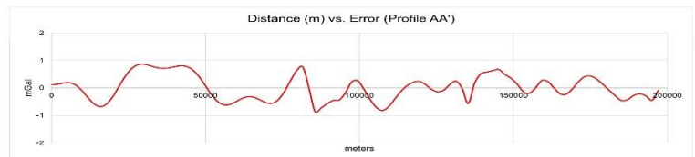
755 Figure 7: Observed complete Bouguer anomaly data (Fig. 3) and calculated Bouguer gravity responses (upper panel) with the computed density models (lower panel) along the AA' profile (Fig. 1b). Corresponding distance vs misfit error along profile AA' is shown below as a separate panel.
