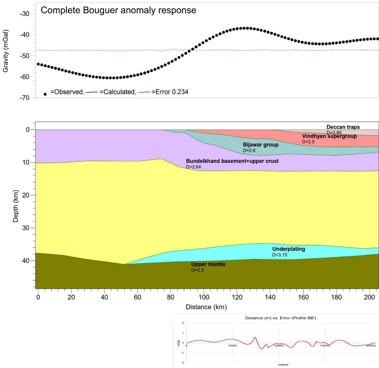
Figure 8: Observed complete Bouguer anomaly data (Fig. 3) and calculated Bouguer gravity responses (upper panel) with the computed density models (lower panel) along the BB' profile (Fig. 1b). Corresponding distance vs misfit error along profile BB' is shown below as a separate panel.
