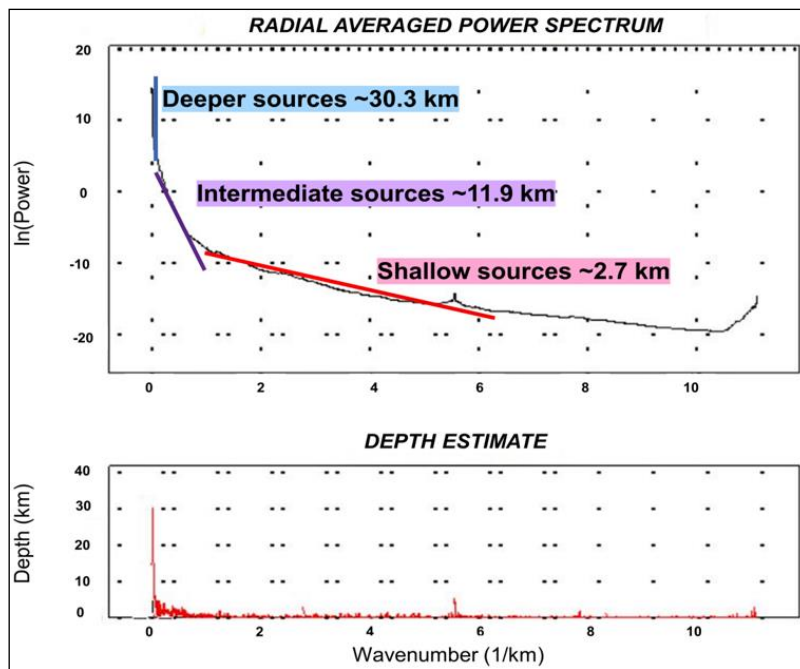
Figure 5: Radially averaged power spectrum plot (upper panel) with the corresponding depth estimates plot (lower panel) for the complete Bouguer anomaly data (Fig. 3).
