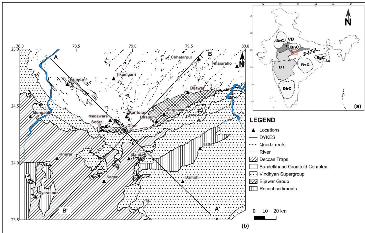
715 Figure 1: (a) Position of the Bundelkhand craton and Vindhyan basin with respect to other major cratons of the Indian subcontinent. Bijawar basin forms the base of the Vindhyan basin, and the exposed sequences are shown in Figure 1b. [ArC- Aravalli Craton, BnC- Bundelkhand Craton, VB- Vindhyan Basin, DT- Deccan Traps, DhC- Dharwar Craton, BsC- Bastar Craton, SgC- Singhbhum Craton, C.I.T.Z.- Central Indian Tectonic Zone] (b) General geological setup of the region used for the regional scale study of the craton and surrounding areas along the southern boundary of the craton. The two profiles used for gravity modelling are marked here as AA' and BB'. (Data source: GSI Bhukosh platform, https://bhukosh.gsi.gov.in/ )
