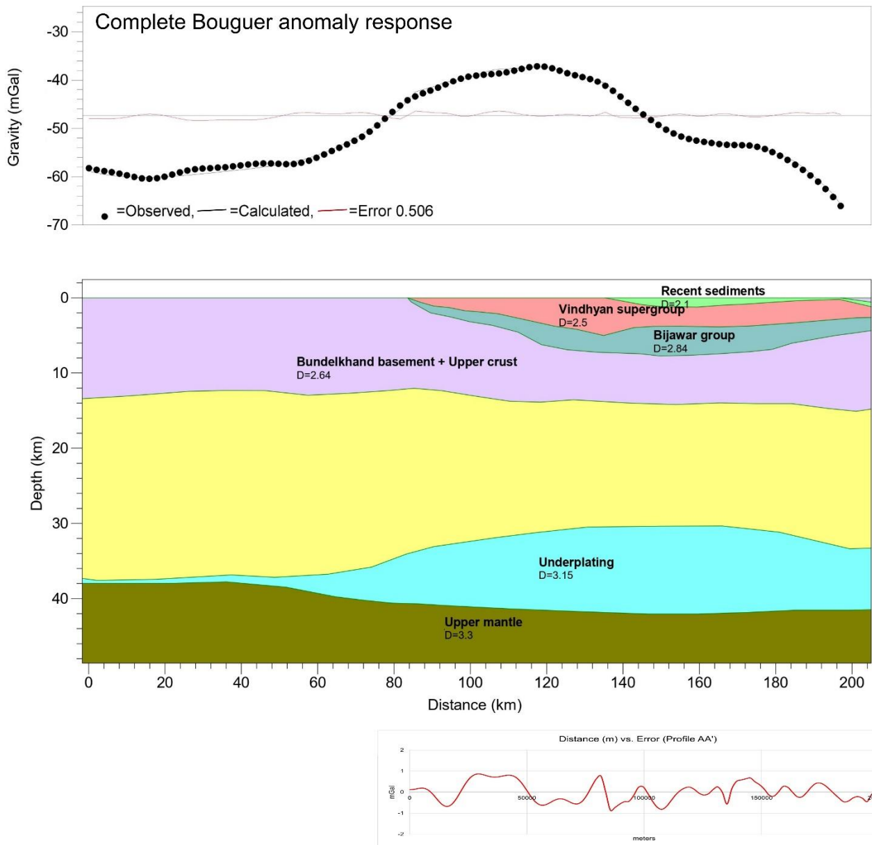
755 Figure 7: Observed complete Bouguer anomaly data (Fig. 3) and calculated Bouguer gravity responses (upper panel) with the computed density models (lower panel) along the AA' profile (Fig. 1b). Corresponding distance vs misfit error along profile AA' is shown below as a separate panel.
