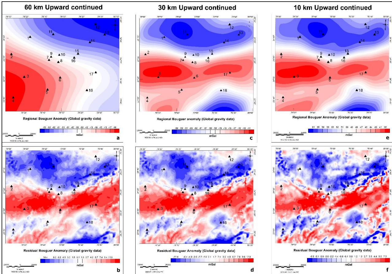
735 Figure 4: (a) Regional gravity anomaly map of the global gravity data, upward continued up to 60 km, (b) Residual gravity anomaly map of the global grid data, obtained after subtracting the 60 km upward continued regional gravity anomaly from complete Bouguer anomaly. (c) Regional gravity anomaly map of the global gravity data, upward continued up to 30 km, (d) Residual gravity anomaly map of the global grid data, obtained after subtracting the 30 km upward continued regional gravity anomaly from complete Bouguer anomaly. (e) Regional gravity anomaly map of the global gravity data, upward continued up to 10 km, (f) Residual gravity anomaly map of the global grid data, obtained after subtracting the 10 km upward continued regional gravity anomaly from complete Bouguer anomaly. Locations: (1)Lalitpur, (2)Mungaoli, (3)Khurai, (4)Gyaraspur, (5)Sagar, (6)Banda, (7)Sonrai, (8)Girar, (9)Madawara, (10)Karitoran, (11)Tikamgarh, (12)Chhatarpur, (13)Khajuraho, (14)Bijawar, (15)Dargawan, (16)Hirapur, (17)Hatta, (18)Damoh. 740
