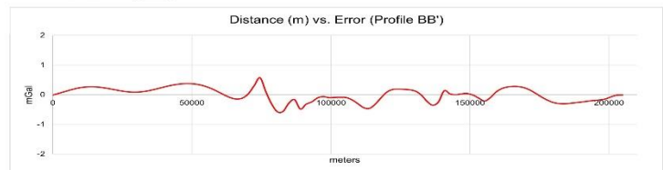
Figure 8: Observed complete Bouguer anomaly data (Fig. 3) and calculated Bouguer gravity responses (upper panel) with the computed density models (lower panel) along the BB' profile (Fig. 1b). Corresponding distance vs misfit error along profile BB' is shown below as a separate panel.
