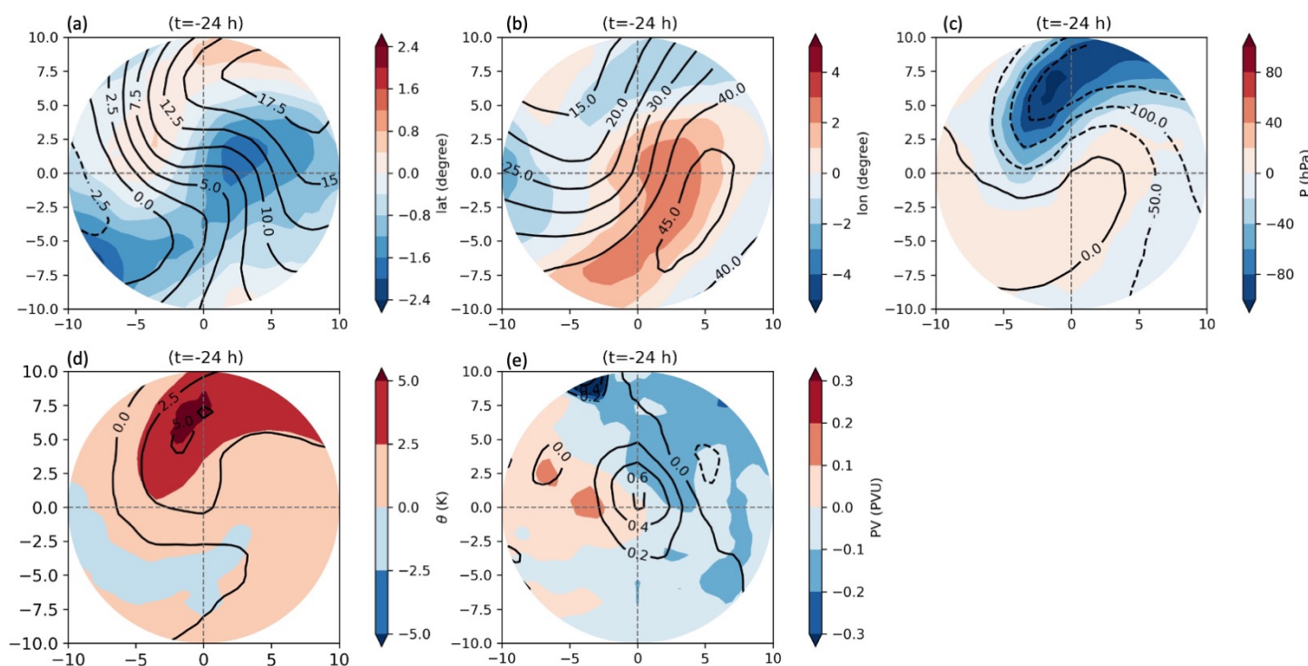
Figure 7. Composites of Lagrangian tendencies along backward trajectories initialized at 250 hPa in the last 24 hours before arrival in the cyclone area of (a) latitude, (b) longitude, (c) pressure, (d) potential temperature and (e) PV. Contours show present-day Lagrangian tendencies and the color shading indicates the response to future climate change (difference in the Lagrangian tendencies between future and present-day climate).
