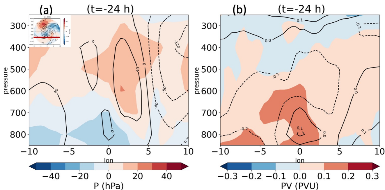
Figure 10. West-east vertical cross section through the dry intrusion region 4^\circ south of the cyclone center. Contours show present-day Lagrangian tendencies along backward trajectories in the last 24 hours before arrival in the cyclone area of (a) pressure and (b) PV. Color shading shows the response to future climate change.
