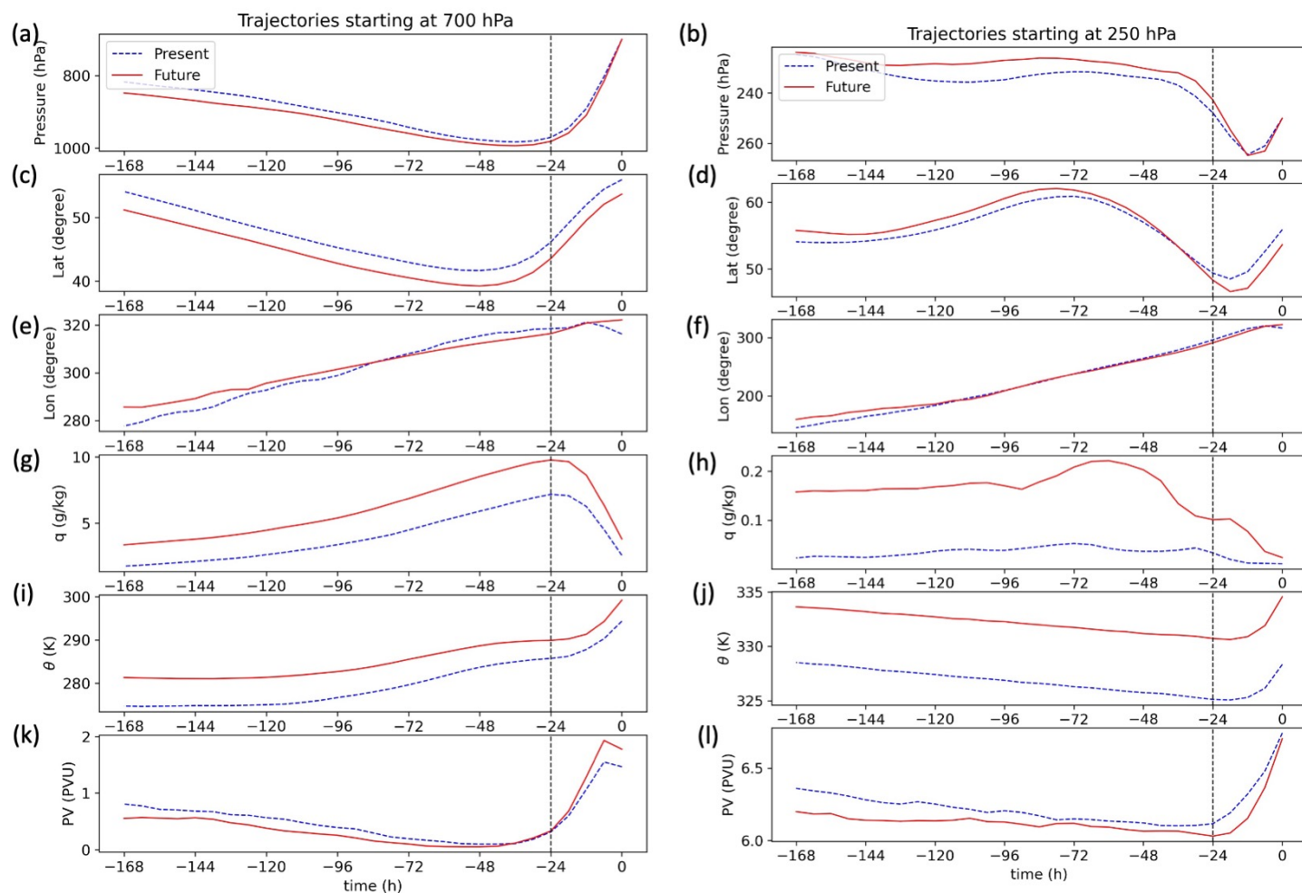
Figure 5. Temporal evolution of (a,b) pressure, (c,d) latitude, (e,f) longitude, (g,h) specific humidity, (i,j) potential temperature and (k,l) PV averages along backward trajectories initialized at the cyclone center and at (left column) 700 hPa and (right column) 250 hPa.
