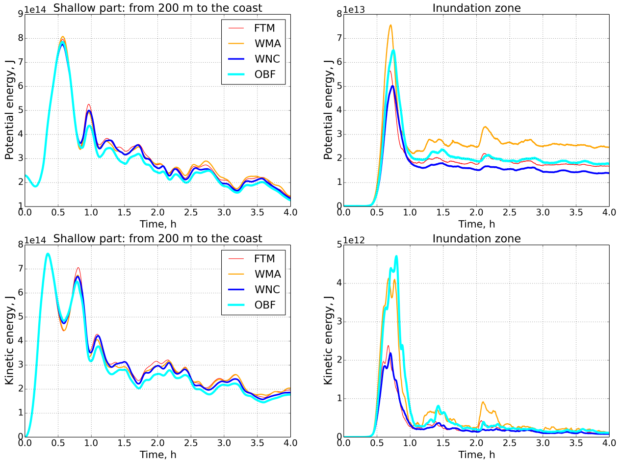
Figure 10. Potential and kinetic energy for four experiments for shelf zone and inundation area. Upper panel - potential energy; bottom panel - kinetic energy; left - shelf zone (from 200 m to coast); right - inundation area.
