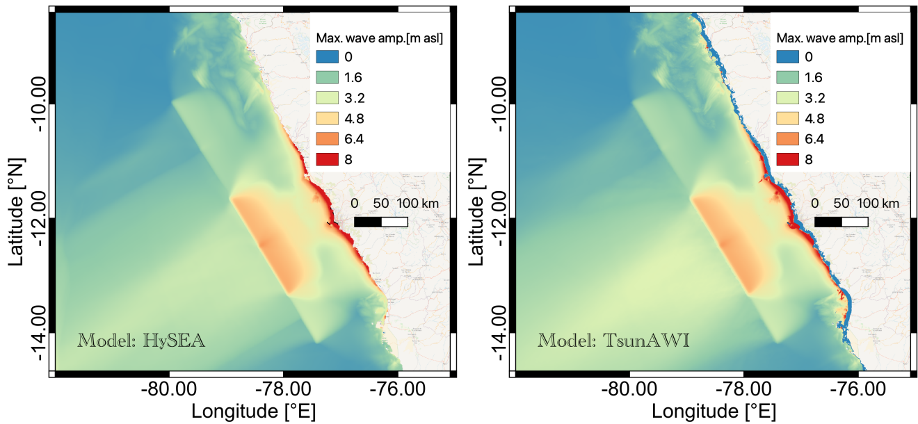
Figure 5. Maximum wave amplitude (in [m asl.]) for a simulation of four hours propagation time in the models Tsunami-HySEA (left panel) and TsunAWI (right panel). Basemap: © OpenStreetMap contributors 2021. Distributed under the Open Data Commons Open Database License (ODbL) v1.0.
