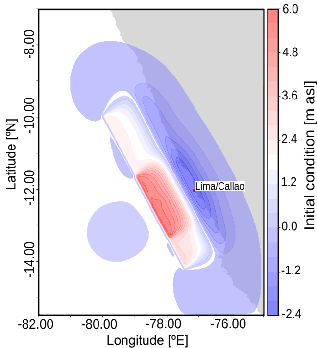
Figure 4. Initial conditions for the tsunami numerical simulations used by both models. Parameters modified from Jimenez et al. (2013). Values are given in meters relative to average sea level (m asl).
