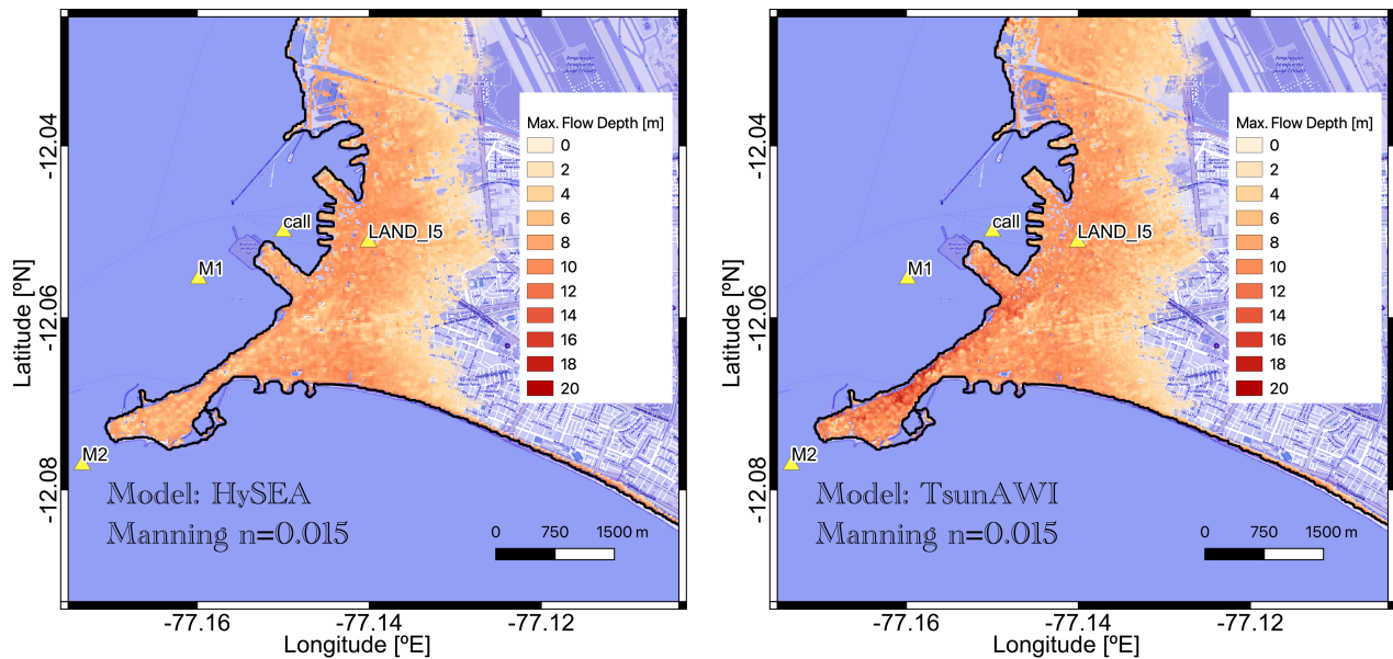
Figure A1. Maximum flow depth (in [m] relative to topography) in La Punta and the Callao port area for simulations of four hours propagation in Tsunami-HySEA (left panel) and TsunAWI (right panel). Basemap: © OpenStreetMap contributors 2021. Distributed under the Open Data Commons Open Database License (ODbL) v1.0.
