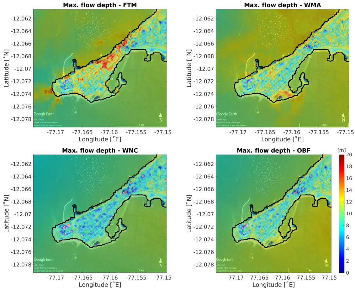
Figure 11. Maximum sea surface amplitude in the ocean (in [m asl.]) and flow depth (in [m] relative to topography) for the complete simulation period. Upper left panel: Full model (FTM); upper right: Without momentum advection (WMA); lower left: Omitting nonlinearity in the continuity equation (WNC); lower right: Only bottom friction (OBF). Basemap: © Google Earth 2018.
