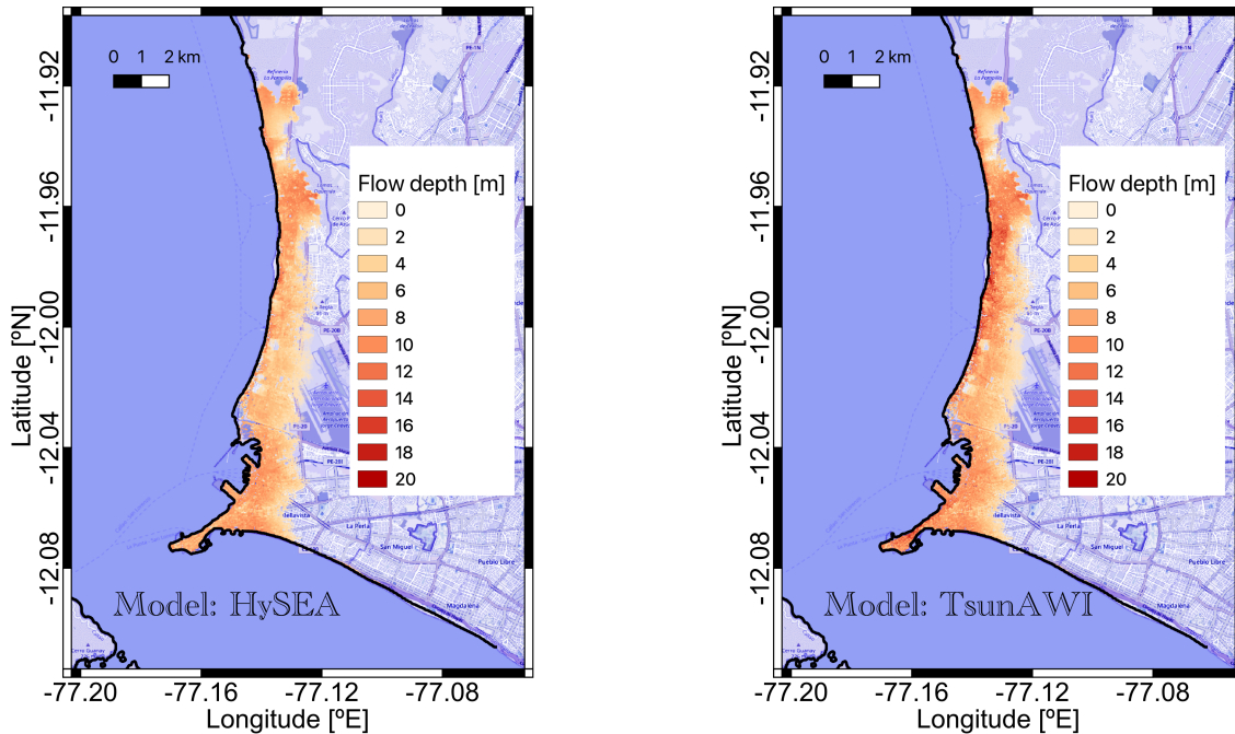
Figure 6. Maximum flow depth (in [m] relative to topography) in the inundated area in Callao obtained by Tsunami-HySEA (left panel) and TsunAWI (right panel) for a Manning value of n = 0.015 and a simulation time of four hours. The box indicates the area in which the inundation extent and inundation properties were calculated. Basemap: © OpenStreetMap contributors 2021. Distributed under the Open Data Commons Open Database License (ODbL) v1.0.
