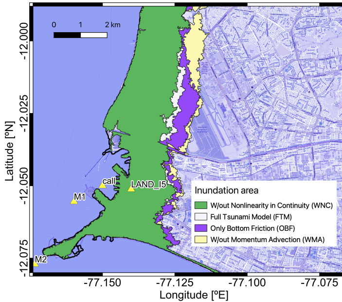
Figure 14. Inundation area obtained with TsunAWI for the experiments with the deactivation of different nonlinear terms. Basemap: © Open-StreetMap contributors 2021. Distributed under the Open Data Commons Open Database License (ODbL) v1.0.
