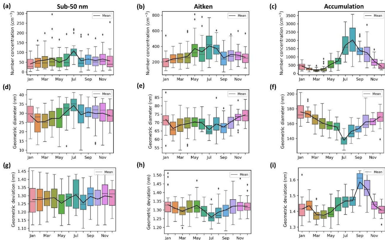
Figure S2. Monthly boxplot of each parameter of the multi-modal lognormal fit. The modes are shown in each column and the parameters number concentration ( N ), geometric diameter ( D_g ), and standard geometric deviation ( \sigma ) are in each row, respectively. The solid line represents the mean.
