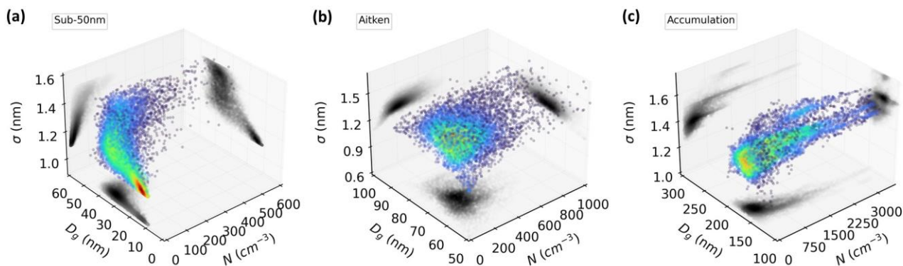
215 Figure 2. Hourly Amazonian PNSDs arrangements in the N - D_g - \sigma phase space. The patterns show the distribution of the (a) sub-50 nm, (b) Aitken, and (c) accumulation modes. Every data point represents one full PNSD. In color is the density of the data points, with respective projections in grey scale shadows on all three axes. The distribution considered spans one year of measurements (May 2021 to April 2022).
