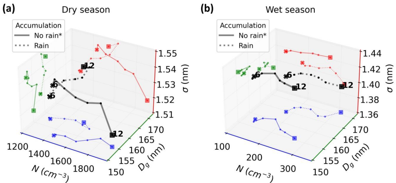
Figure 6. Composites of Amazonian PNSDs in the N - D_g - \sigma phase space for days with and without precipitation. The trajectories are in the morning, going from 6 (cross marker) to 12 (square marker) LST, for cases of afternoons with and without rainfall events.
