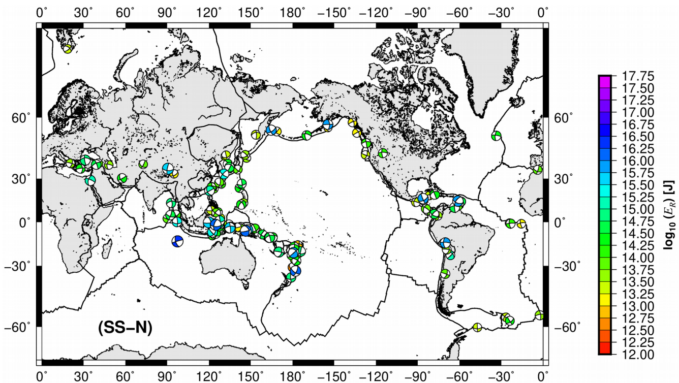
Figure S12. Spatial distribution of radiated seismic energy for SS-N events.
