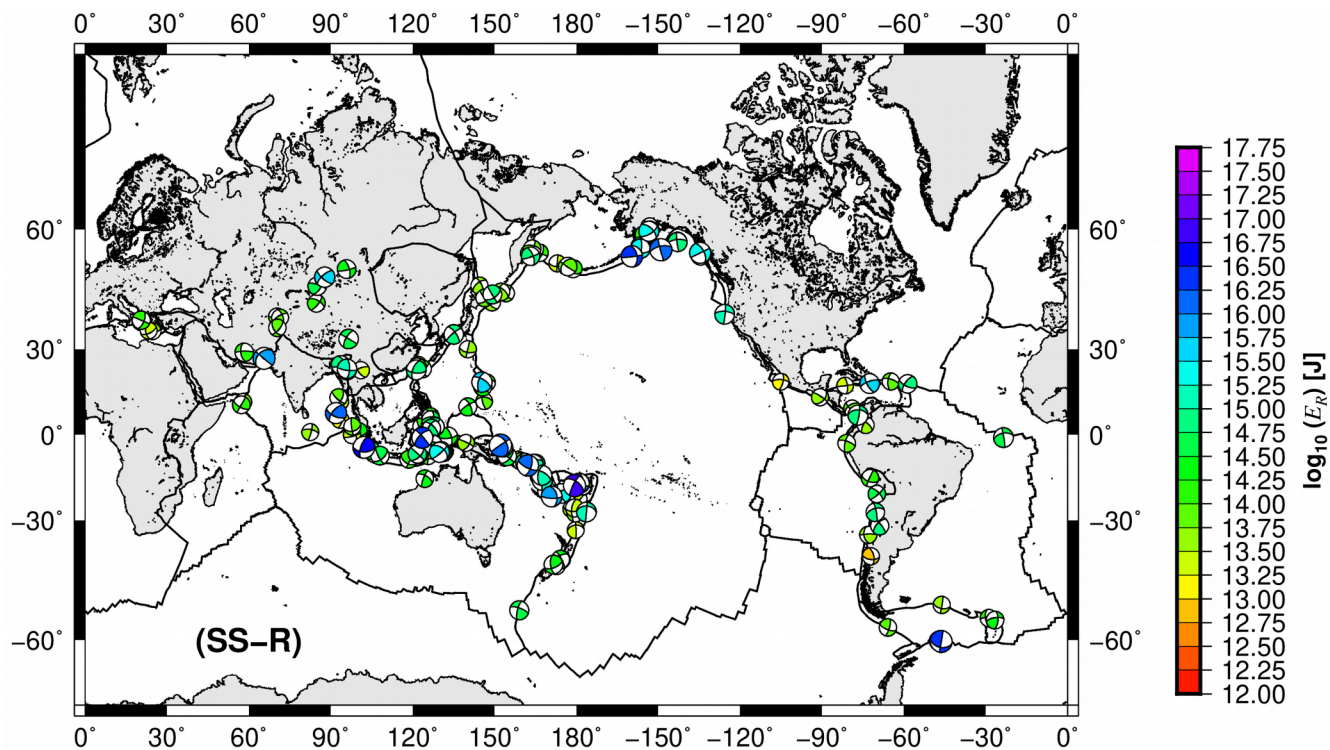
Figure S10. Spatial distribution of radiated seismic energy for SS-R events.
