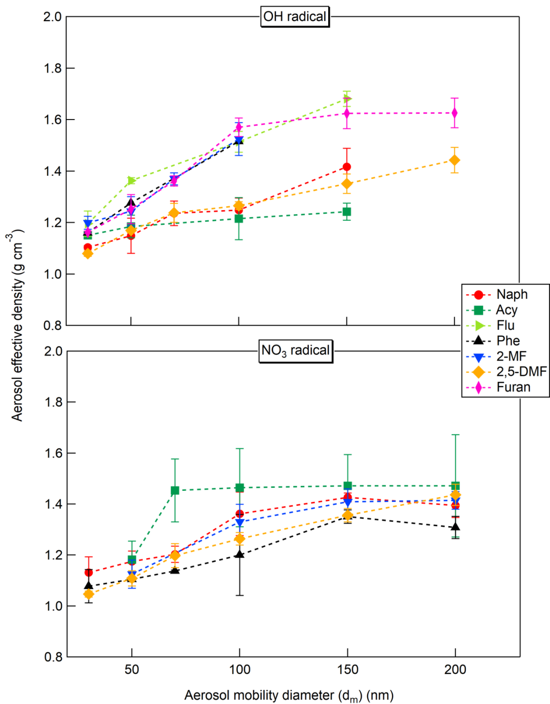
Figure 4. Comparison of the effective density of the PAHs and furans SOA formed under day and nighttime conditions (OH and NO 3 radicals respectively) as a function of the aerosol mobility diameter. The error bars correspond to the standard deviations ( 2\sigma ) on the number of measurements replicates ( n=2 to 4 ). No results are shown for Furan and Flu with NO 3 radicals due to unstable SOA generation or no SOA formed.
