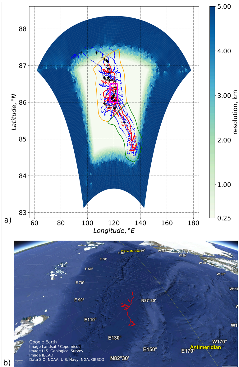
Figure 1. a) - Model domain resolution with the position of the observational data used in this study, covering a period of \approx 2.5 months. The positions of the observational data used for nudging are separated by instrument type: blue - 5 SIT buoys, with CTDs at 10,20,50,75,100 m depth (Hoppmann et al., 2022). red – PS- and OC-CTD casts (Tippenhauer et al., 2023a, b), and ITP profiles (Toole and Krishfield, 2016). Black crosses - position of MSS profiles used for validation Schulz et al. (2022). The green polygon indicates an area with mainly straight drift trajectories, whereas the orange polygon indicates an area with often overlapping buoy trajectories. The magenta rectangle shows the area of Figure 11. b) - The border situation map with the ship's drift trajectory is marked in red. ©Google Earth 2019
