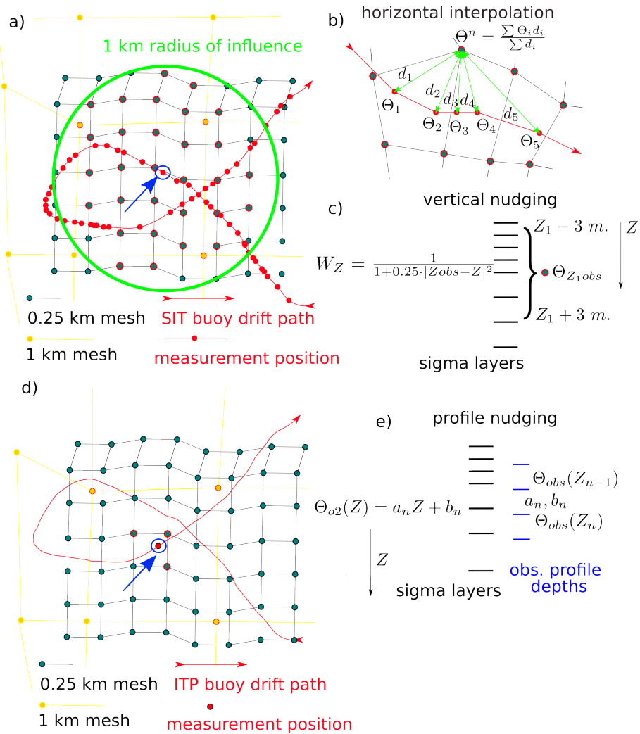
Figure 2. a), b) and d) - Schematic of interpolation and masking on the mesh. Blue and yellow circles are vertices of 0.25 and 1 km resolution meshes. The red lines and circles represent the paths and measurement positions of SIT buoys in a) and of ITP and PS/OC CTDs in d). c) - vertical relaxation weights distribution. e) - vertical interpolation of observed profile. a_n and b_n linear interpolation coefficients. Meshes vertices marked in red are influenced by the measurement marked with a blue circle.
