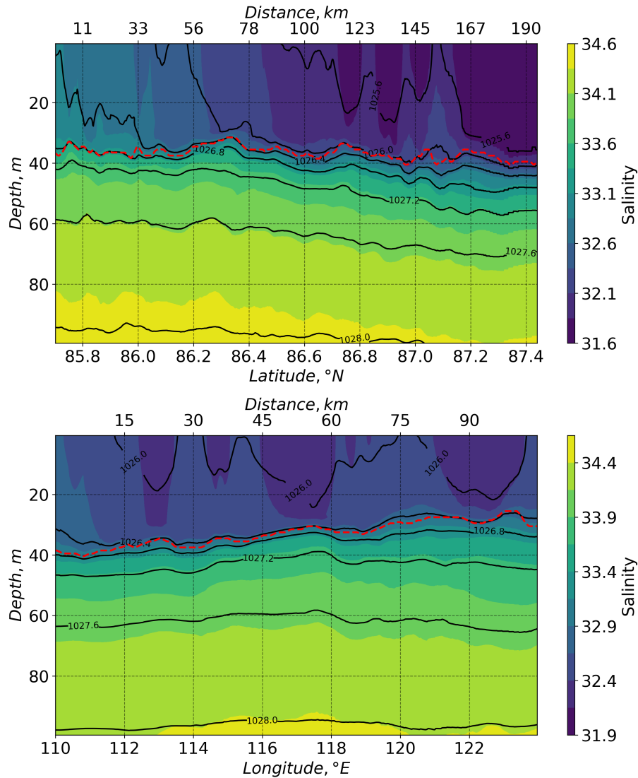
Figure 8. Cross sections along 115 °East Longitude (upper) and 86.2 °North Latitude (lower). Filled colour contours are salinity psu, and black contours are density \text{kg}/\text{m}^3 . Red dashed lines show ML depth. Results of the free run after 2.5 days.
