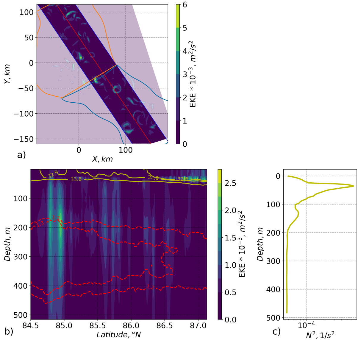
Figure 9. Modeled eddy kinetic energy and N^2 after 5 days of free run. a) - EKE at 47 m depth. The highlighted area indicates an averaging area in the stereographic projection. The area of averaging is chosen so that the line length along the X direction is the same for any Y position. Averaging was done along X direction and covered 80 km with the center indicated by the red line. The red line was chosen to be the longest straight line within the area covered by data. Green and orange polygons indicate the same areas as in Figure 1. b) - vertical distribution of the averaged along X direction EKE. Red dashed lines are isotherms for 1.2 and 1.3 ^{\circ}\text{C} . Yellow solid lines are isohalines for 33.6 and 32.9 psu. c) panel shows mean stratification computed over the area shown in panel a).
