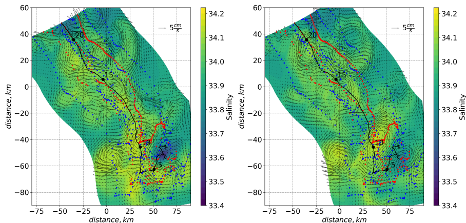
Figure 8. Salinity at 47 meters-m depth in the free run after 5 (left) and 19 (right) days model time, with velocity vectors (arrow top right indicate 5 cm/s) zoomed to the area with mainly straight drift (indicated by a green contour in Figure 1). The black line indicates the drift track of Polarstern . The black dots are the daily positions of the ship.
