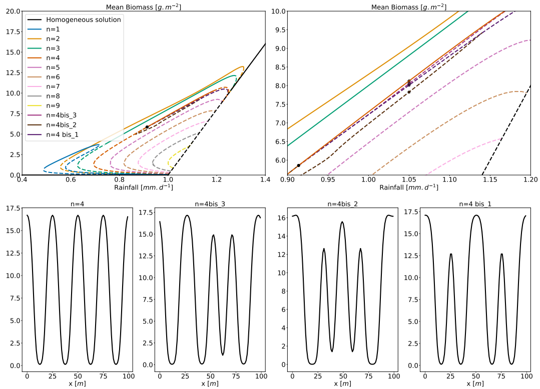
Figure 6. On the left-hand-side upper panel, bifurcation diagram with the addition of n -mixed state branches. The mixed state branches originating the zero modes along the n = 4 branch are called n = 4bis_1 , n = 4bis_2 and n = 4bis_3 . The bifurcation point is marked with a black dot. On the right-hand-side upper panel, an enhancement of the area around the bifurcation point. On the lower panels, solutions for two values the biomass profile of rainfall of the n = 4 and the n = 4bis -branch mixed states for a particular value of rainfall. The position on those solutions equilibria on the bifurcation diagram are marked by pentagone circle on the right-hand-side upper panel
