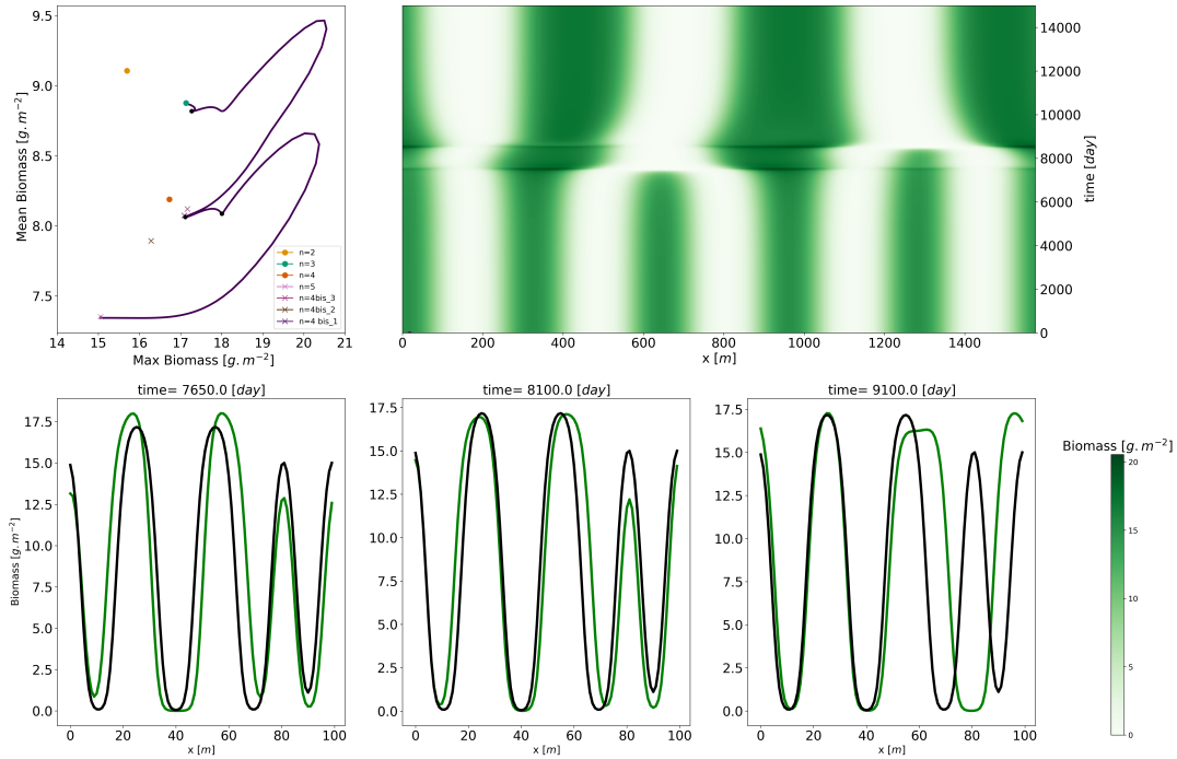
Figure 8. On the left upper panel, trajectories on a pseudo-summary phase space from an initial condition close to the n = 5 equilibrium with a fixed rainfall R = 1,05 \text{ mm/year} R = 1.05 \text{ mm d}^{-1} . The relevant equilibria are shown, if the equilibrium is stable (unstable) the marker associated is a circle (cross). On the right panel, we show the time evolution of the biomass. On the three lower panels, the dynamical solution at three different times are shown: the mixed state is represented (in green) and also the shape (in black) of the mixed state denoted by n = 4bis_3 .
