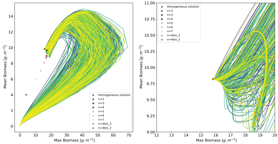
Figure A4. Trajectories on a summary phase space from random initial condition with a fixed rainfall R = 1.1 \text{ mmd}^{-1} . The relevant equilibria are shown, if the equilibrium is stable (unstable) the marker associated is a circle (cross).
