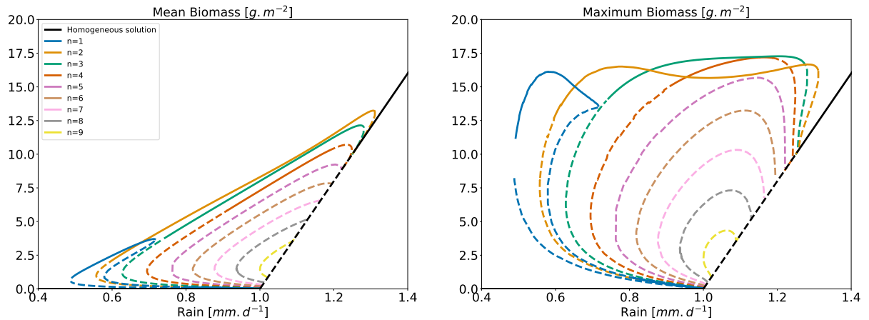
Figure 4. Bifurcation diagram for the Rietkerk's model with L=100mL=100m . Each branch is labelled-labeled by an integer corresponding to the order of the wavenumber associated with the zero mode. Solid lines correspond to stable states and dashed lines to unstable states.
