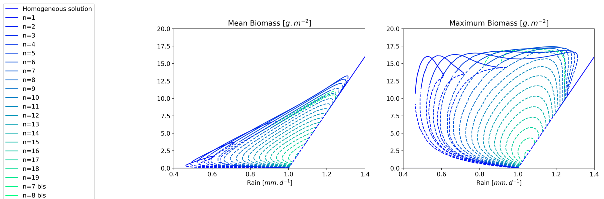
Figure 9. Bifurcation diagram for the Rietkerk's model with L = 200 \text{ m} L = 200 \text{ m} . Each branch is labelled by an integer corresponding to the order of the wavenumber associated with the zero mode. Plain lines correspond to stable states and dashed lines to unstable states.
