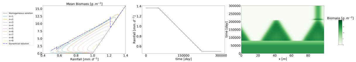
Figure 7. Trajectories on Trajectory of the Rietkerk model under a summary phase space from random initial condition with a fixed decreasing rainfall R = 1,13 \text{ mm/year} scenario. The relevant equilibria are shown on the left panel, if the equilibrium is stable (unstable) trajectory in the marker associated is a circle (cross) bifurcation diagram plotted in blue dashed-dot line. On the middle panel, the rainfall with respect to time and on the right panel, the time evolution of the biomass.
