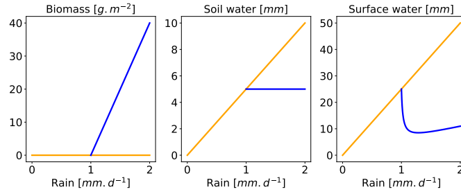
Figure 1. Homogeneous solutions-equilibria of Rietkerk's model. From left to right are represented the biomass, the soil water and the surface water. Blue line is solutions-the equilibrium with vegetation, yellow is without.
