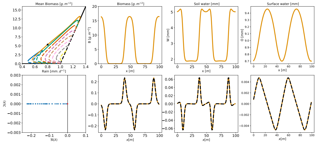
Figure 5. On the upper panels, equilibrium solution for a given value of R (rainfall) ( 0.9\text{mm.day}^{-1} – 0.9\text{mmd}^{-1} ) on the n = 2 branch. The black pentagon-dot on the left-hand-side panel shows the position of the solution-equilibrium . The three other panels show, from left to right, B ( biomassbiomass ) [ g.m^{-2} – gm^{-2} ], W (soil water) [ mmmm ] and O (surface water) [ mmmm ]. On the left-hand-side lower panel, eigenvalues of the Jacobian matrix associated with the solution-equilibrium . The real part is on x axis and the imaginary part on the y axis . The larger eigenvalue is represented wit ha-with a red dot . The black vertical line marks the 0 position . The black vertical line marks the 0 position . The three other lower panels show, from left to right, the eigenvector associated with the larger eigenvalue projected on B ( biomassbiomass ), W (soil water) and O (surface water) and with a dashed black line, the first spatial derivative of the solution-equilibrium rescaled.
