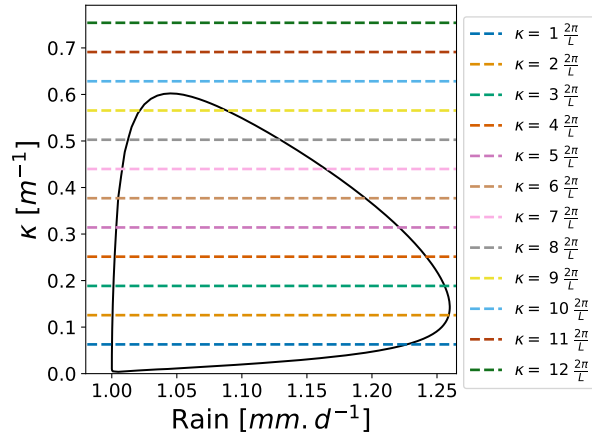
Figure 3. Zero modes present in a domain of L=100L=100m . Horizontal lines correspond to harmonics that fit inside the periodic L = 100 domain. The intersection of the horizontal lines with the \Omega_1 = 0 contour, provides the values of rain R at which new branches of solutions equilibria might appear. Notice that each of the 9 horizontal lines that intersect the contour, intersect it twice, hence 18 zero modes.
