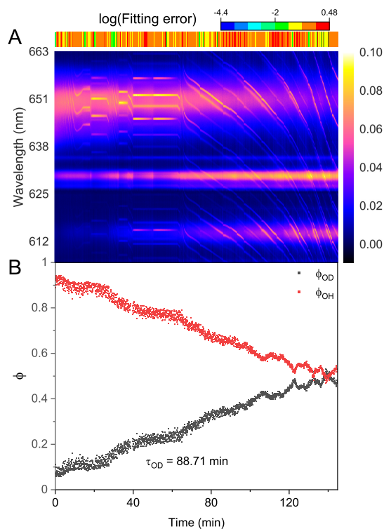
Figure 7. Water diffusion in single phase-separated H_2O +AS+HEX aerosol at RH = 60\% . (A) The time-resolved cavity-enhanced Raman spectra of the droplet. The top color bars indicates the \log(\text{fitting errors}) of the WGMs based on the homogenous Mie scattering model. (B) The temporal variations of fractional concentration of water molecules within the droplet. The droplet was first trapped and equilibrated in H_2O vapor. t = 0 means the onset of switch H_2O moisture vapor to D_2O vapor. The experiment was conducted at room temperature.
