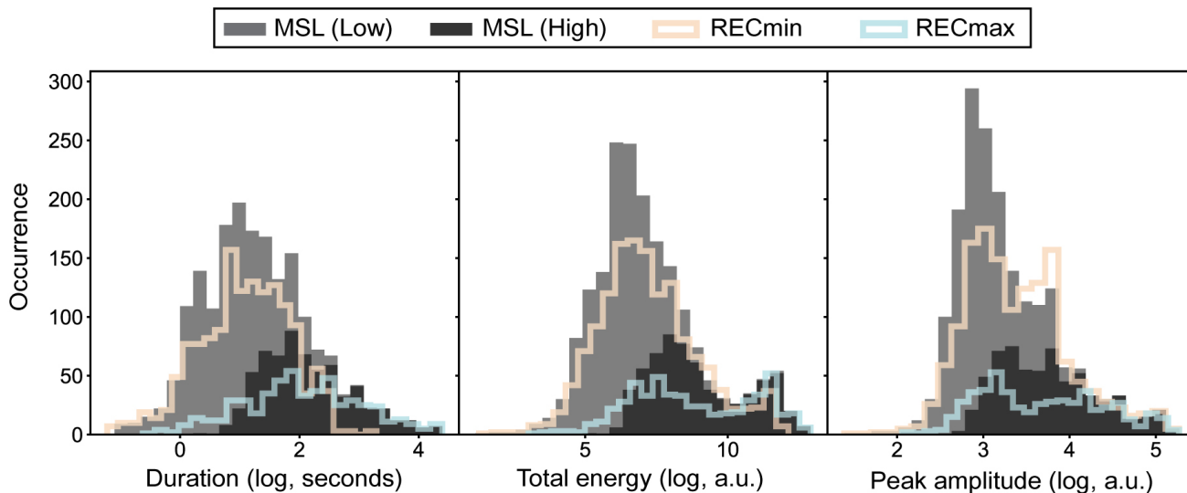
Figure 6. Reference event catalogue feature distributions. Shown on the x-axes are duration ( \log_{10} seconds), total energy ( \log_{10} a.u.), and peak amplitude ( \log_{10} a.u.), while the y-axis shows the occurrences of events with the respective feature value. Detections from the three algorithms are: MSL, i.e. multi-STA/LTA (low confidence, light grey filled, stacked; high confidence, dark grey filled), the recursive RECmin (light orange outline), and the recursive RECmax (light blue outline). The multi-STA/LTA algorithm combines advantages of the other algorithms, as it is able to match, and improve upon, the detections achieved by RECmin, while capturing the full length of extended events in common with RECmax (see also Fig. 5, parameter values given in caption). False detections are less of a concern using the current workflow than in conventional catalogue generation as events are appraised using the Part B unsupervised learning with both events and event-like noise potentially providing insight into glacier processes. See also the discussion of low confidence events following patterns of high confidence events in main text.
