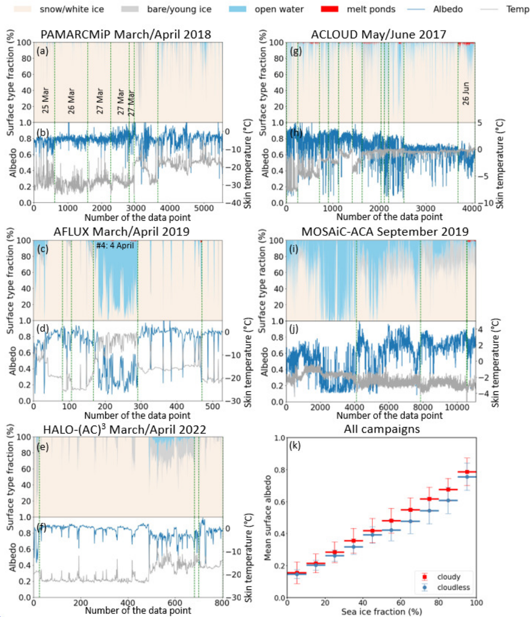
Figure 3. (a) - (j) Temporal development of changes in surface types, surface albedo (blue lines; left y-axis) and surface skin temperature (grey lines; right y-axis) for all five flight campaigns. The proportions of surface types are presented as a stacked area plot to identify the predominant subtypes. Vertical green lines separate the individual flight days. Dates given in the panels are explicitly mentioned in the text. (k) Averaged surface albedo as a function of sea ice fraction (bin size of 10 %), separately for cloudless and cloudy conditions. The standard deviation of the averages is represented by thin vertical bars.
