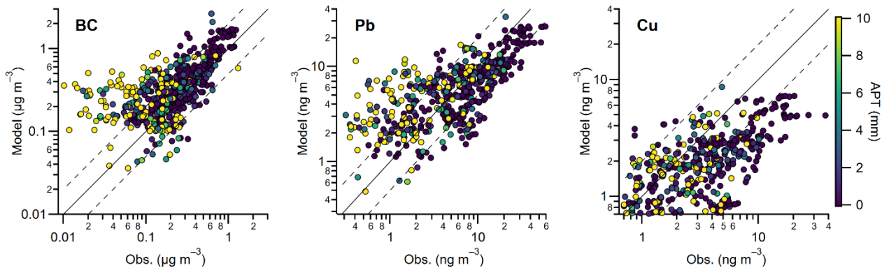
Figure S5. Correlations between the modeled and observed concentrations of black carbon (BC) (left), Pb (middle), and Cu (right) are colored by the values of the accumulated precipitation along trajectories. The solid line indicates the 1:1 line, and the two dashed lines indicate the boundaries of the factor of 2.
