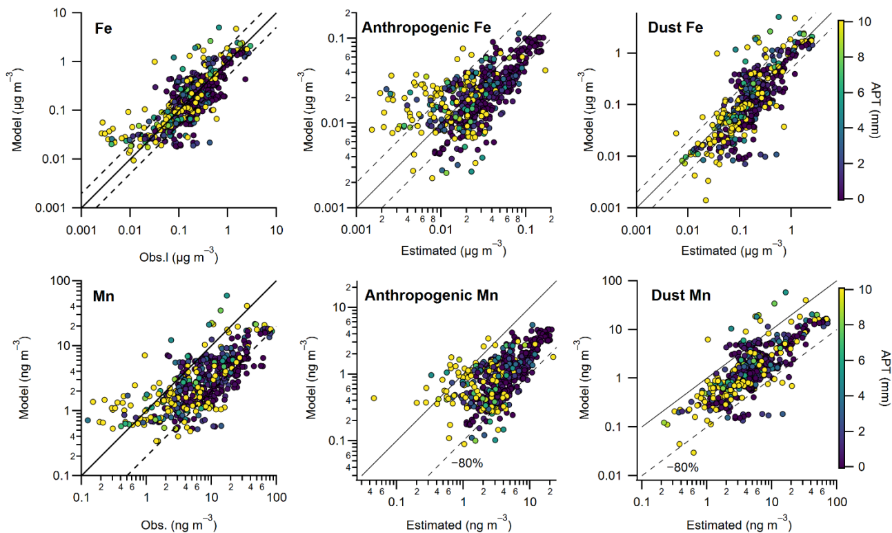
Figure S10. (Top) Correlations of the modeled and observed/estimated concentrations of (left) total-Fe, (middle) anthropogenic-Fe, and (right) dust-Fe. (bottom) Correlations of the modeled and observed/estimated concentrations of (left) total-Mn, (middle) anthropogenic-Mn, and (right) dust-Mn. All the data points are colored by the values of the accumulated precipitation along trajectories (APT). The black line depicts the 1:1 line. The dashed two lines in the top panel depict the boundaries of the factor 2. The dashed line in the bottom panel depicts the -80% of the model-to-estimation ratios.
