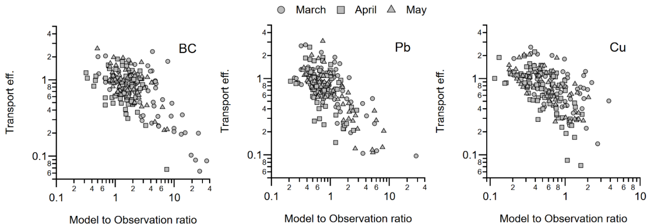
Figure S6. Relationship between transport efficiency and model-to-observation ratios for black carbon (BC) (left), Pb (middle), and Cu (right). Shaded markers for 4-hourly data points are differentiated by the month (circles (March); squares (April); triangles (May)) of 2018.
