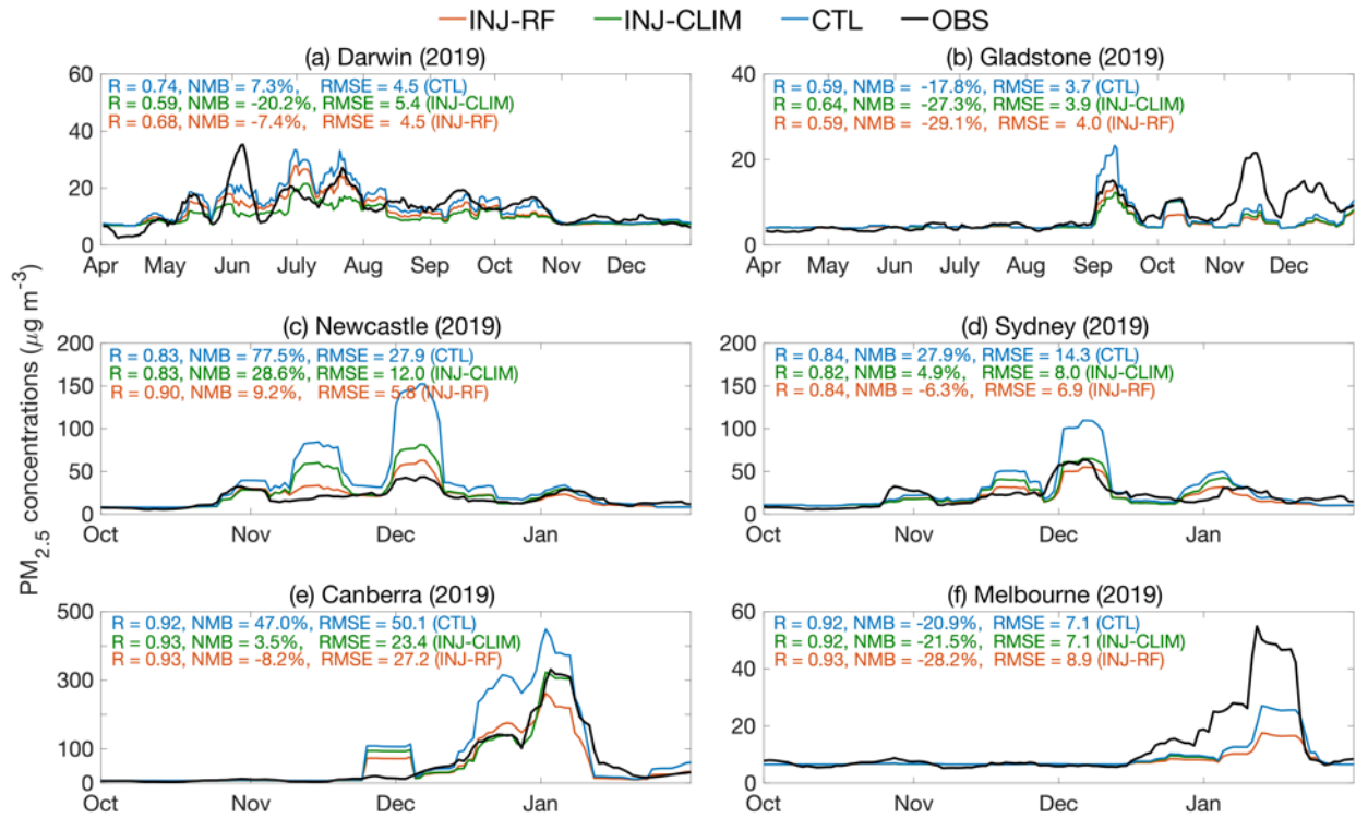
1040 Figure 7. Time series of 10-day moving average of observed and simulated total PM 2.5 concentrations from the CTL (blue), INJ-CLIM (green), and INJ-RF (red) experiments during the fire seasons of 2019-2020 at six sample receptors: (a) Darwin (Palmerston), (b) Gladstone (South Gladstone), (c) Newcastle (Wallsend), (d) Sydney (Liverpool), (e) Canberra (Florey), and (f) Melbourne (Footscray). Shown inset are the temporal correlation coefficients R , NMBs, and RMSEs of daily total PM 2.5 concentrations compared to the surface measurements.
