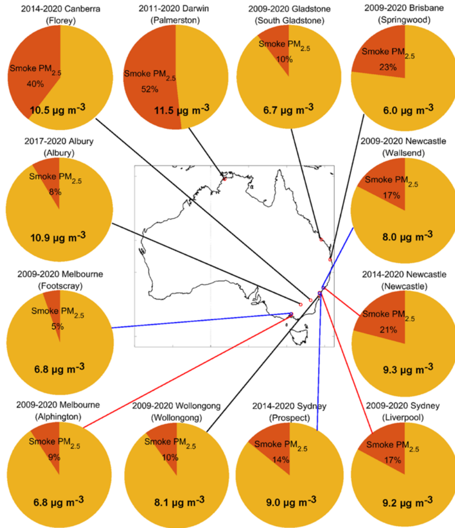
1030 Figure 6. Contributions of simulated smoke PM 2.5 concentrations from the INJ-RF experiment to the observed total PM 2.5 concentrations (numbers on the pie charts) at 12 receptors averaged over the fire seasons of their respective observation periods (Table 3). Names of the observation sites are given in parentheses. Red sectors represent smoke contributions, while dark yellow sectors signify the differences between observed total PM 2.5 and simulated smoke PM 2.5 concentrations – i.e., the non-fire PM 2.5 . Small 1035 circles on map represent the locations of these receptors. Different colors (red, blue, and black) are used to distinguish adjacent receptors.
