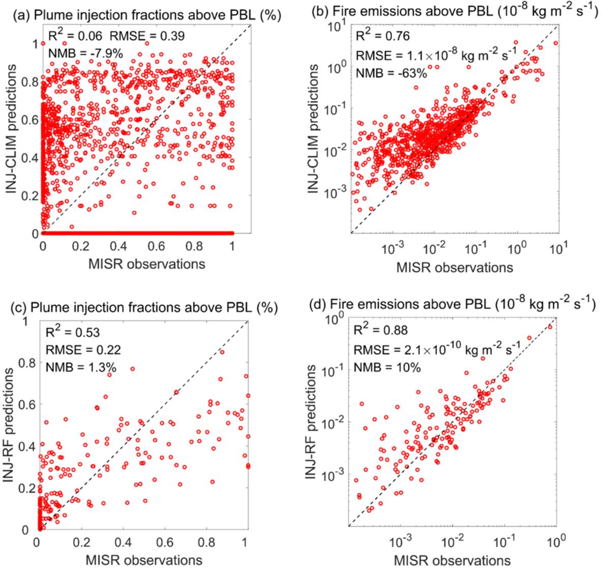
1005 Figure 2. Scatter plots of plume injection fractions above the PBL calculated by (a) climatological method and by (c) random forest, compared to the MISR derived plume injection fractions. Scatter plots of mass fluxes of fire emissions injected above the PBL estimated by injection fractions from (b) climatological method and (d) random forest, compared to MISR observations, in units of \text{kg m}^{-2} \text{ s}^{-1} . Also shown are the R^2 values and the RMSEs and NMBs between the predictions and MISR observations.
