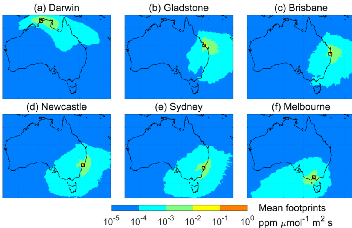
1055 Figure 9. Mean of sensitivity footprints simulated by STILT in unit of \text{ppm } \mu\text{mol}^{-1} \text{ m}^2 \text{ s} during the fire seasons (April to December for Darwin and Gladstone; August to the following January for other cities) in (a) Darwin (Palmerston), (b) Gladstone (South Gladstone), (c) Brisbane (Springwood), (d) Newcastle (Wallsend), (e) Sydney (Liverpool) and (f) Melbourne (Alphington) from 2009 to 2020. The names in parentheses are site names. The black squares represent the locations of receptors.
