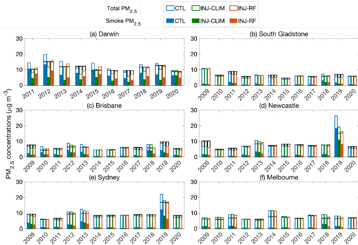
1005 Figure 8. Mean simulated concentrations of smoke PM_{2.5} and background PM_{2.5} from the three sensitivity experiments (blue: CTL, green: INJ-CLIM, red: INJ-RF), as well as observed total PM_{2.5} concentrations (black: OBS) in (a) Darwin (Palmerston), (b) Gladstone (South Gladstone), (c) Brisbane (Springwood), (d) Newcastle (Wallsend), (e) Sydney (Liverpool), and (f) Melbourne (Alphington). The different receptors have different observation periods. The modeled total PM_{2.5} concentrations are designated by the height of 1010 the colored bars, consisting of smoke PM_{2.5} (color-filled bars) and the background PM_{2.5} (empty bars) in units of \mu\text{g m}^{-3} .
