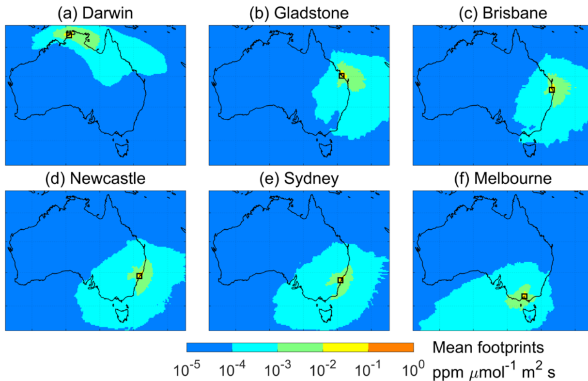
1015 Figure 9. Mean of sensitivity footprints simulated by STILT in unit of ppm \mu\text{mol}^{-1} m 2 s during the fire seasons (April to December for Darwin and Gladstone; August to the following January for other cities) in (a) Darwin (Palmerston), (b) Gladstone (South Gladstone), (c) Brisbane (Springwood), (d) Newcastle (Wallsend), (e) Sydney (Liverpool) and (f) Melbourne (Alphington) from 2009 to 2020. The names in parentheses are site names. The black squares represent the locations of receptors.
