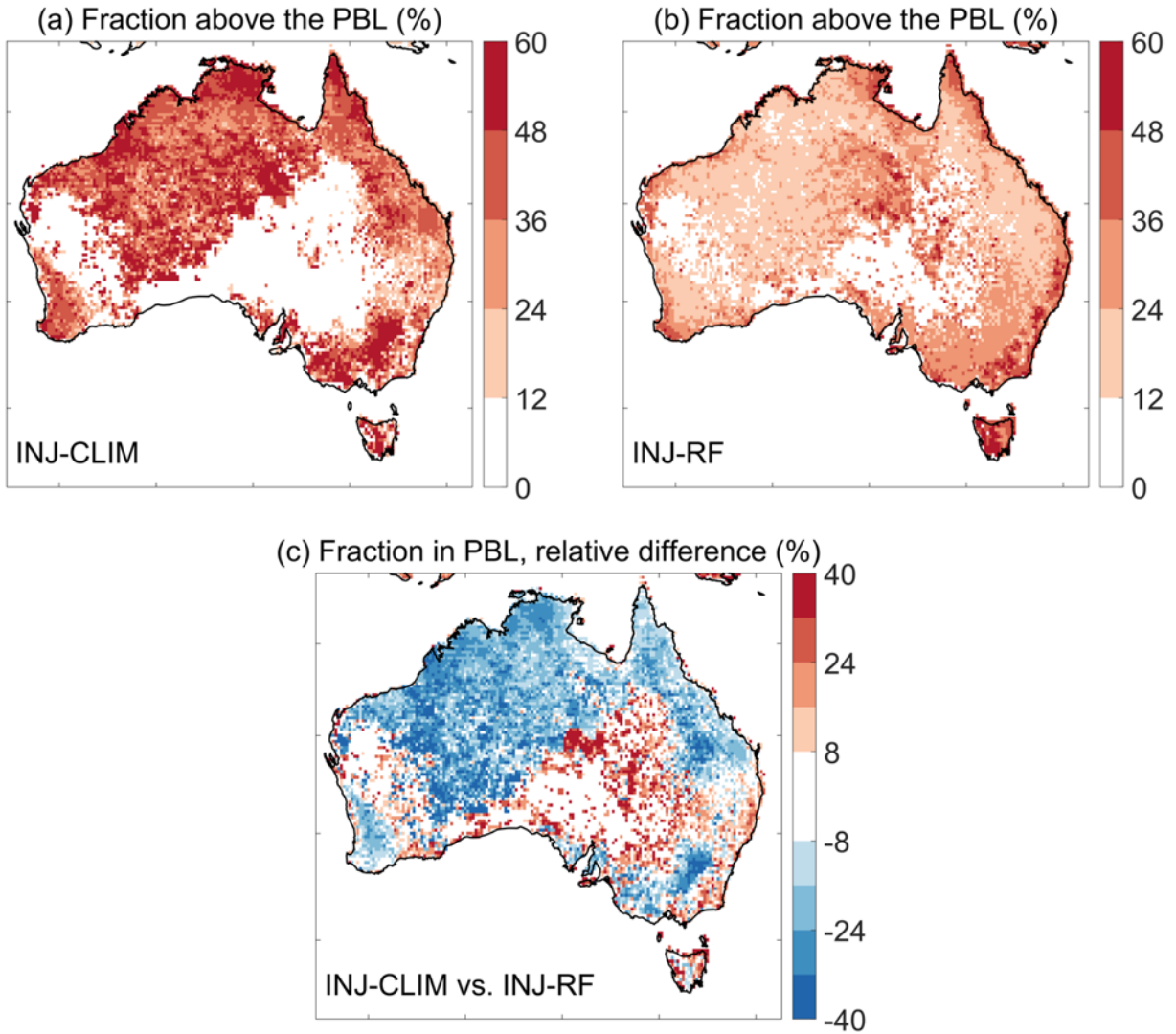
975 Figure 4. Spatial distributions of mean fractions of total OC fire emissions injected above the PBL (in units of %) estimated by (a) climatological method (INJ-CLIM) and (b) random forest method (INJ-RF), as well as (c) the percent differences in OC fire emissions within the PBL between the two methods relative to total OC fire emissions during April to the following January from 2009 to 2020.
