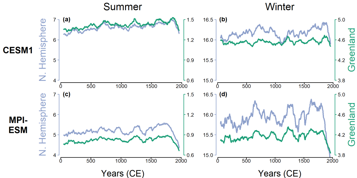
420 Figure 5. Sea-ice area (in million \text{km}^2 ; 100-year running mean) in both models, around Greenland (green) and in the whole Northern Hemisphere (blue), for boreal summer and winter seasons, over the Common Era. The very high agreement indicates that sea-ice proxy-compilations around Greenland are representative for the total northern hemispheric sea-ice area on longer time scales. Disregarding magnitude bias, temporal changes in the sea-ice area simulated around Greenland follow the changes as simulated for the whole Arctic Ocean, especially during summer.
