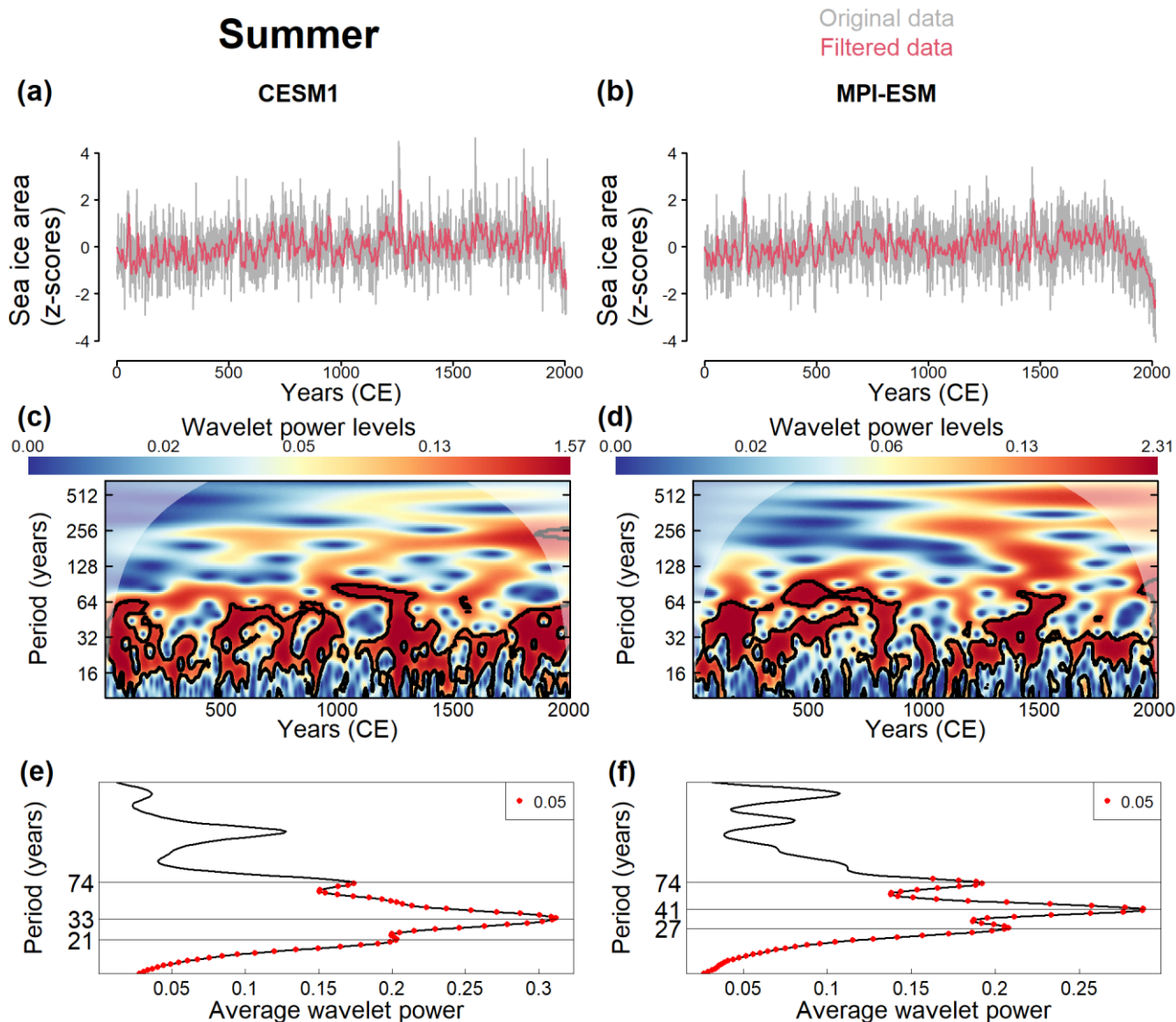
480 Figure 7. Wavelet analysis from both numerical models (CESM1 and MPI-ESM), considering summer sea-ice area. (a,b) 485 Normalized time series of sea-ice area considering the original data (in grey) and the filtered data (in red). (c,d) Wavelet power spectrum and (e,f) global wavelet of the normalized signal on the time-frequency domain. Marked regions on the wavelet spectrum indicate significant power to a 95% confidence interval. The areas under the cone of influence show where edge effects are important. Sea-ice simulations from both models display significant multidecadal quasi-periodic variability but no significant (multi-)centennial variability as found in longer simulations and proxy records for the Holocene (e.g., Askjær et al., 2022).
