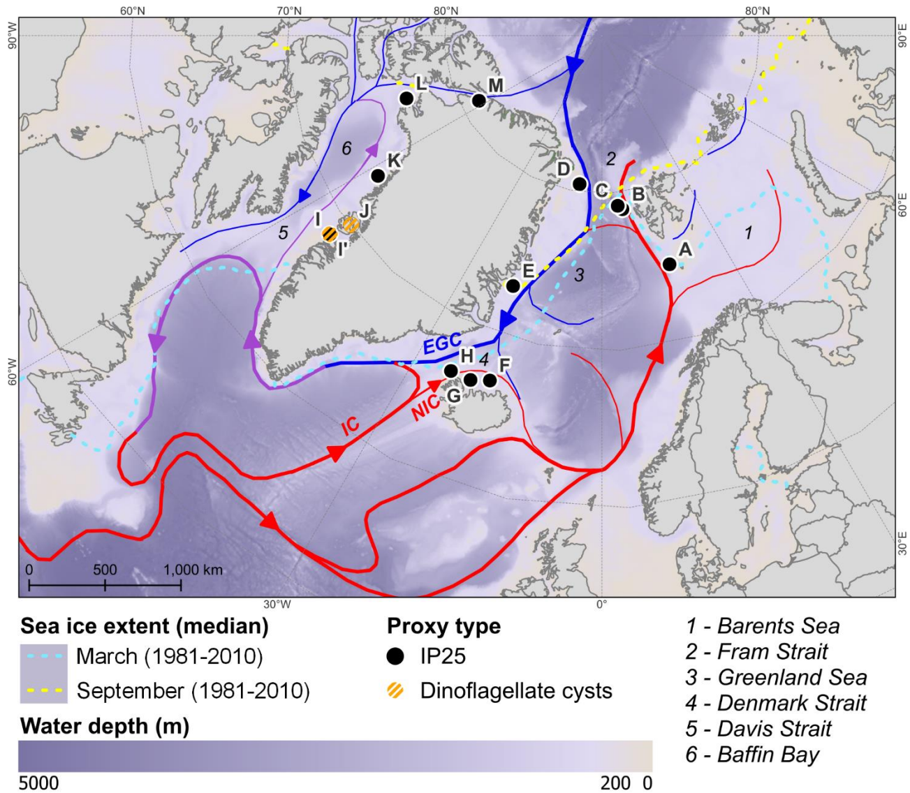
235 Figure 1. Map showing the locations of IP 25 and dinoflagellate cyst records for sea-ice reconstructions. The major surface currents are shown (blue: cold waters; purple: mixed water; red: warm waters), but only the currents discussed in the text are identified. EGC: East Greenland current; IC: Irminger current; NIC: North Irminger Current. The bold black line indicates the area used for the numerical model calculations. The bathymetry was obtained from Amante and Eakins (2009), the currents were plotted based on Talley et al. (2011a) and Talley et al. (2011b), and the median sea-ice extent was obtained from NOAA-NSIDC.
