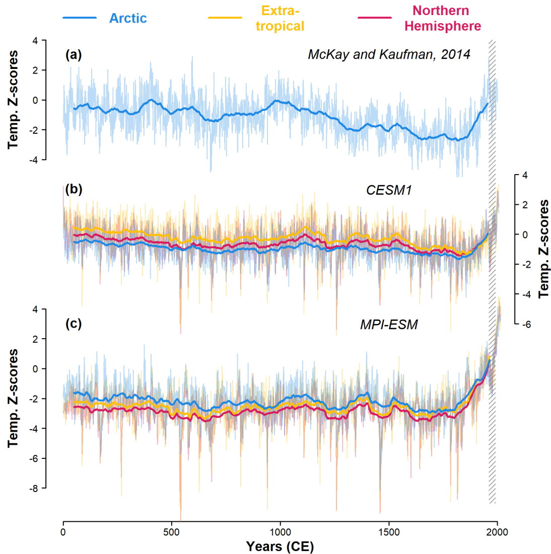
395 Figure 4. Air temperature z-scores (relative to the period between 1961-1990) based on (a) Arctic proxy data (McKay and Kaufman, 2014), (b) CESM1 simulation data and (c) MPI-ESM simulation data. Bold lines refer to 100-years running means. The hatched area indicates the period between 1961-1990. Northern Hemisphere refers to latitudes between 0 – 90° N, the Arctic region refers to latitudes between 60 – 90° N, and the Extra-tropical region refers to latitudes between 30 – 60° N. Temperature simulations from both models and for all three regions display a very similar long-term evolution, showing cooling temperatures for most of the Common Era, followed by a warming trend after 1850. This is consistent with the leading cluster G1 for the sea-ice proxies in Figure 3c. 400
