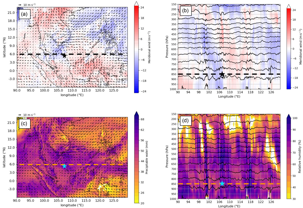
Figure 8. Borneo vortex at maximum intensity (mature stage). As in Fig. 7, but valid at 12 UTC on 23 October 2018 (T+48).
