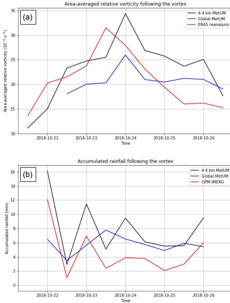
Figure 6. (a) Area-averaged relative vorticity in a 3^\circ box following and centred on the vortex from the 4.4 km MetUM simulation (black line), the N768 MetUM simulation (blue line) and the ERA5 reanalysis product (red line). Area-averaged relative vorticity is calculated at 850 hPa in the 4.4 km MetUM simulation and ERA5 reanalysis, and at the nearest model level at 1.4 km altitude for the N768 simulation due to the unavailability of appropriate pressure level data. (b) 12-h accumulated precipitation in a 3^\circ box following and centred on the vortex, from the 4.4 km MetUM simulation (black line), the N768 MetUM simulation (blue line) and the GPM-IMERG satellite product (red line).
