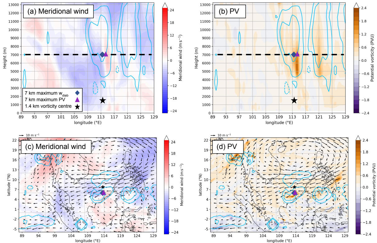
Figure 13. (a) Longitude-height cross-sections of meridional wind (shaded; \text{m s}^{-1} ), and (b) Ertel potential vorticity (shaded; PVU) along 6^\circ \text{N} , from the global MetUM simulation initialised at 12 UTC on 21 October 2018, valid at 00 UTC on 22 October 2018 (T+12). (c) Meridional wind (shaded; \text{m s}^{-1} ) and (d) potential vorticity (shaded; PVU) with horizontal wind vectors overlaid ( \text{m s}^{-1} ; reference vector = 10 \text{ m s}^{-1} ) at 7 km. In all panels, balanced vertical velocity forced by diabatic heating is overlain (blue contours; -2, 2, 6 and 10 \text{ cm s}^{-1} ).
