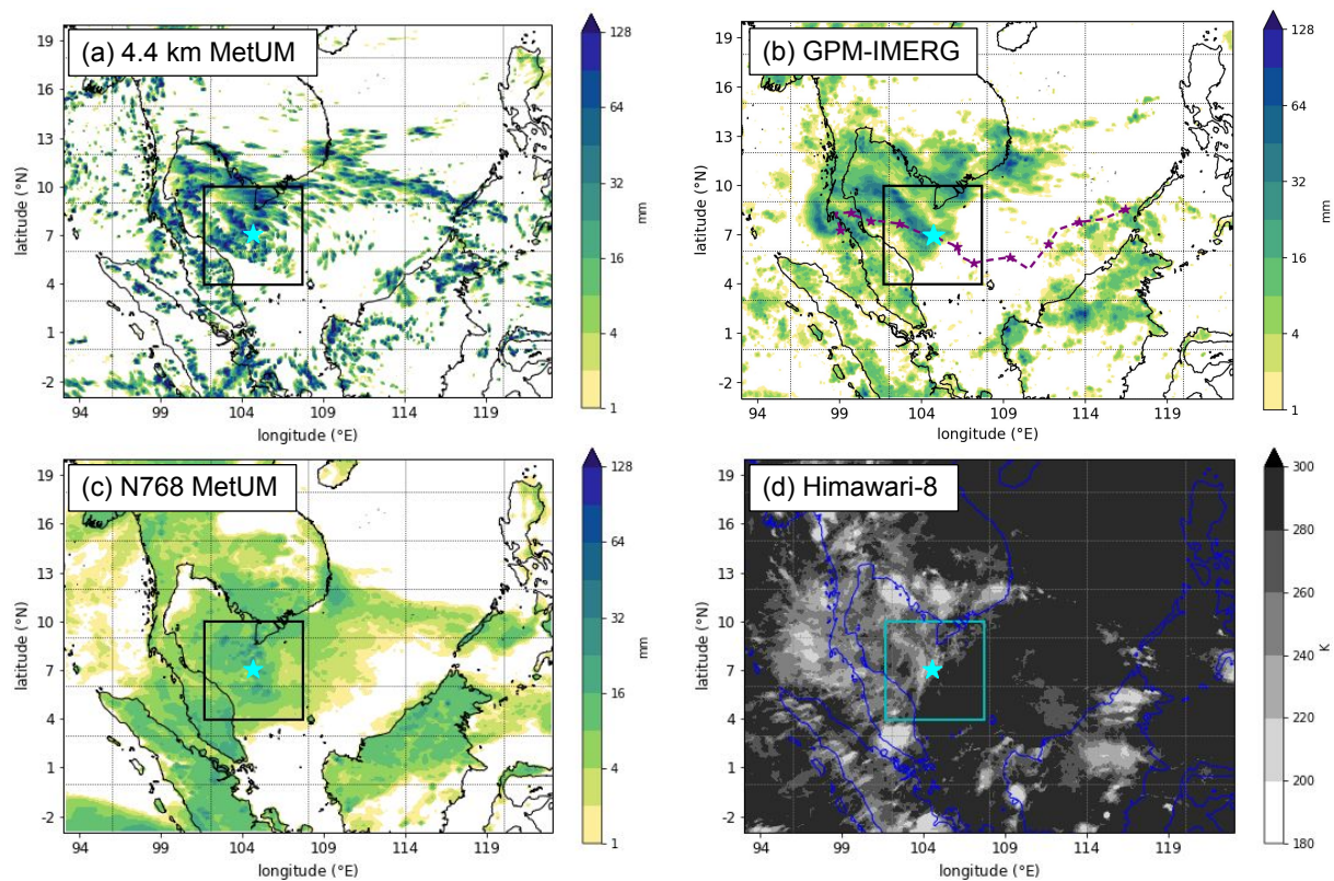
Figure 5. 12-h accumulated precipitation ending at 12 UTC on 24 October 2018 (shaded, mm) from: (a) 4.4 km MetUM simulation initialised at 12 UTC on 21 October 2018, (b) GPM-IMERG satellite product, (c) N768 MetUM simulation initialised at 12 UTC on 21 October 2018. (d) Brightness temperature (shaded, K) from the Himawari-8 satellite, valid at 12 UTC on 24 October 2018. The cyan star marks the position of the Borneo vortex centre. The purple dashed line in (b) represents the vortex track between 12 UTC on 21 October and 12 UTC on 26 October 2018, with the smaller purple stars marking the vortex centre position every 12 h.
