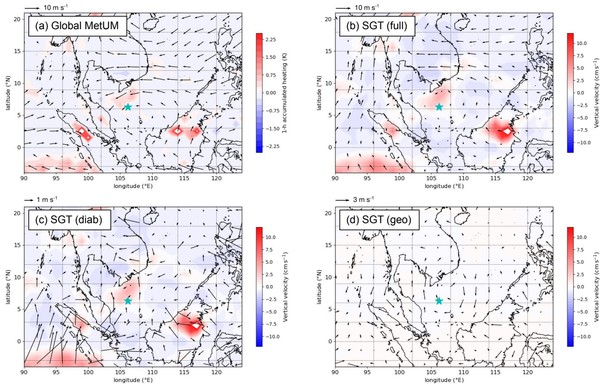
Figure 11. (a) 1-h accumulated heating at 7 km (shaded; K) and horizontal wind at 2 km (vectors; \text{m s}^{-1} ) from N768 MetUM simulation initialised at 12 UTC on 21 October 2018, valid at 12 UTC on 23 October 2018 (T+48). (b to d) Balanced vertical velocity at 7 km (shaded; \text{cm s}^{-1} ) and horizontal wind at 2 km (vectors; \text{m s}^{-1} ) inverted using the SGT tool at 12 UTC on 23 October 2018 with (b) full forcing, (c) diabatic forcing only, and (d) geostrophic forcing only. In (a) and (b), the wind vectors represent the full horizontal wind. In (c) and (d), the wind vectors represent the ageostrophic wind only. Note that the scale of the vectors is different in all panels, with the key in the upper left corner.
