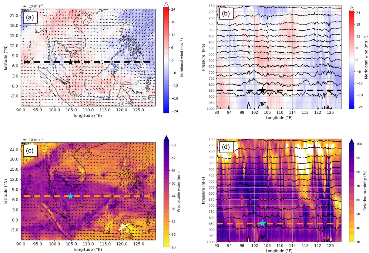
Figure 9. Borneo vortex at start of weakening phase. As in Fig. 7, but valid at 12 UTC on 24 October 2018 (T+72).
