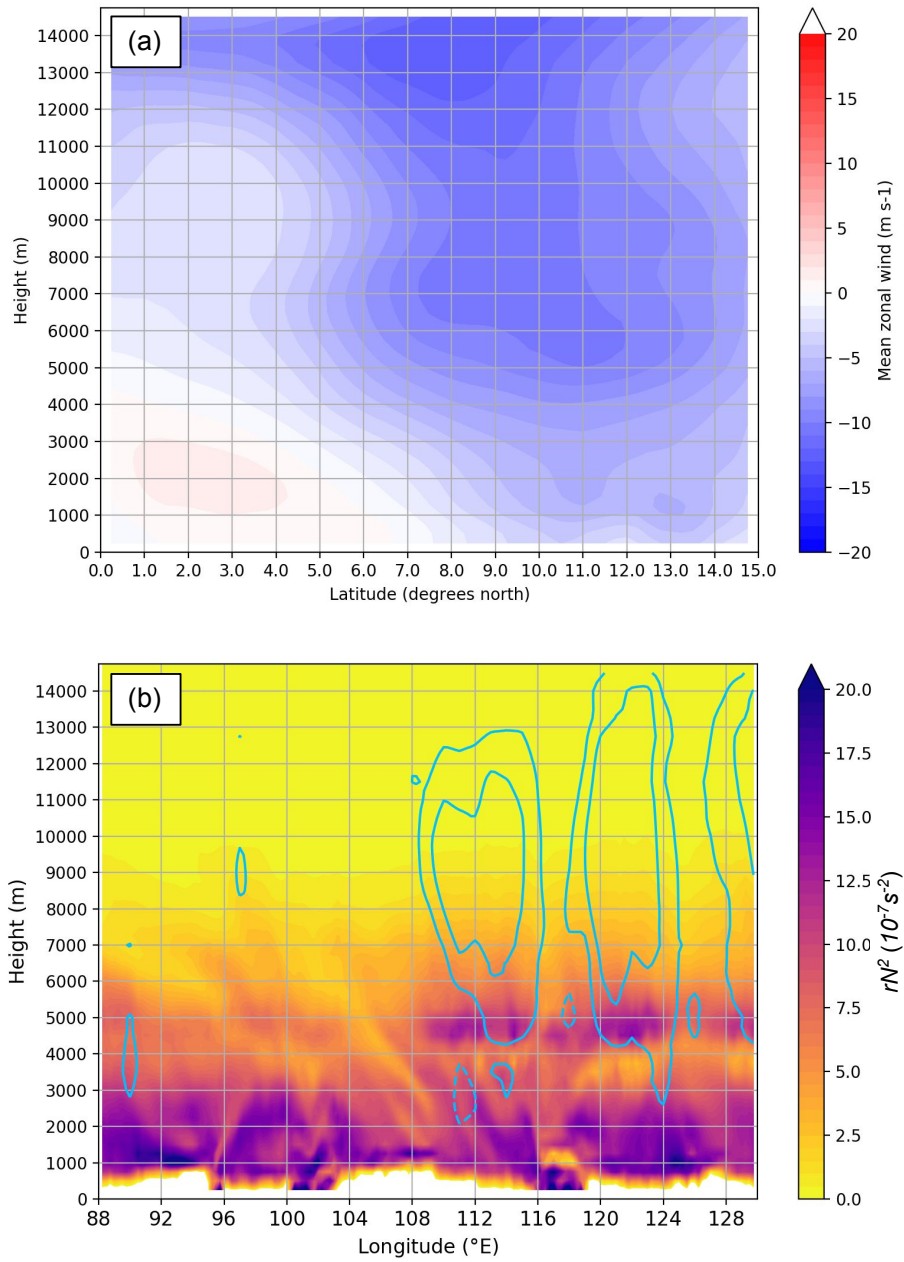
Figure 10. (a) Mean zonal wind from the N768 MetUM simulation initialised at 12 UTC on 21 October 2018, averaged over time (12 UTC on 21 October 2018 to 12 UTC on 26 October 2018) and longitude ( 95^{\circ} E to 120^{\circ} E). (b) The quantity rN^2 (shaded; 10^{-7} \text{ s}^{-2} ), averaged across 5.5\text{-}7^{\circ} N, combines specific humidity and static stability to identify changes between moist, unstable air (large rN^2 ) and drier, more stable air (smaller rN^2 ), valid at 00 UTC on 22 October 2018 (T+12). Blue contours indicate the diabatically-forced component of the balanced vertical velocity from the SGT tool ( -2, 2, 6, 10 \text{ cm s}^{-1} ).
