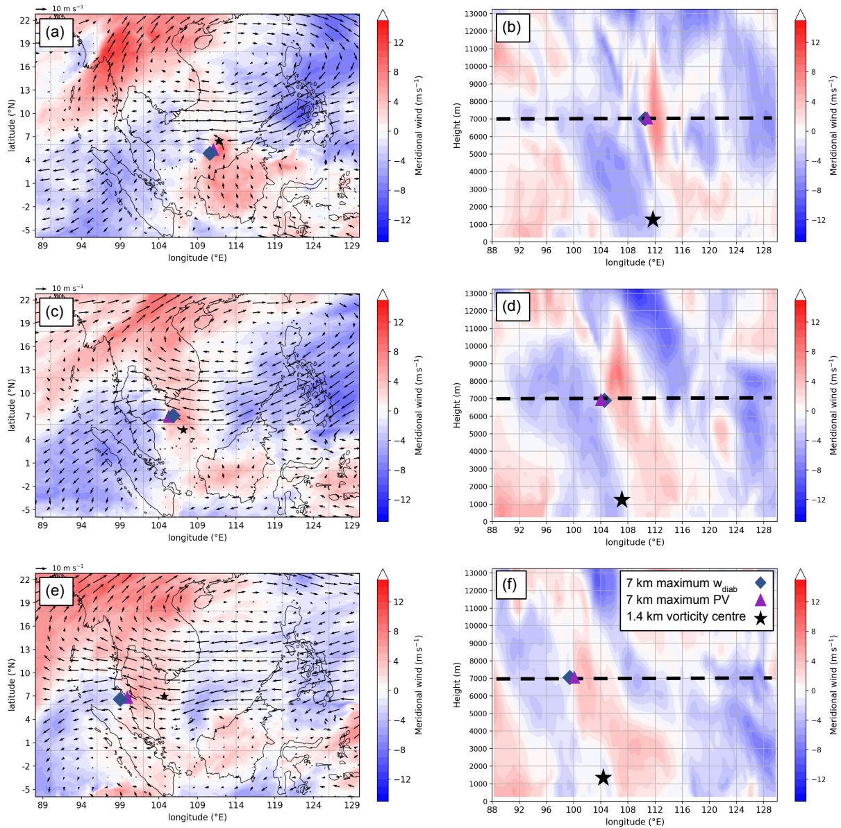
Figure 12. (a) Meridional wind (shaded; \text{m s}^{-1} ) and horizontal wind ( \text{m s}^{-1} ; reference vector = 10 \text{ m s}^{-1} ) at 7 km, from the global MetUM simulation initialised at 12 UTC on 21 October 2018, valid at 12 UTC on 22 October 2018 (T+24); (b) longitude-height cross-section of meridional wind (shaded; \text{m s}^{-1} ) along 6^\circ\text{N} . Overlain are the 850 hPa vorticity centre identified by the tracking algorithm (black star), maximum potential vorticity at 7 km from the MetUM simulation (purple triangle), maximum vertical velocity forced by diabatic heating from the SGT tool at 7 km (blue diamond), and the height of the x-y section in ((a); black dashed line at 7 km). (c) and (d), as in (a) and (b) but valid at 12 UTC on 23 October 2018 (T+48); (e) and (f), as in (a) and (b) but valid at 12 UTC on 24 October 2018 (T+72). For reference, panels (c) and (d) are equivalent to Figs. 1a and b.
