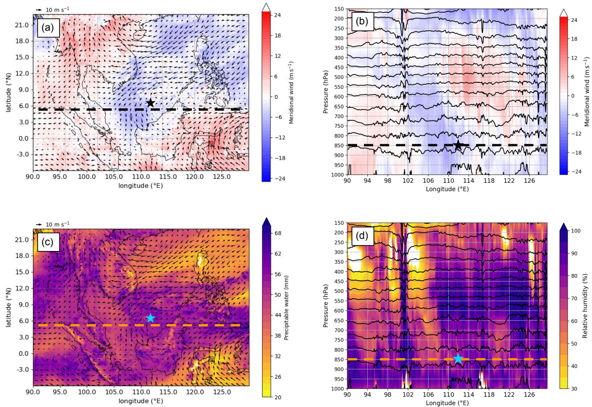
Figure 7. (a) Borneo vortex at intensifying stage. Meridional wind (shaded; \text{m s}^{-1} ) and horizontal wind vectors ( \text{m s}^{-1} ; reference vector = 10 \text{ m s}^{-1} ) at 850 hPa from the 4.4 km MetUM simulation initialised at 12 UTC on 21 October 2018, valid at 12 UTC on 22 October 2018 (T+24); (b) longitude-height cross-section of meridional wind (shaded; \text{m s}^{-1} ) with potential temperature overlaid (black contours; every 2K), from the same 4.4 km MetUM simulation. (c) as in (a), but for total precipitable water (shaded; mm). (d) as in (b), but for relative humidity (shaded; %). Overlaid is the 850 hPa vorticity centre identified by the tracking algorithm (black/blue star).
