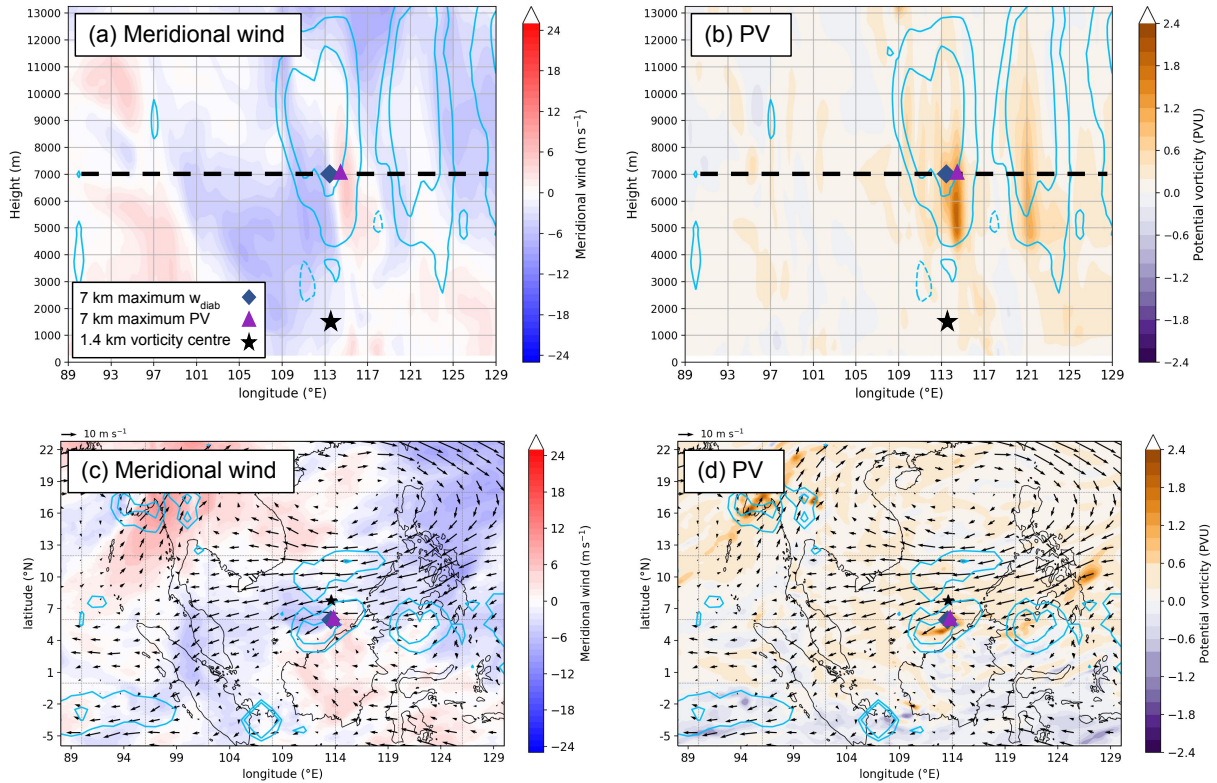
Figure 12. (a) Longitude-height cross-sections of meridional wind (shaded; \text{m s}^{-1} ), and (b) Ertel potential vorticity PV (shaded; PVU) along 6^\circ\text{N} , from the global MetUM simulation initialised at 12 UTC on 21 October 2018, valid at 00 UTC on 22 October 2018 ( T+12 ). (c) Meridional wind (shaded; \text{m s}^{-1} ) and (d) potential vorticity Ertel PV (shaded; PVU) with horizontal wind vectors overlaid ( \text{m s}^{-1} ; reference vector = 10 \text{ m s}^{-1} ) at 7 km. In all panels, balanced vertical velocity forced by diabatic heating is overlain (blue contours; -2, 2, 6 and 10 \text{ cm s}^{-1} ).
