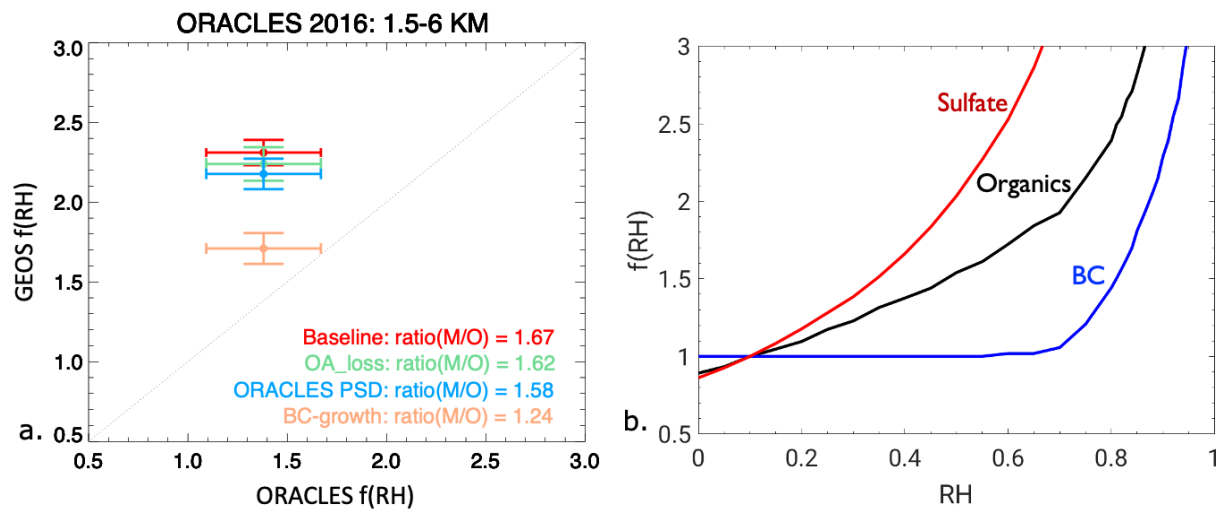
Figure 13. (a) Comparison of simulated to observed f(\text{RH}) in smoke plumes during the ORACLES-I deployment. Different cases of the model optical property assumptions are shown, and the ratio(M/O) reports the ratio of the model to the observed mean values. (b) Default f(\text{RH}) in the GEOS lookup tables for sulfate, OA, and BC.
