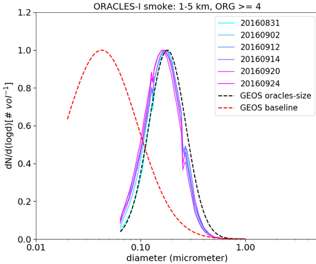
1115 Figure 12. Comparison of GEOS baseline and adjusted particle size distribution for organic aerosol to ORACLES observations from the UHSAS instrument.
