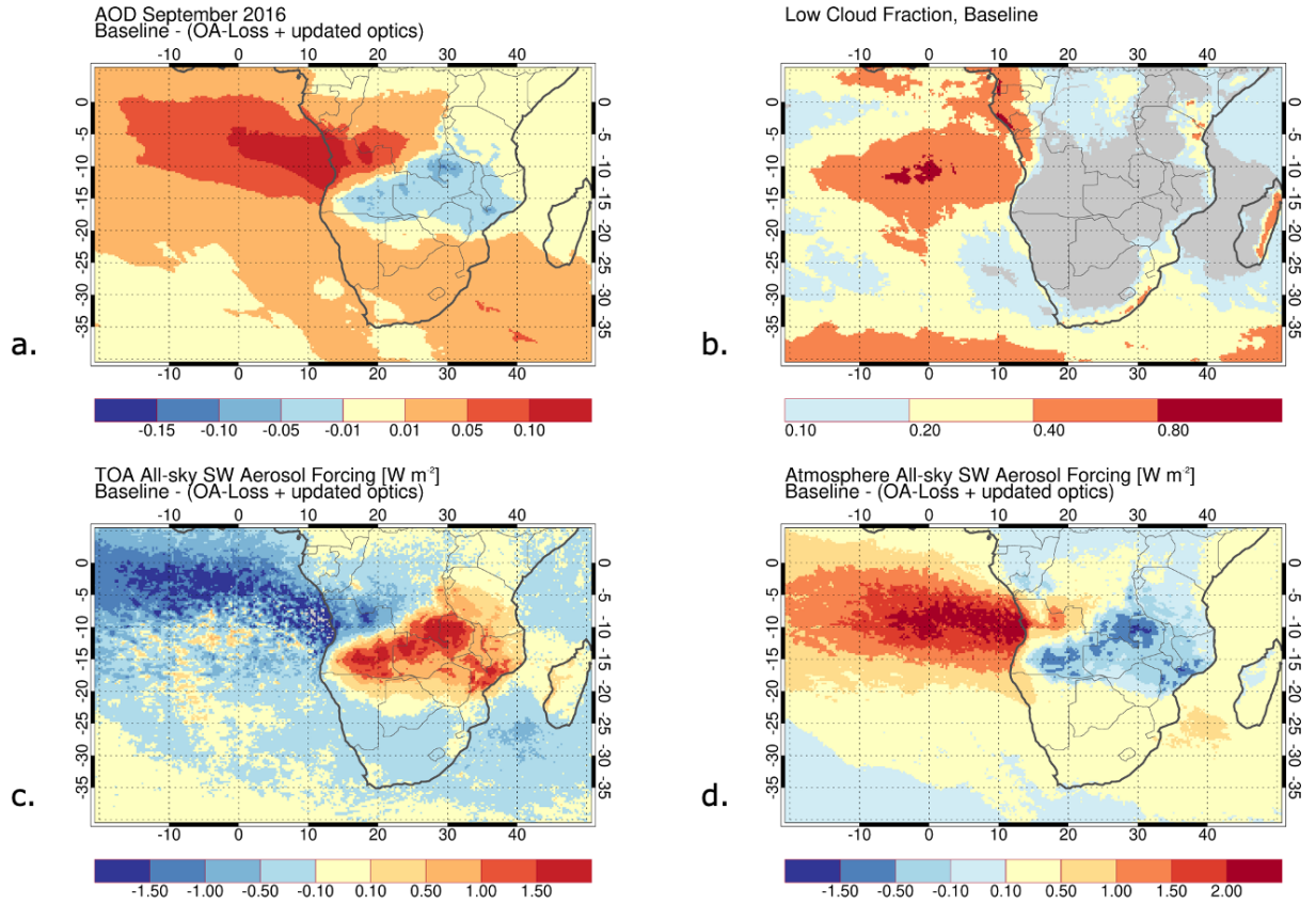
Figure 18. The September 2016 average GEOS-simulated (a) total 550 nm AOD difference between the baseline and OA-loss+updated optics model runs, (b) the low cloud fraction of the baseline run, (c) top-of-atmosphere all-sky shortwave aerosol forcing difference of the baseline and updated runs, and (d) the all-sky shortwave aerosol atmospheric heating difference of the baseline and updated runs. The grey area in (b) is cloud fraction less than 10%.
