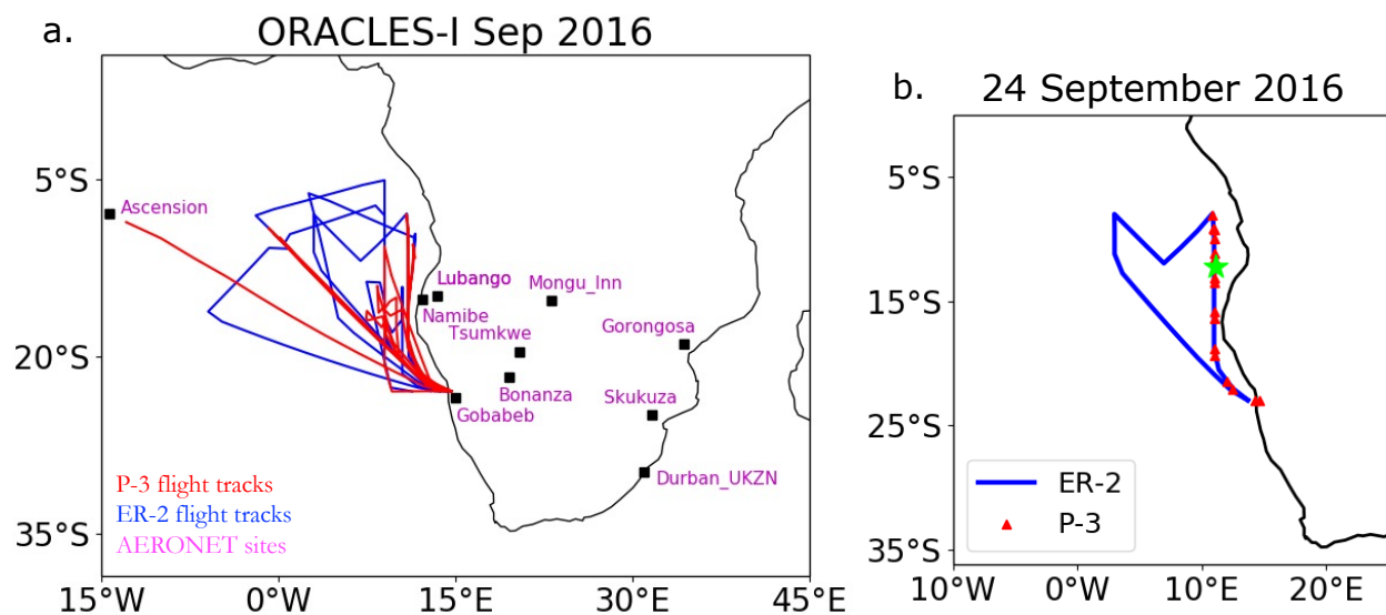
1045 Figure 1. (a) Location of ORACLES-I P-3 and ER-2 flights off southwestern Africa during September 2016 and ground-based AERONET sites over the continent. (b) P-3 and ER-2 flight tracks for September 24, 2016, with the green star highlighting the location of the vertical profile illustrated in later plots.
