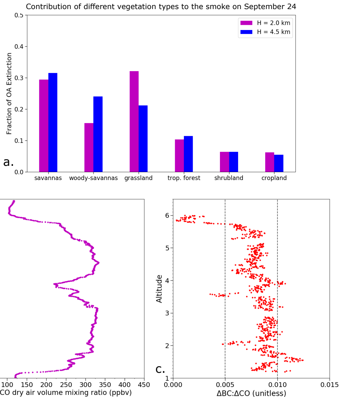
Figure 10. (a) Fraction of the OA extinction for the September 24, 2016, profile at 4.5 and 2 km altitude attributable to emissions from various types of vegetation burned. (b) P-3 observed carbon monoxide concentrations for the September 24, 2016, profile made near 12°S and 11°E. (c) Ratio of excess BC to carbon monoxide for the profile. Dashed lines demarcate regimes where smoldering (ratio < 0.005) and flaming (ratio > 0.01) conditions dominate.
