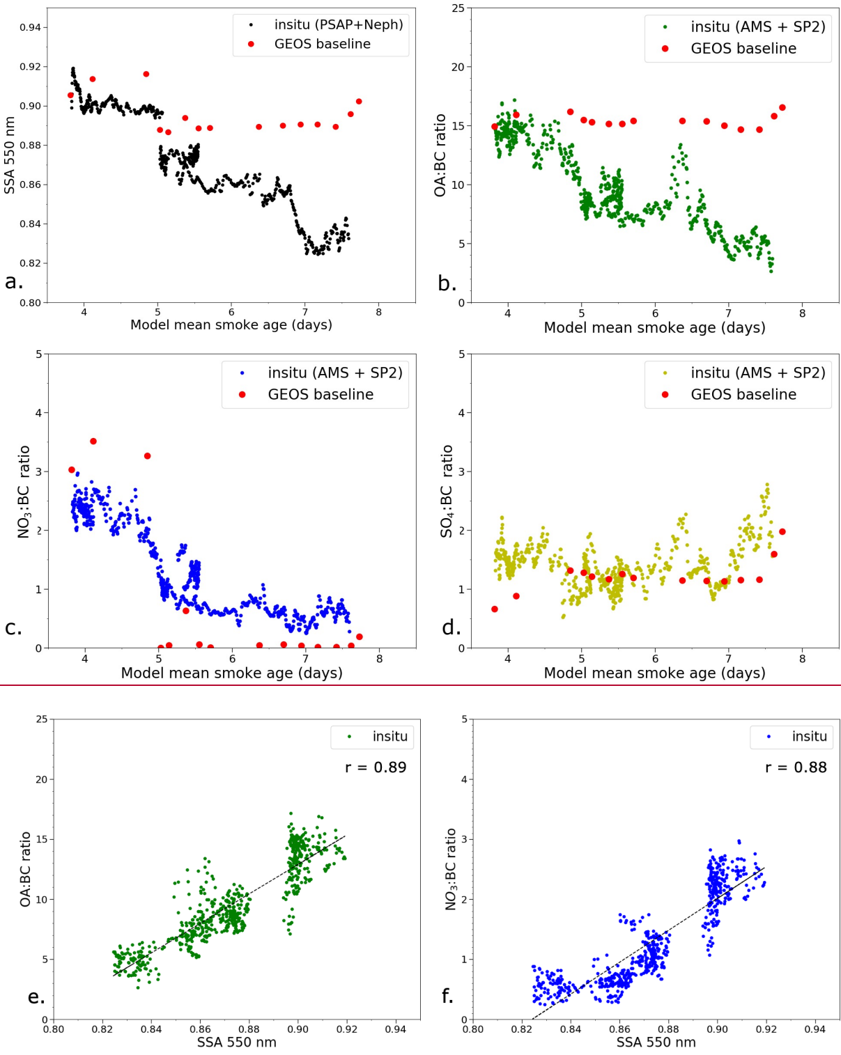
Figure 8. Observed and simulated (a) SSA at 550 nm, (b) OA:BC ratio, (c) \text{NO}_3 :BC ratio, and (d) \text{SO}_4 :BC ratio for the smoke layers near 12°S and 11°E flown by the P-3 on September 24, 2016. All the results are sorted by mean smoke age from the GEOS baseline simulation. Also shown are the correlation of OA:BC ratio (e) and \text{NO}_3 :BC (f) ratio against SSA.
