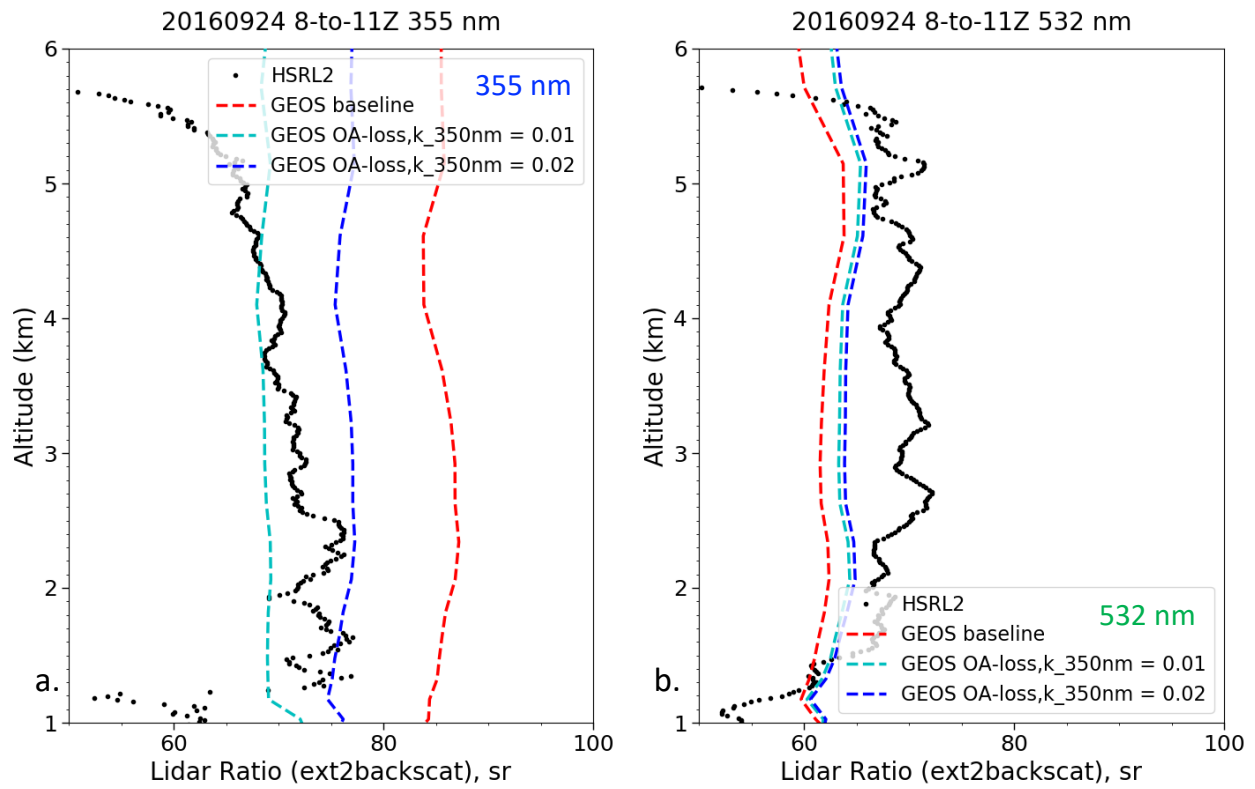
1125 Figure 14. Comparison of the simulated and HSRL-2 observed lidar ratios at (a) 355 nm and (b) 532 nm for the profile near 12°S and 11°E on September 24, 2016.
