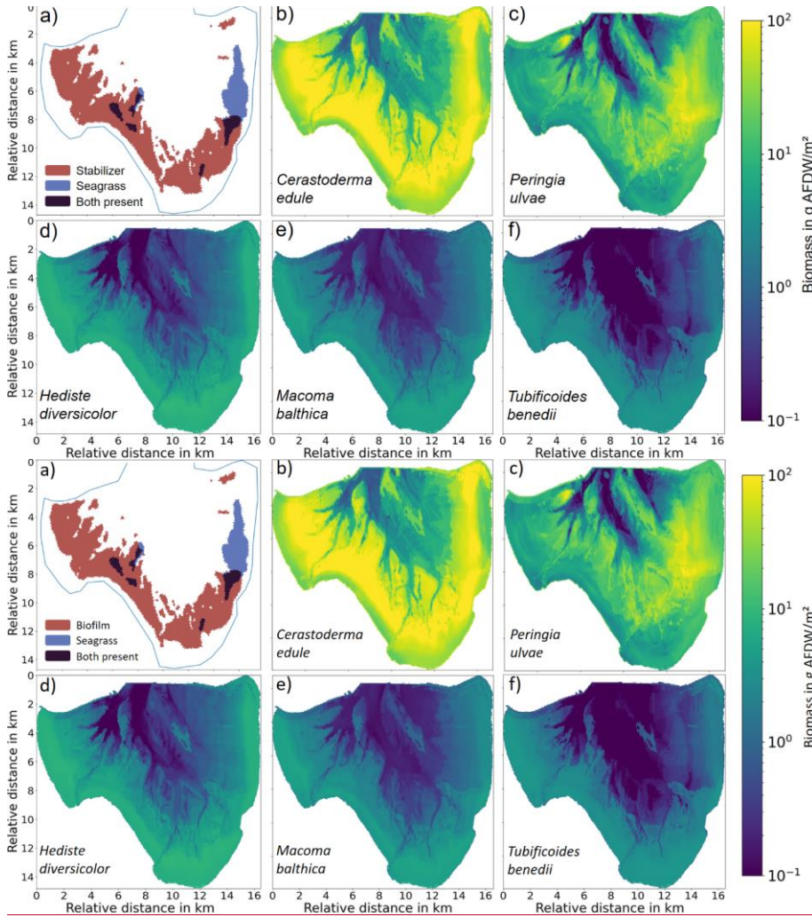
320 Figure 2. (a) Presence of stabilizers (MPB) and seagrass according to Adolph (2010); (b)-(f) Modeled biomass distribution of the five dominant benthic faunal species.
