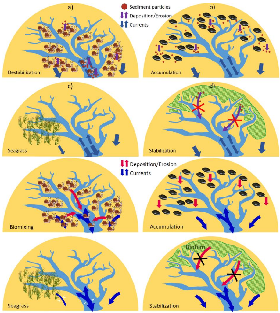
Figure 10. Conceptual sketch of different effects of the four functional groups on sedimentation and hydrodynamics in tidal embayments: (a) destabilization in tidal flats caused by bioturbators/biomixers , (b) accumulation caused by filter / suspension feeders, (c) modification of flooding / ebbing flows by seagrass meadows, and (d) sediment stabilization by MPB and reduced input to channels.
