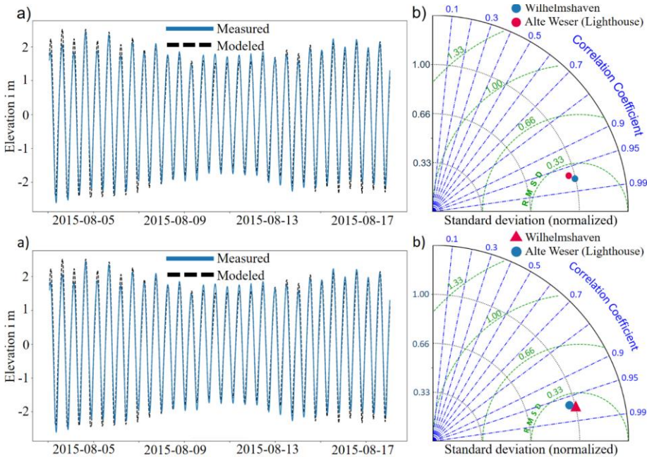
Figure 3. (a) Modeled and measured water elevation at the tide gauge station in Wilhelmshaven. (b) Comparison between model results and measurement at the gauge stations in Wilhelmshaven and the Lighthouse Alte Weser in a Taylor diagram.
