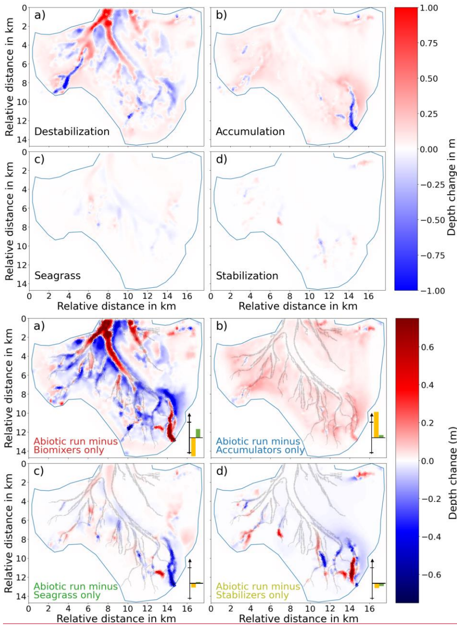
485 Figure 8. Difference in the depth change between the reference run Ref-bio no TS 10 and (a) Des-mix no TS 1 , (b) Acc-bio no TS 10 , (c) Gr-abgr no TS 10 and (d) Stab-bio no TS 10 . Positive and negative values indicate increased deposition and erosion, respectively, in the runs with benthos compared to the reference run. The bars in the
