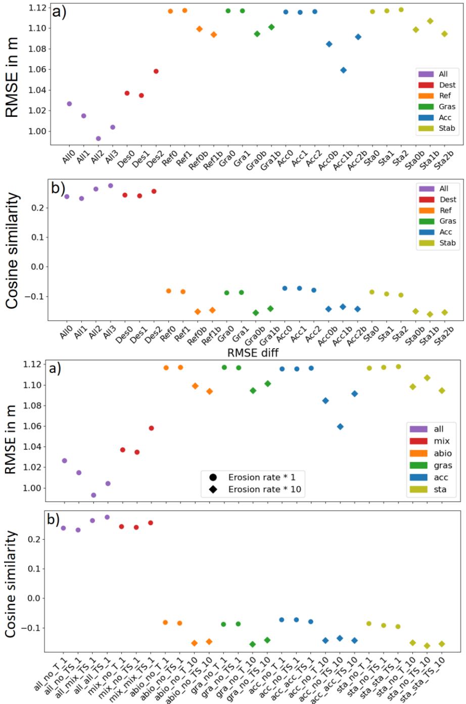
Figure 4. Performance of all simulations in terms of (a) RMSE between the modeled and measured water depth change
