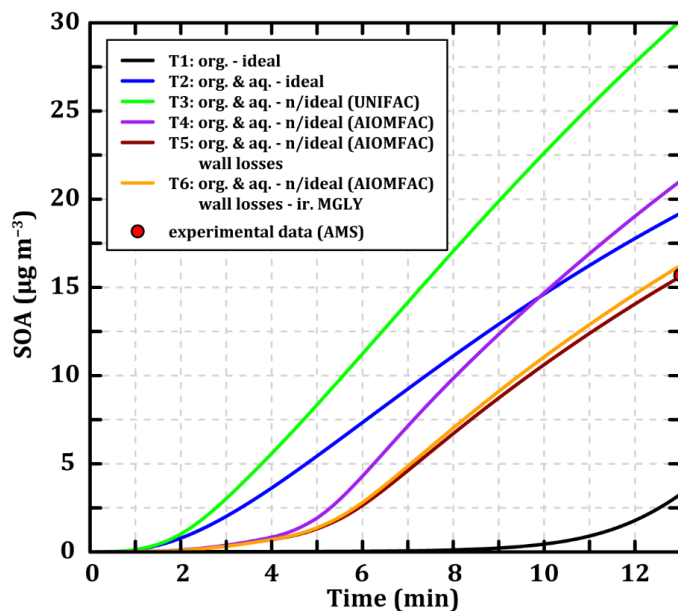
655 Figure 7: Temporal evolution of the SOA concentrations during toluene oxidation under experimental conditions (see sect. 2.2.3) simulated with MG-Cr-Al mechanism at 280 K considering mass transfer through an ideal organic phase (T1, black line), ideal
