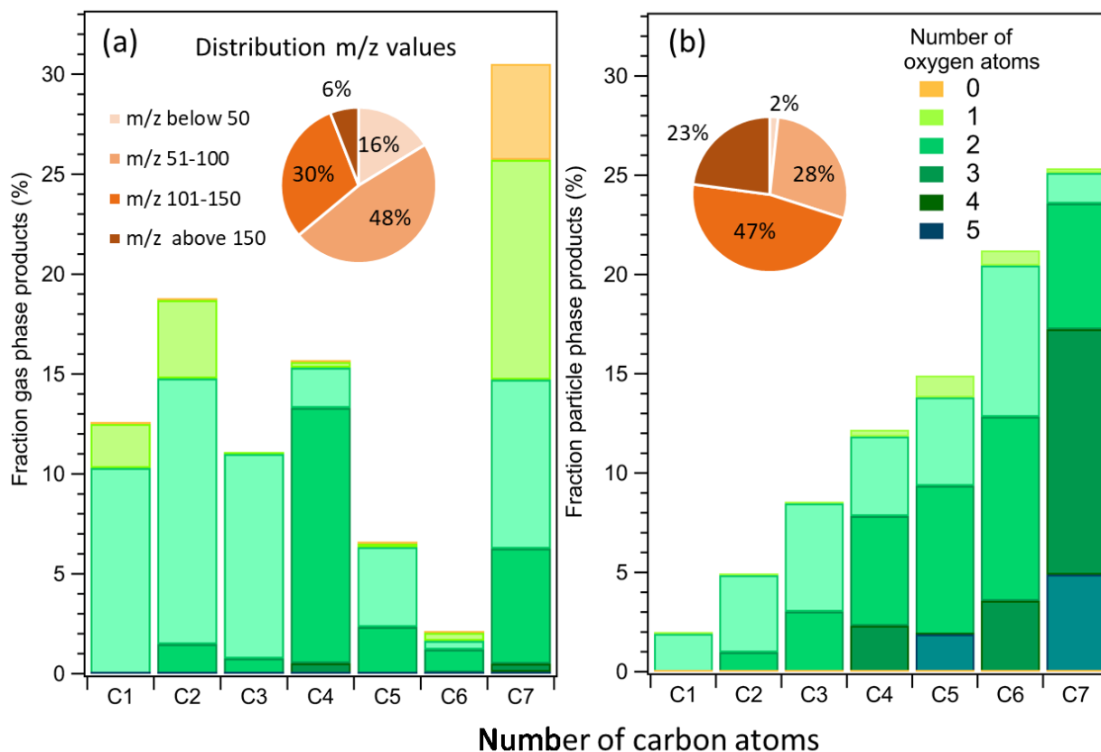
385 Figure 2: Mass products fraction (y-axis) distribution based on the number of carbon atoms (x-axis) for an experiment with 112 ppbv toluene at 280 K. Detected ions in the (a) gas phase and (b) particle phase. Pie charts correspond to the molecular weight contribution to the overall mass.
