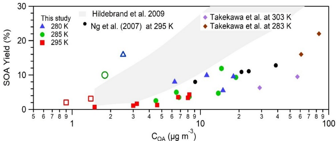
355 | Figure 1: SOA yield (measured by HR-ToF-AMS) vs organic aerosol formed. Red squares refer to 295 K, green circles stand for 285 K and blue triangles represent data points at 280 K. Empty markers present experiments with low toluene concentration (8 and 23 ppbv), filled markers indicate high toluene concentration experiments (above 110 ppbv). Data points from this work are compared with toluene experiments from Ng et al. (2007), Hildebrandt et al. (2009) and Takekawa et al. (2003).
