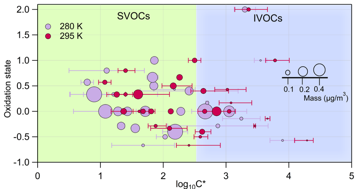
Figure 3: The oxidation state for the detected parent ions (OSc), versus the averaged saturation concentration in terms of \log_{10}C_i^* . The area size of the dots denotes the mass of associated to each species. In light violet are represented the ions fragments identified for an experiment carried out at 280 K and in magenta those at 295 K. Errors bars correspond to \pm 1\sigma of the experimental average. Pie charts show the percent of mass measured by Charon when adding all the parent ions compared to the total organic mass evaluated by the AMS at the two experimental temperatures.
