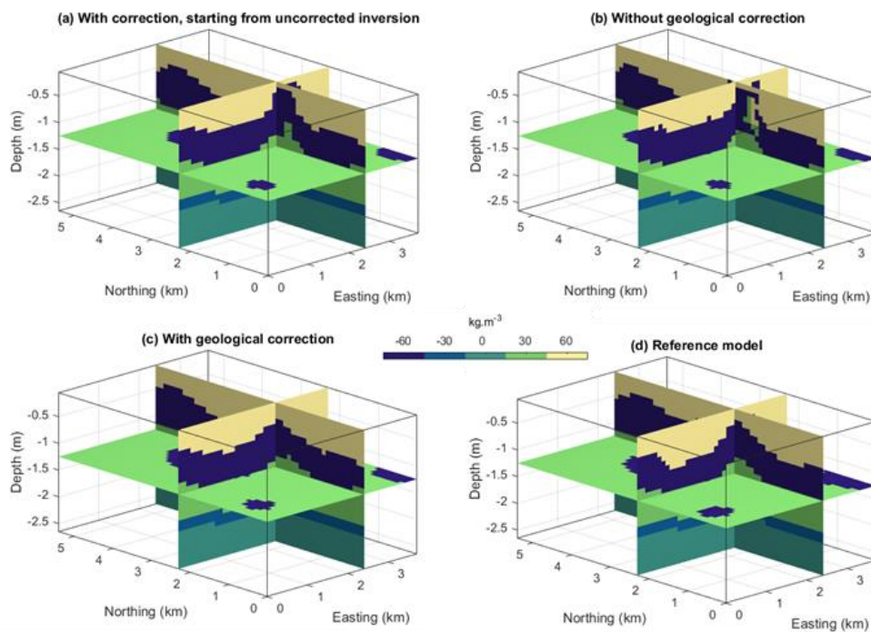
565 Figure 14. Comparison of inversion results with (a) geological correction starting from inverted model obtained without geological correction, as shown in (b); results with geological correction (c) and reference model (d).
