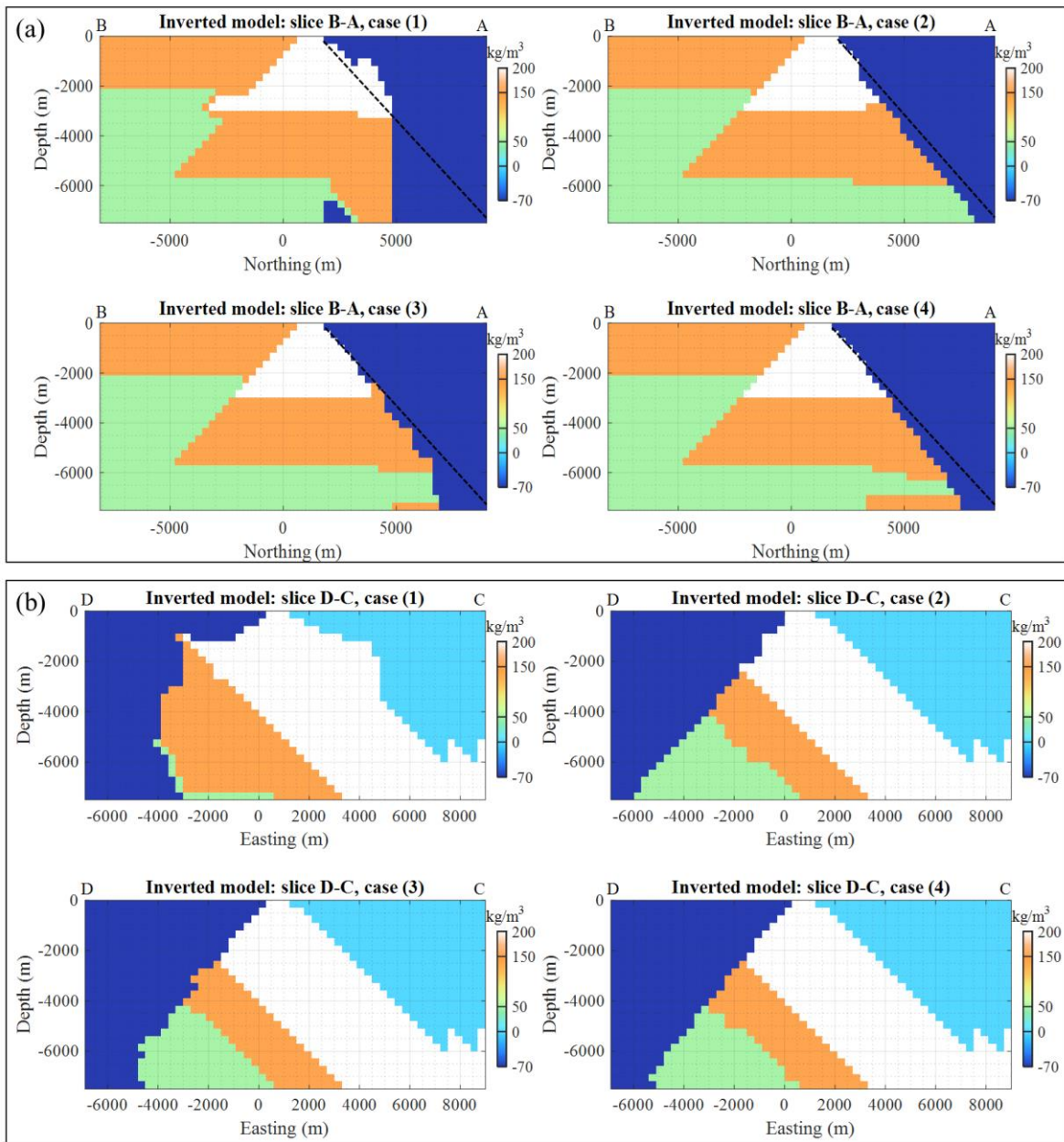
Figure 12. Inversion results for cases (1) through (4) along section B-A (a) and D-C (b). In (a) The true location of the unconformity is indicated by the black dashed line.
