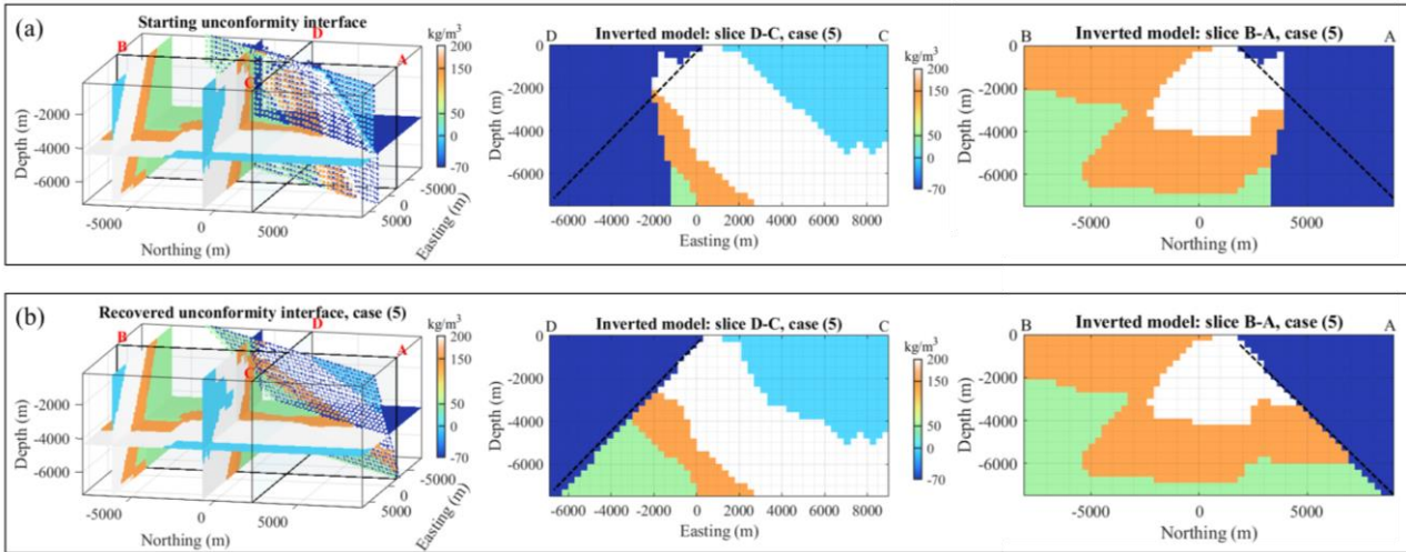
Figure 15. (a) starting model and (b) inverted model. From left to right, the views are the same as displayed in Figure 11, and Figure 12, respectively.
