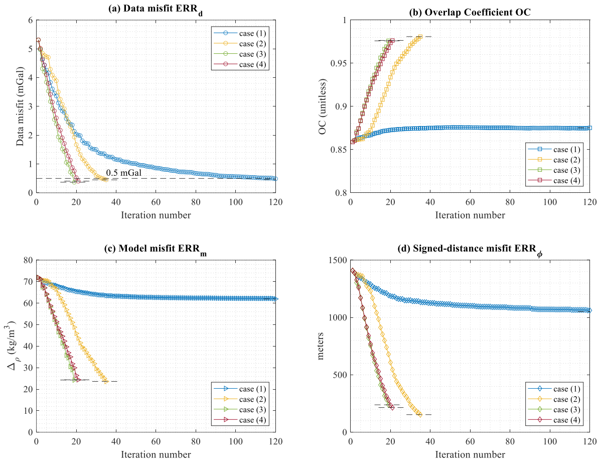
Figure 13. Inversion metrics for cases (1) through (4): data misfit (a), Overlap Coefficient (b), model misfit (c) and signed-distance misfit (d).
