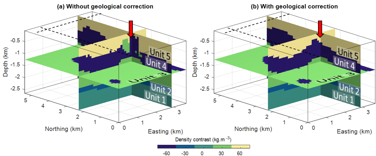
395 Figure 5. Inversion results for proof-of-concept: without application of geological correction (a) and using geological correction (b). Modified and adjusted from Giraud et al. (2022).
