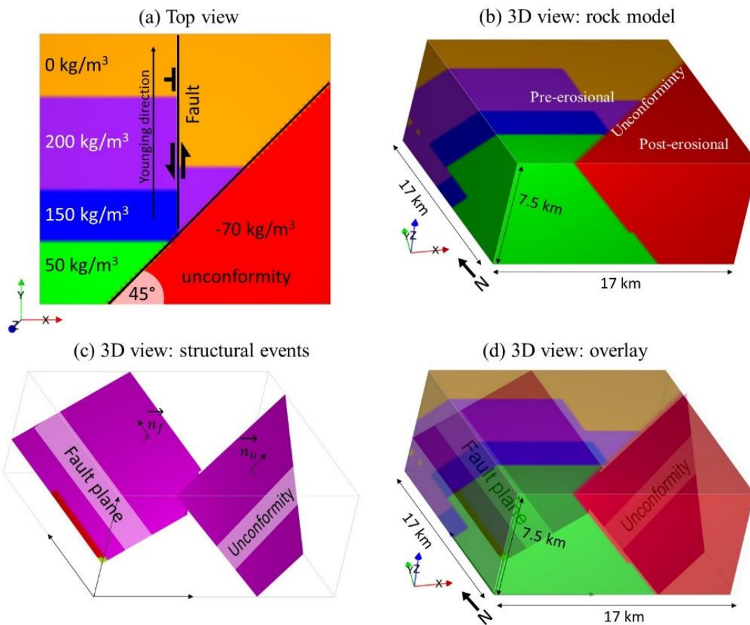
465 Figure 7. Reference geological model and density contrasts: (a) top view, (b) 3D rock unit cube and (c) structural events, overlaid in (d).
