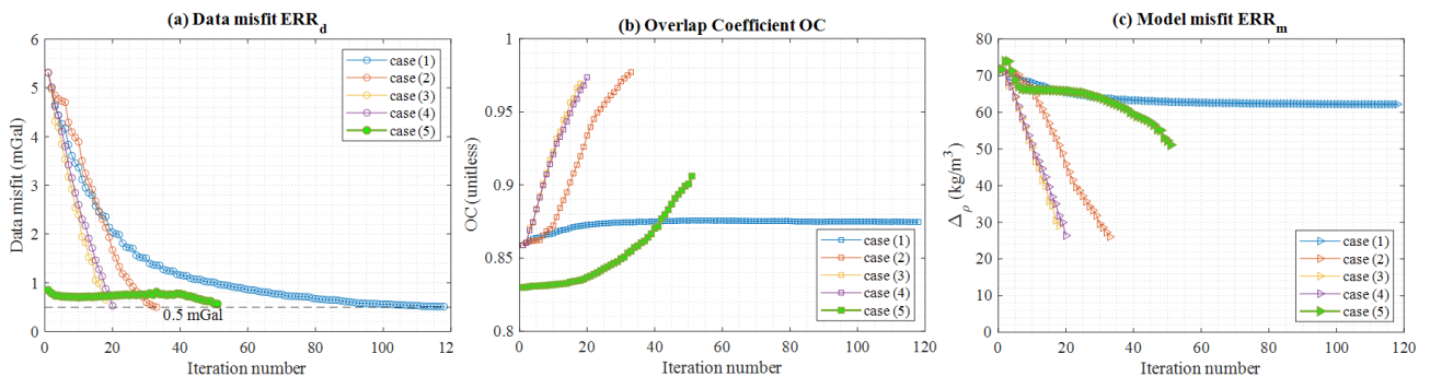
Figure 16. Comparison of inversion metrics for cases 1-4 with case 5.
