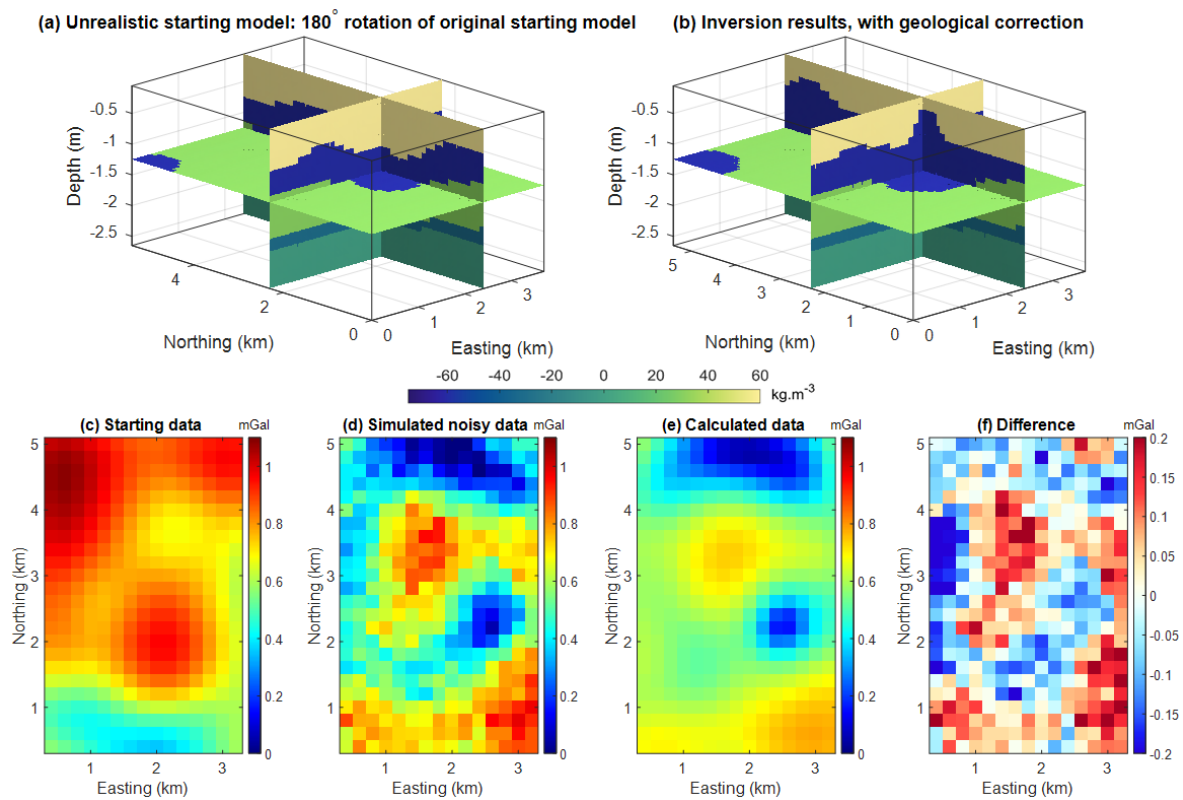
Figure 18. Simulation of a degenerate case. Top row: starting (a) and inverted model (b). Bottom row: starting data (c), data contaminated by noise (d), calculated data from the inverted model (e), and difference between inverted and calculated data (f).
