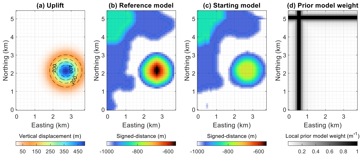
365 Figure 3. (a) Dome added to the original model, (b) reference model: signed distance field of unit 1 at depth equal to -1000 meters, (c) starting model: signed distance field of unit 1 at depth equal to -1000 meters, (d) weights W_p assigned to the prior model term in Eq. (4). We note that the starting model as shown in (c) also corresponds to the prior model.
