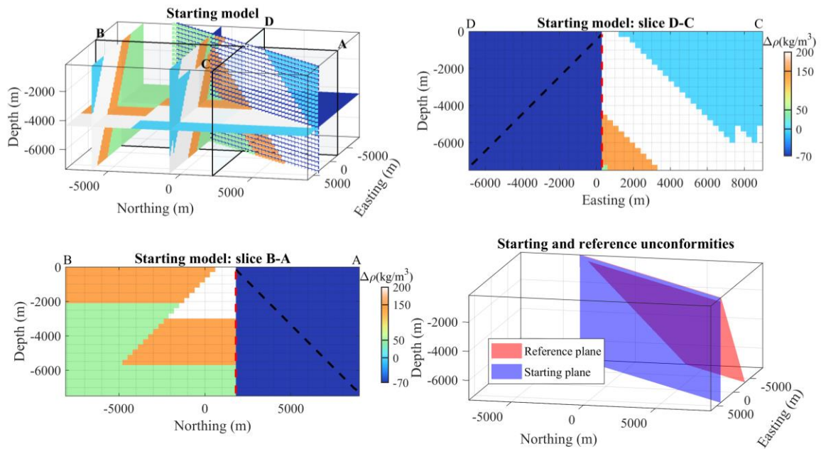
Figure 9. Starting model visualised in 3D view, slices, and representation of the unconformity plane. The black dashed line represents the location of reference (or true) unconformity plane.
