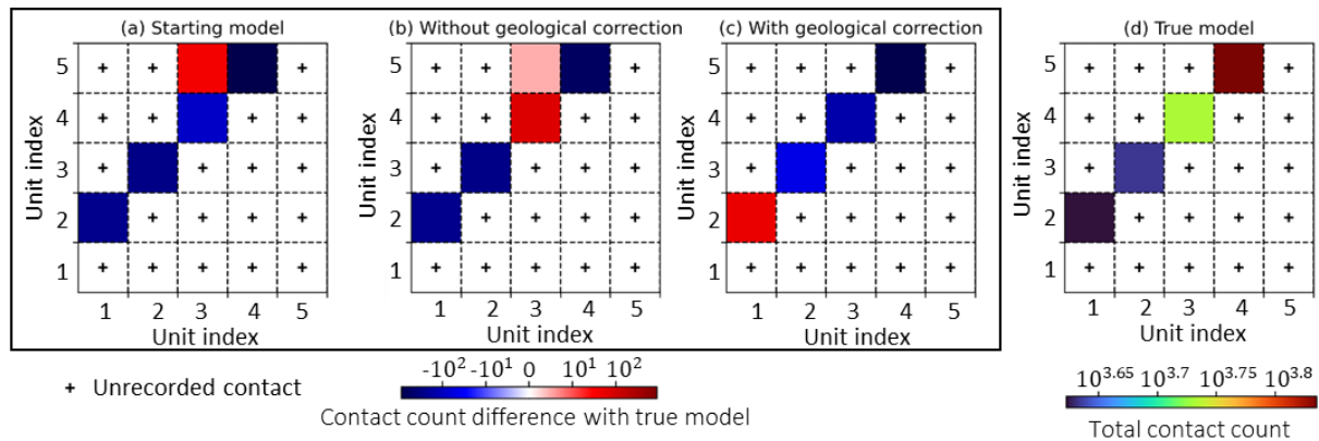
Figure 6. Adjacency matrices: differences between the starting model (a), inverted model without geological correction (b), and with geological correction used during inversion (c); (d) shows the adjacency matrix of the true model. Adjacency relationships are represented using upper triangular adjacency matrices as adjacency relationships are symmetric. The diagonal is left empty because we do not record occurrences of a rock in contact with itself.
