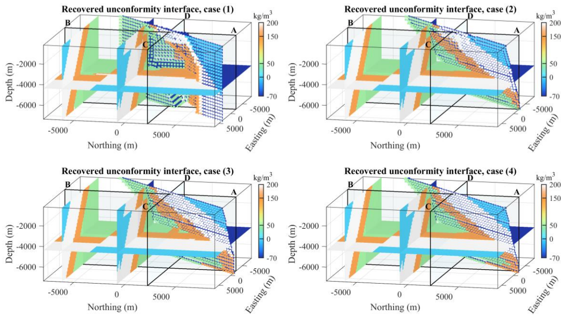
Figure 11. 3D visualisation of Inversion results for cases (1) through (4). The differences between the best fitting planes corresponding to the recovered uniformity interface shown here and the reference plane (Fig. 9) amount to 11.9, 3.2, 5.7, and 4.6 degrees for cases (1) through (4), respectively.
