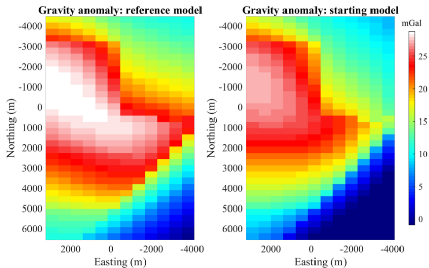
Figure 10. Gravity data simulated for the reference model (left), which we consider as the field data to honour, and for the starting model (right), which corresponds to the starting point of all inversion scenarios.
