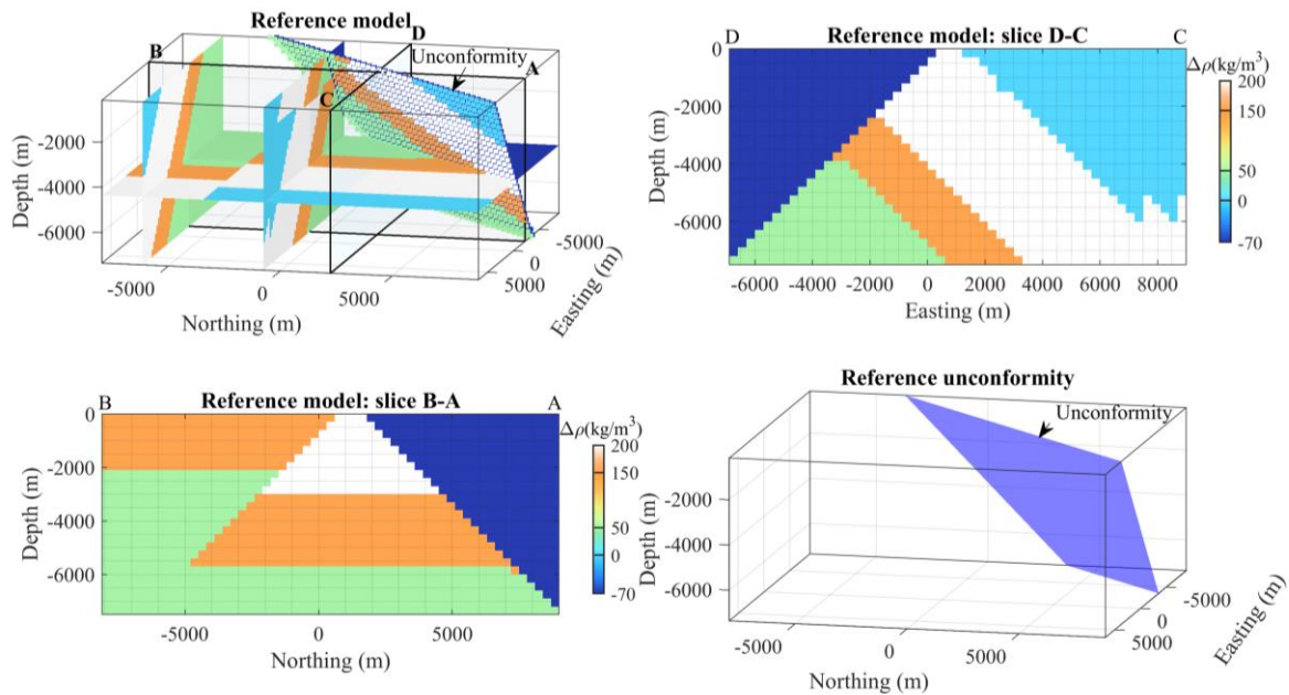
Figure 8. Reference model visualised in 3D view, slices, and representation of the unconformity plane.
