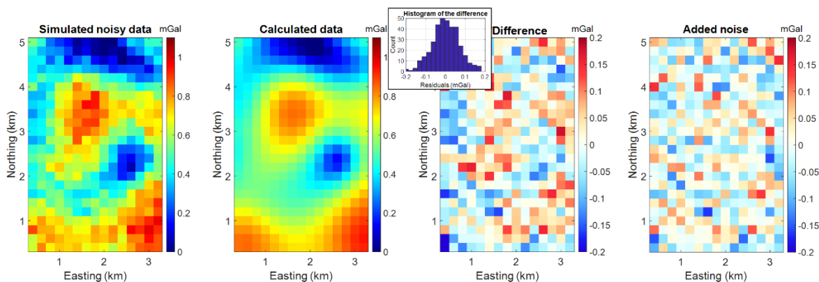
Figure 17. Simulation of noisy data. From left to right: data contaminated by noise, calculated data from the inverted model, difference between inverted and calculated data with histogram and noise that was added to the data..
