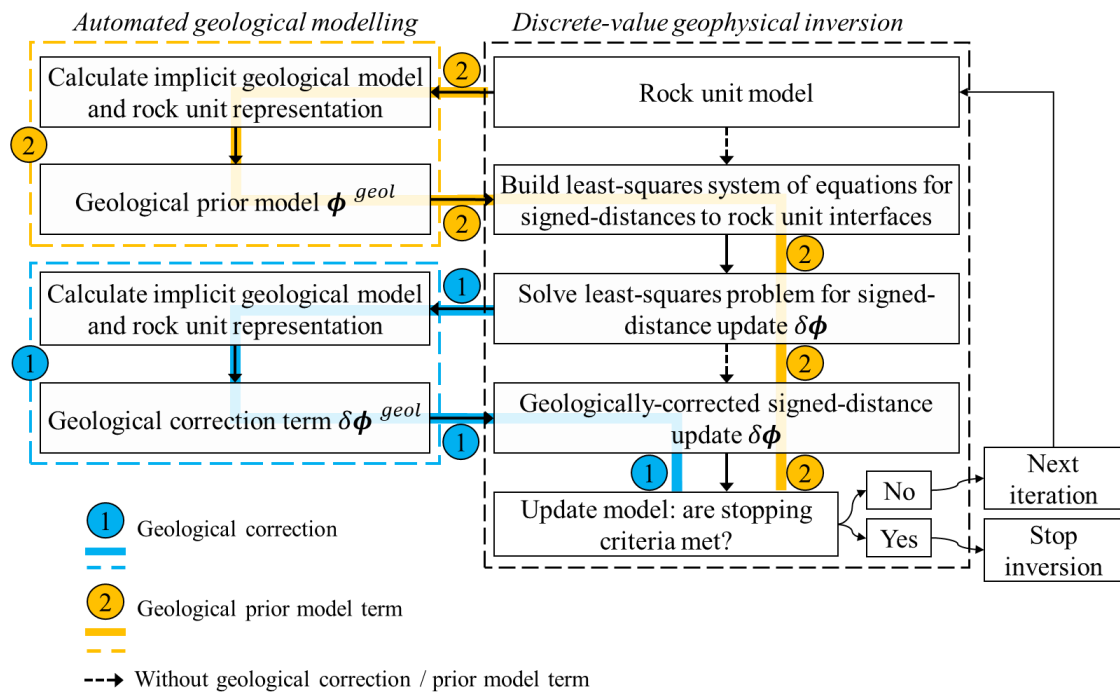
Figure 2. Summary of the proposed approaches to integrated geological modelling in geophysical inversion: iterative use of the geological correction term with a fixed prior (1) or update of the prior geological model (2). Note that the combination of both is possible. Modified from Giraud et al. (2022).
