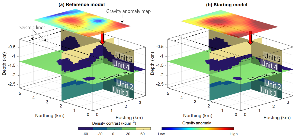
385 Figure 4. Synthetic model for proof-of-concept testing: reference model (a) with the corresponding gravity anomaly shown in transparency and starting model (b). The location of the seismic sections used to derive the prior model is shown by the dashed lines. The red arrow shows the dome location. The two colour bars and their respective palettes are common to (a) and (b). Modified and adjusted from Giraud et al. (2022).
