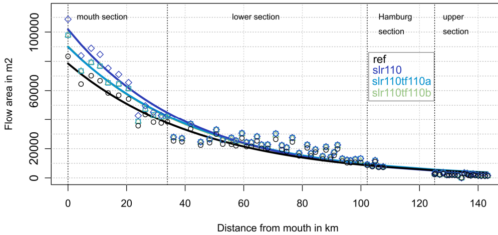
375 Figure 8: Cross-sectional flow area A analysed for each control volume boundary along the estuary profile (markers) and fitted regression model (lines) for the scenarios ref (black), slr110 (dark blue, rhombuses), slr110tf110a (light blue, squares), slr110tf110b (green, triangles). (The results of scenarios slr110tf55a and slr110tf55b are not shown in the figure for better readability.)
