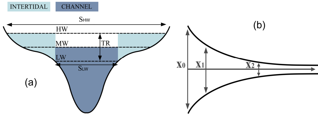
335 Figure 6: (a) Schematic cross-section with channel and intertidal volume, high water ( HW ), mean water level ( MW ) and low water ( LW ), tidal range ( TR ) and surface area at HW and LW ( S_{HW} and S_{LW} ); (b) schematic plan view of a funnel-shaped estuary.
