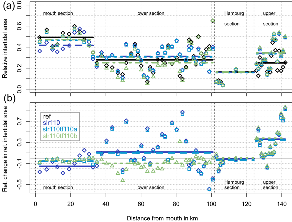
Figure 10: Relative intertidal area (a) and relative change in relative intertidal area (b) in each control volume (markers) and section (lines) along the estuary for scenarios ref (black), slr110 (dark blue rhombuses), slr110tf110a (light blue squares), slr110tf110b (green triangles). (The results of the scenarios slr110tf55a and slr110tf55b are not shown in the figure for better readability.)
