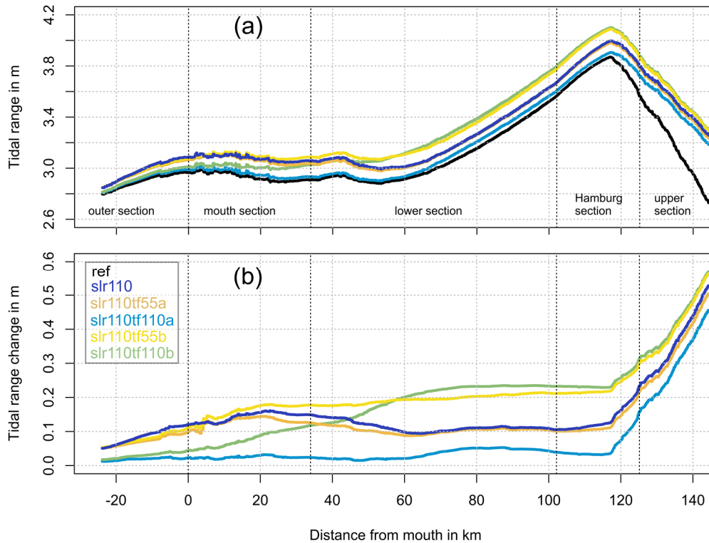
355 Figure 7: TR in m (a) and change in TR relative to reference condition in m (b) along the estuary profile analysed for a spring–neap cycle for scenarios ref (black), slr110 (dark blue), slr110tf55a (orange), slr110tf110a (light blue), slr110tf55b (yellow), slr110tf110b (green).
