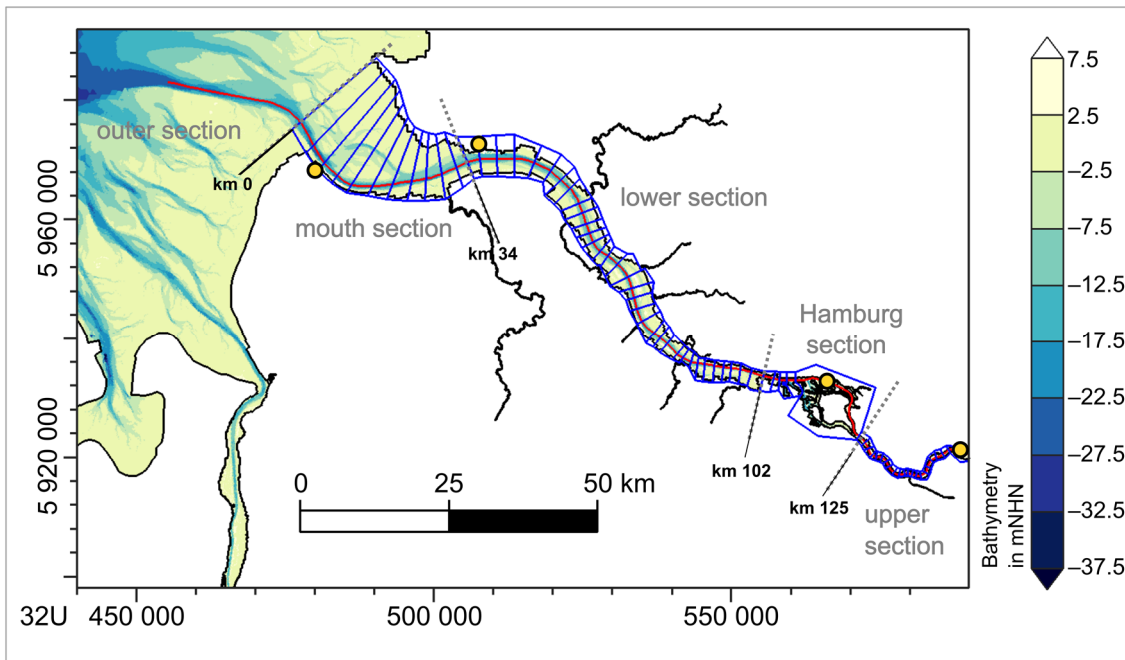
Figure 5: Model excerpt of the Elbe estuary showing the profile along the estuary (red) and a subdivision into 5 sections (grey) and 71 control volumes (blue) that are used for the analysis of the simulation results. The yellow markers represent the following locations from left to right: Cuxhaven, Brunsbüttel, St. Pauli (Hamburg Port) and Geesthacht.
