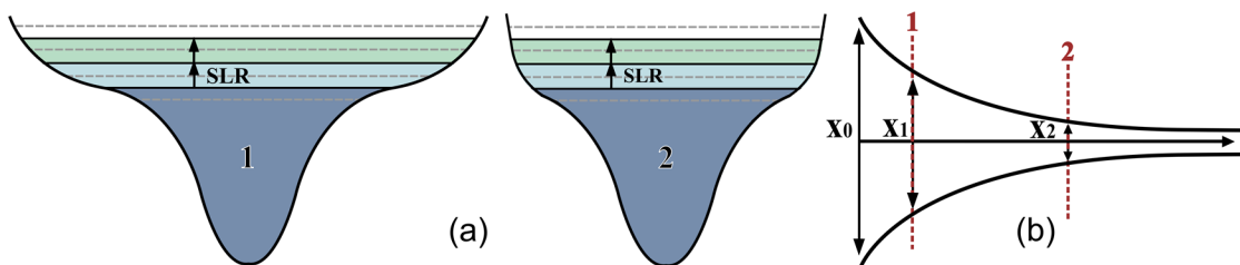
Figure 11: Schematic of SLR in estuary cross-sections (a) with large (1) and small (2) S_{INT} and schematic plan view of an estuary (b). The black lines in the cross-sections show the MW for a reference scenario (dark blue) and two SLR scenarios (light blue and light green).
