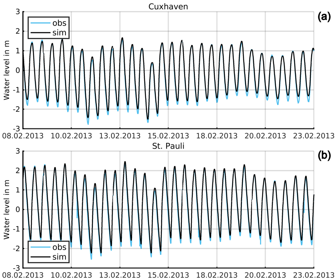
Figure A2: Simulated (black) and observed (blue) water levels at the stations in Cuxhaven (a) and St. Pauli (b).
