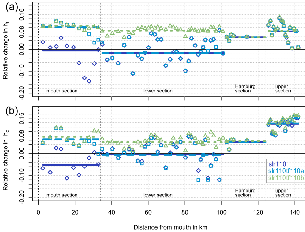
405 Figure 9: Relative change in mean hydraulic depth ( h_t a) and h_c b) in each control volume (markers) and each section (lines) relative to reference condition for scenarios slr110 (dark blue rhombuses), slr110tf110a (light blue squares), slr110tf110b (green triangles). (The results of scenarios slr110tf55a and slr110tf55b are not shown in the figure for better readability.)
