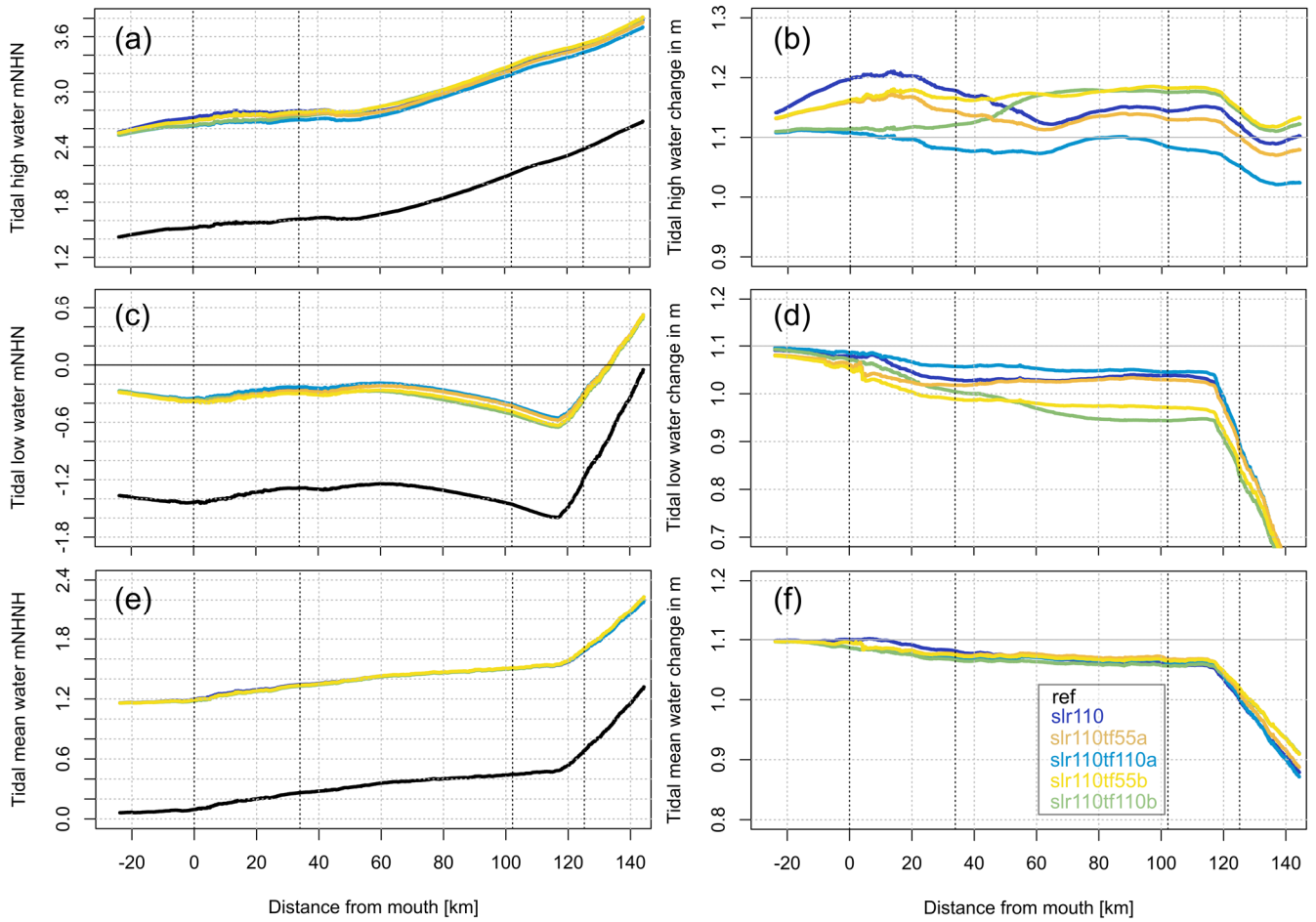
600 Figure A1: HW (a), LW (c) and MW (e) relative to mNHN (German vertical datum) and changes in these parameters relative to reference condition in m (b, d and f) along the estuary profile analysed for a spring-neap cycle for the scenarios ref (black), slr110 (dark blue), slr110tf55a (orange), slr110tf110a (light blue), slr110tf55b (yellow), slr110tf110b (green).
