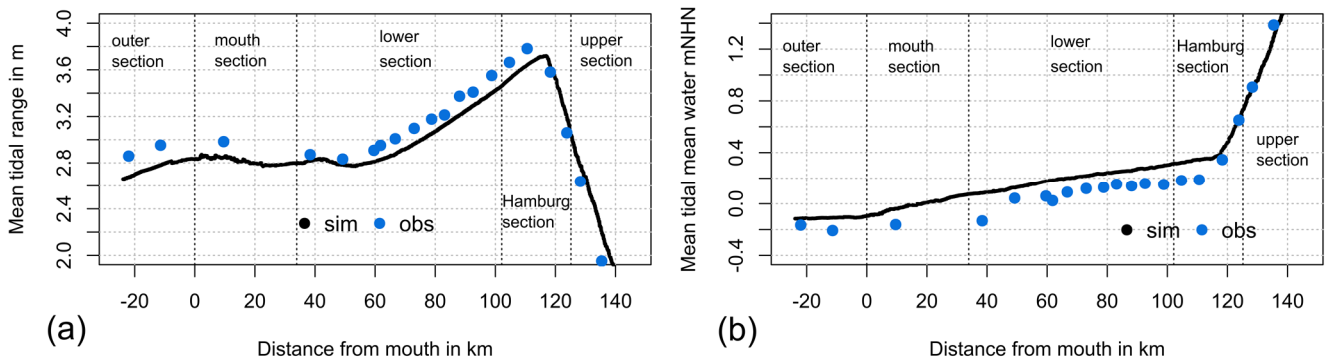
Figure 3: TR (a) and MW (b) above mNHN (meters above the German datum) averaged over 7 spring–neap cycles from January 2013 to April 2013 along the Elbe estuary, calculated from observations (blue) and from simulation results (black).
