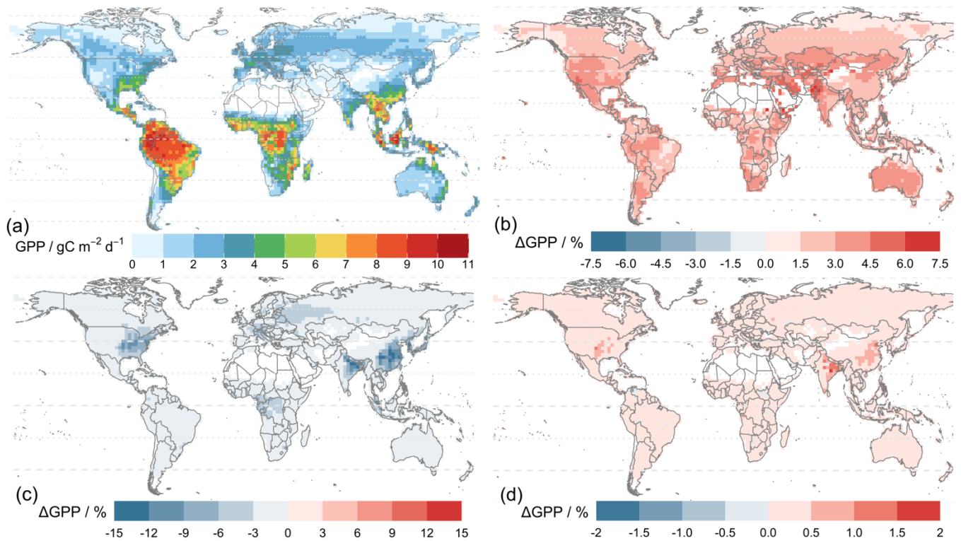
Figure 10: Plots showing results from simulations of Table 3: (a) gross primary product (GPP) modeled for year 2000 at a CO 2 concentration of 370 ppmv (C0_O0), (b) percentage changes in GPP showing CO 2 fertilization effects of year-2010 CO 2 concentration at 390 ppm ( 100\% \times (\text{C1\_O0} - \text{C0\_O0})/\text{C0\_O0} ), (c) percentage changes in GPP due to O 3 damage at high sensitivity of the Sitch O 3 damage scheme for year-2000 modeled O 3 concentration and CO 2 concentration of 370 ppmv ( 100\% \times (\text{C0\_O1} - \text{C0\_O0})/\text{C0\_O0} ), and (d) differences in percentage O 3 damage at a CO 2 concentration of 390 ppmv from that at 370 ppmv ( 100\% \times (\text{C1\_O1} - \text{C1\_O0})/\text{C1\_O0} - 100\% \times (\text{C0\_O1} - \text{C0\_O0})/\text{C0\_O0} ), whereby positive values indicate a reduction in percentage O 3 damage.
