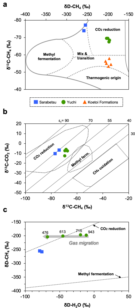
215 Figure 2. Relationships between (a) \delta D and \delta^{13}C of methane, (b) \delta^{13}C of methane and \delta^{13}C of carbon dioxide, and (c) \delta D of 220 methane and \delta D of water for water samples from the upper Sarabetsu Formation (■) and the Yuchi Formation (●). The origins of methane are estimated in each plot according to Whiticar (1999). In (a), data for water samples from the Koetoi Formation (triangles) (Tamamura et al. 2014) are shown for comparison. The light gray diagonal lines in (b) indicate carbon isotopic fractionation contours ( \epsilon_c \approx \delta^{13}C-CO_2 - \delta^{13}C-CH_4 ). In (c), the depths (mbgs) of water samples from the Yuchi Formation are indicated.
