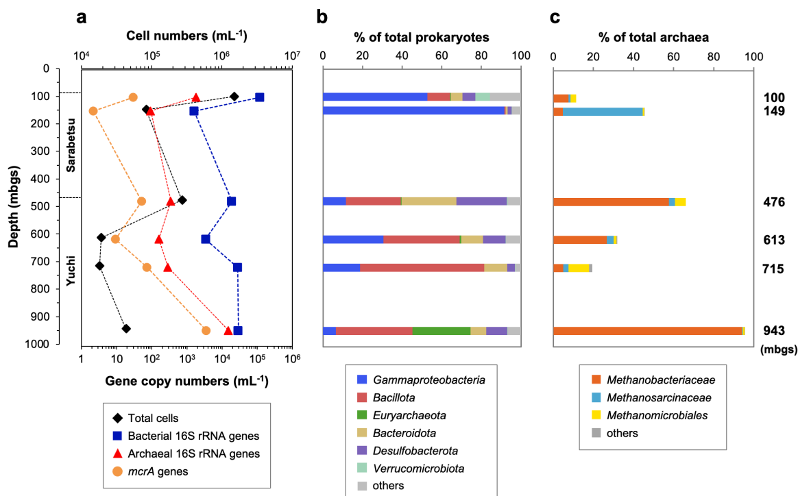
Figure 3. Depth-related changes in (a) microbial populations and (b) prokaryotic and (c) methanogenic community compositions based on the 16S rRNA gene sequences in water samples.
