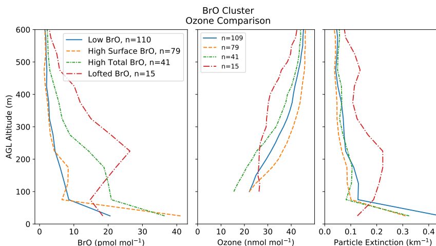
Figure 11. The ozone mixing ratio (middle) and 361 nm particle extinction (right) profiles associated with the four BrO profile clusters. The variability of these parameters is not shown here for clarity, but is indicated with error bars in the supplement (Figures S8 and S9).
