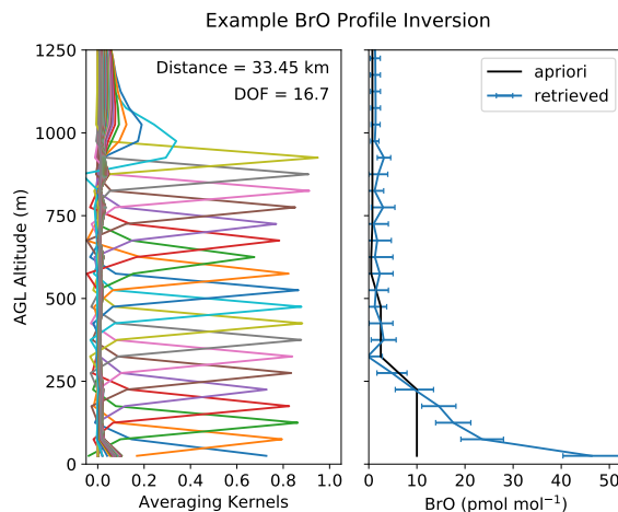
Figure 3. Example BrO profile retrieval from the fifth aircraft profile on March 30 with the averaging kernels on the left showing very good resolution and a high total DOF (16.7). The a priori profile is shown in black and the retrieved profile and uncertainty are shown in blue on the right. This vertical profile spanned a horizontal distance of 33.45 km.
