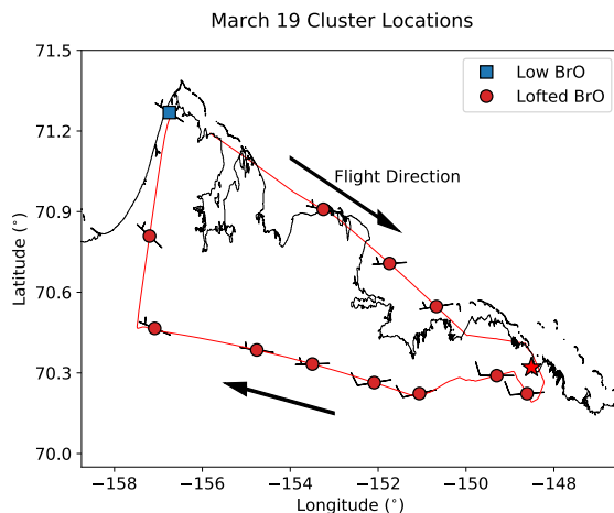
Figure 6. Identified BrO profile clusters for the research flight on March 19, 2022. The flight path is shown in red, beginning in Utqiagvik and heading east along the coast of the Beaufort Sea before turning to the west around Prudhoe Bay (indicated with a star) and returning back over the tundra. The markers indicate the identified cluster and are plotted at the location of the aircraft profile, with the mean wind speed and direction from ALAR meteorological data denoted with the wind bars. Lofted BrO profiles were identified everywhere throughout the flight, except at Utqiagvik.
