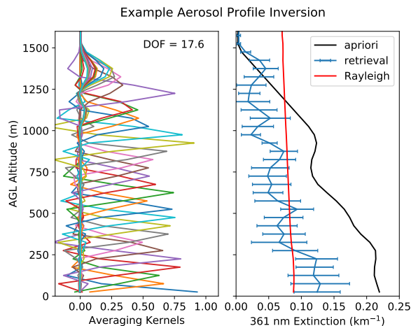
Figure 2. Example retrieval of the average particle extinction profile from March 30 with the averaging kernels on the left (DOF of 17.6) and the extinction profile on the right. The a priori extinction is based on the profile shape from the Grimm particle number density from throughout the flight scaled to Aeronet observations at the ARM facility. VLIDORT modelled how light at 361 nm reached our telescopes to perform the O_4 inversion, and thus retrieves the 361 nm particle extinction. VLIDORT uses a bulk Mie code to determine aerosol optical properties at other wavelengths. The impact of Rayleigh scattering is shown in red, indicating that the particle and molecular extinction are comparable at the surface for this day.
