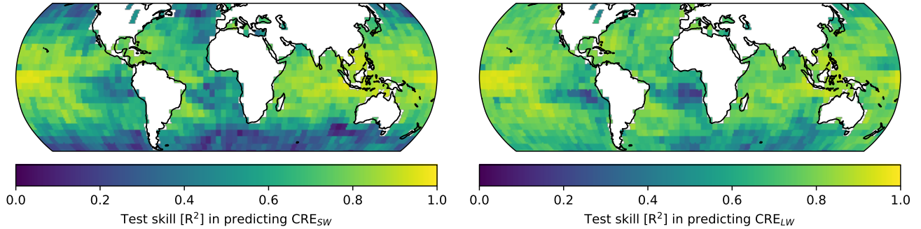
Figure 4. Skill ( R^2 score) of the ridge regression models to predict CRE_{SW} (left) and CRE_{LW} (right) in the independent test data (2016–2020).
