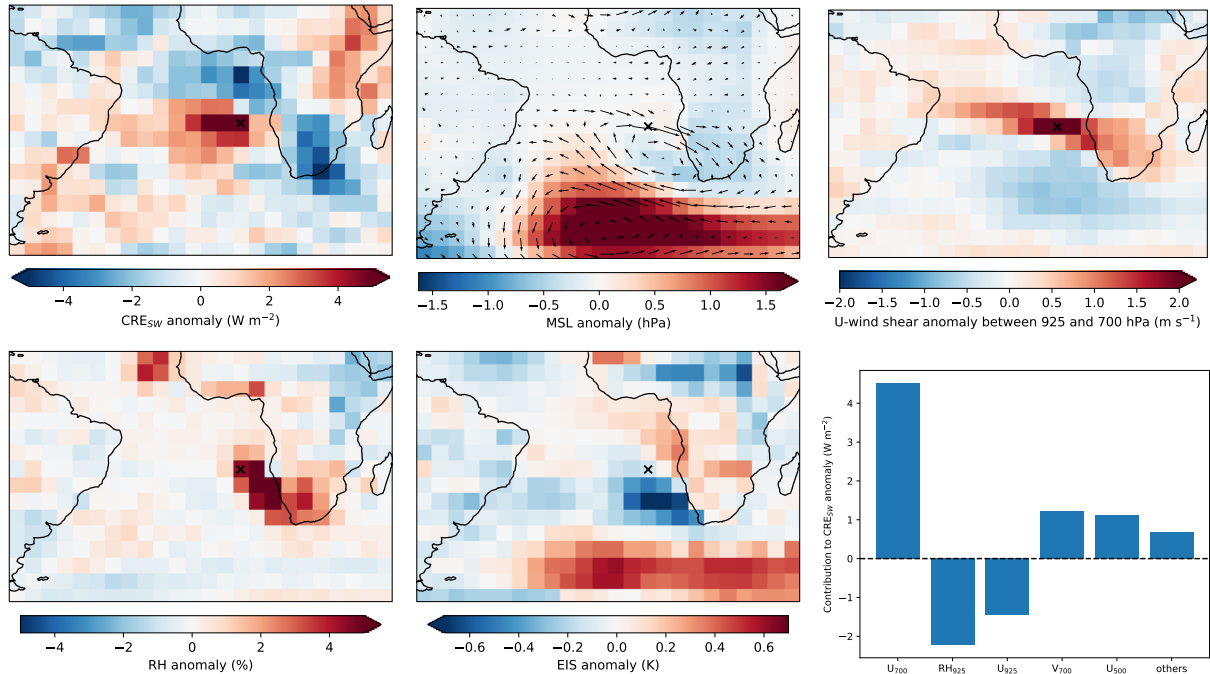
Figure 9. Composite analysis of anomalies in CCFs and CRE_{SW} when U_{700} anomalies in the Southeast Atlantic at 17.5^{\circ}S and 2.5^{\circ}E (black "x") > 1\sigma . The panel in the top left shows the observed CRE_{SW} anomalies in these situations. The top center panel shows the MSL anomalies and wind anomalies at 700 hPa, and the top right panel shows the wind shear anomaly of the u-component between the boundary layer (925 hPa) and the free troposphere (700 hPa). The bottom left panel shows the RH anomaly in the boundary layer (925 hPa), and the bottom center panel shows EIS anomalies. The panel in the bottom right shows the ridge-regression quantified contributions of selected CCFs and the sum of all others to the predicted CRE_{SW} .
