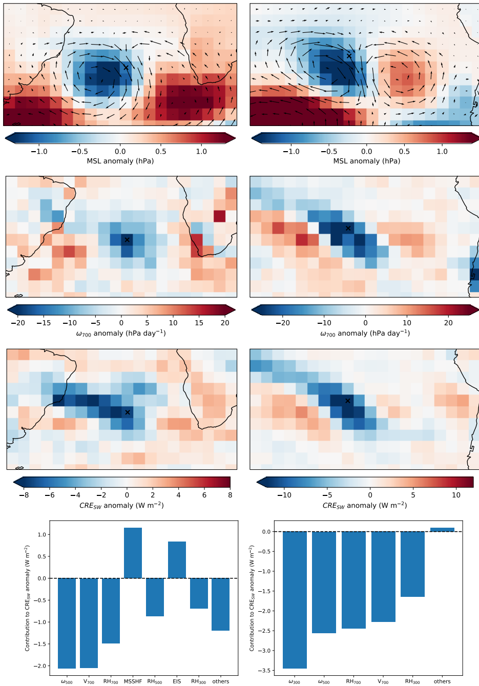
Figure 11. Composite analysis of anomalies in CCFs and CRE_{SW} when V_{700} in the Southeast Atlantic (left: at 27.5°S and 12.5°W) and in the South Pacific (right: at 22.5°S and 127.5°W) > 1\sigma . From top to bottom, the panels show MSL anomalies and wind anomalies at 700 hPa, \omega_{700} anomalies, observed CRE_{SW} anomalies, and ridge-regression quantified contributions to the predicted CRE_{SW} anomaly.
