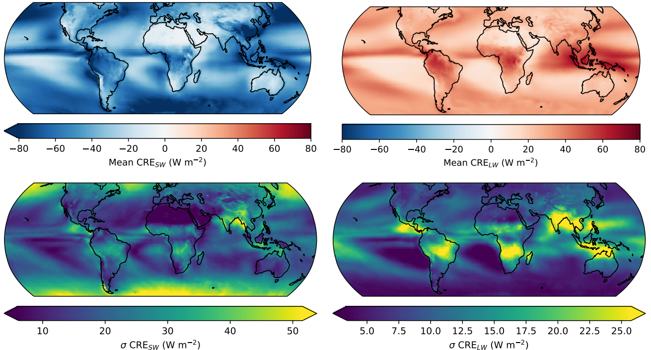
Figure 1. Climatological (2001–2020) mean (top) and standard deviation (bottom) of CRE_{SW} (left) and CRE_{LW} (right) from the CERES EBAF data. Pointy ends of the colorbars indicate that not the entire value range is shown in the figure to improve its clarity.
