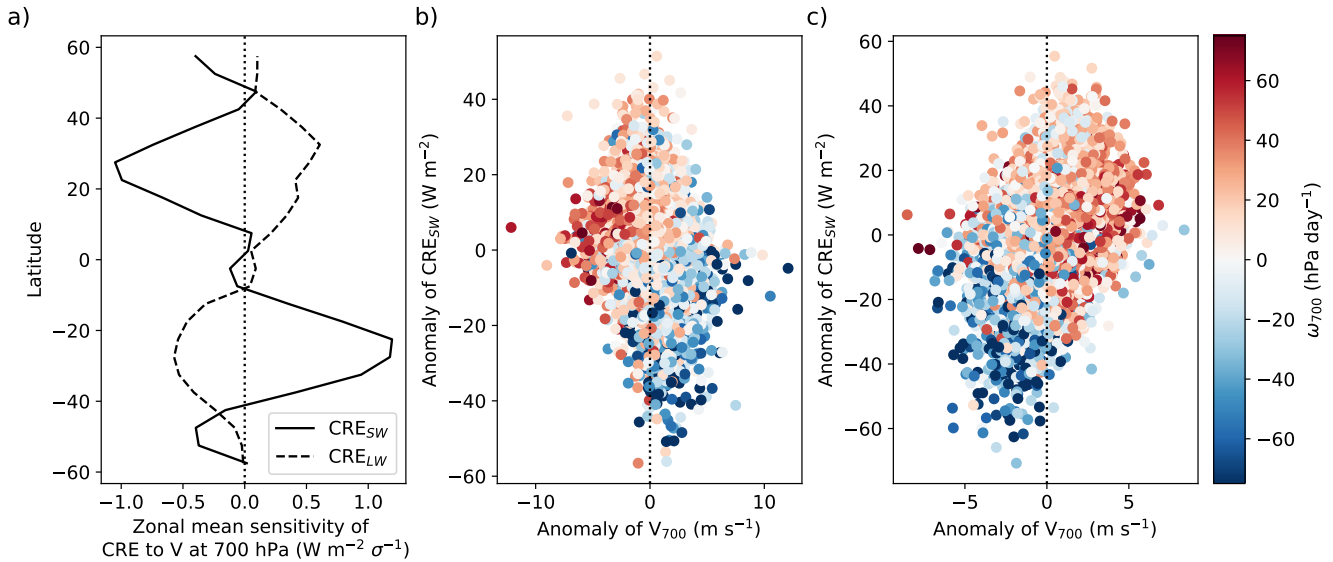
Figure 10. Summary of the CRE sensitivity to V_{700} anomalies. a) Zonal mean sensitivities of CRE_{SW} (solid line) and CRE_{LW} (dashed line) point to strong sensitivities in the subtropics. b/c) show the CRE_{SW} anomaly against the V_{700} anomalies in the Northern (centre panel) and Southern (right-hand panel) Hemisphere where the absolute value of the sensitivity exceeds \pm 1.5 W m^{-2} \sigma^{-1} , with the color showing \omega_{700} (blue: ascent, red: subsidence).
