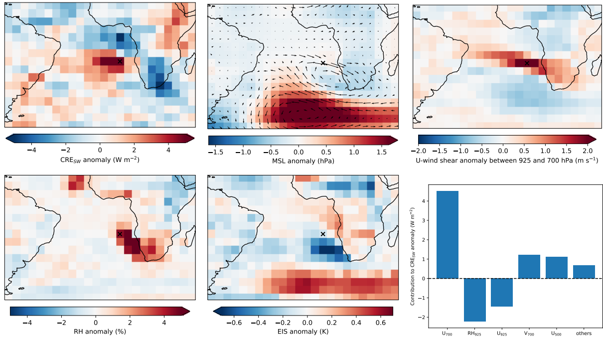
Figure 9. Composite analysis of anomalies in CCFs and CRE_{SW} when U_{700} anomalies in the Southeast Atlantic at 17.5^{\circ}S and 2.5^{\circ}E (black "x") > 2\sigma > 1\sigma . The panel in the top left shows the observed CRE_{SW} anomalies in these situations . The top center panel shows the MSL anomalies and wind anomalies at 700 hPa, and the top center-right panel shows the wind shear anomaly of the u-component between the boundary layer (925 hPa) and the free troposphere (700 hPa). The top-right-bottom left panel shows the RH anomaly in the boundary layer (925 hPa). The bottom-left panel shows EIS anomalies, and the bottom center panel shows the observed CRE_{SW} EIS anomalies. The panel in the bottom right shows the ridge-regression quantified contributions of selected CCFs and the sum of all others to the predicted CRE_{SW} .
