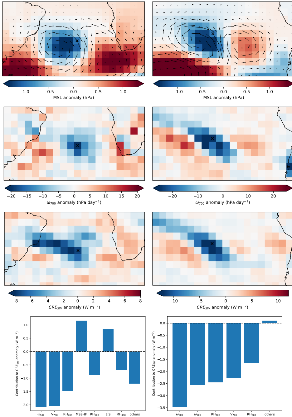
Figure 11. Composite analysis of anomalies in CCFs and CRE_{SW} when V_{700} in the Southeast Atlantic ( topeleft : at 22.527.5^{\circ}S and 12.5^{\circ}W ) and in the South Pacific ( bottomright : at 22.5^{\circ}S and 117.5127.5^{\circ}W ) \rightarrow 2\sigma > 1\sigma . The left-hand From top to bottom, the panels show MSL anomalies and wind anomalies at 700 hPa, the centre panels show \omega_{700} anomalies and the right-hand panels show the , observed CRE_{SW} anomalies, and ridge-regression quantified contributions to the predicted CRE_{SW} anomalies.
