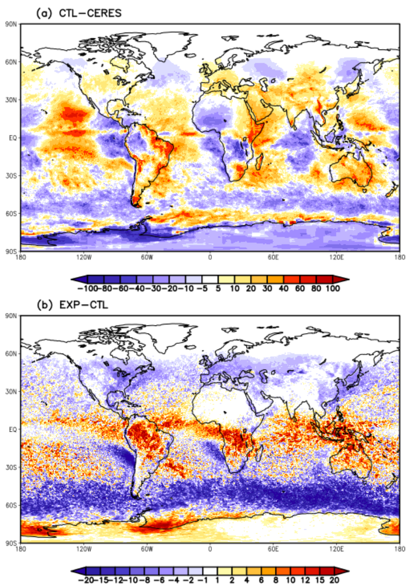
Figure 6. The 120h averaged (a) surface downward shortwave radiation ( \text{W m}^{-2} ) bias from the CTL run against CERES observation, and (b) the difference between the EXP and CTL run (EXP minus CTL).
