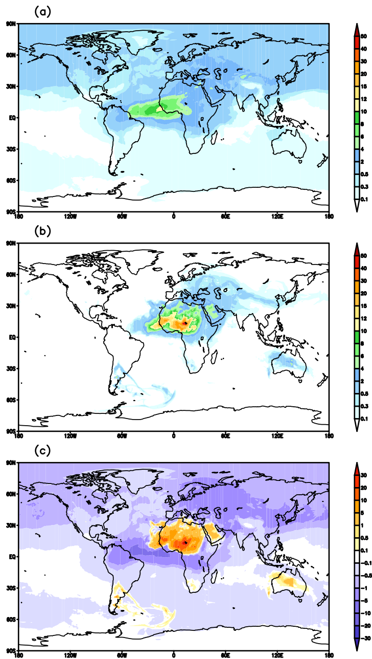
Figure 2. The 120-h forecast IFA number concentration ( 10^{10} \text{ kg}^{-1} ) from (a) CTL, (b) EXP, and (c) EXP minus CTL.
