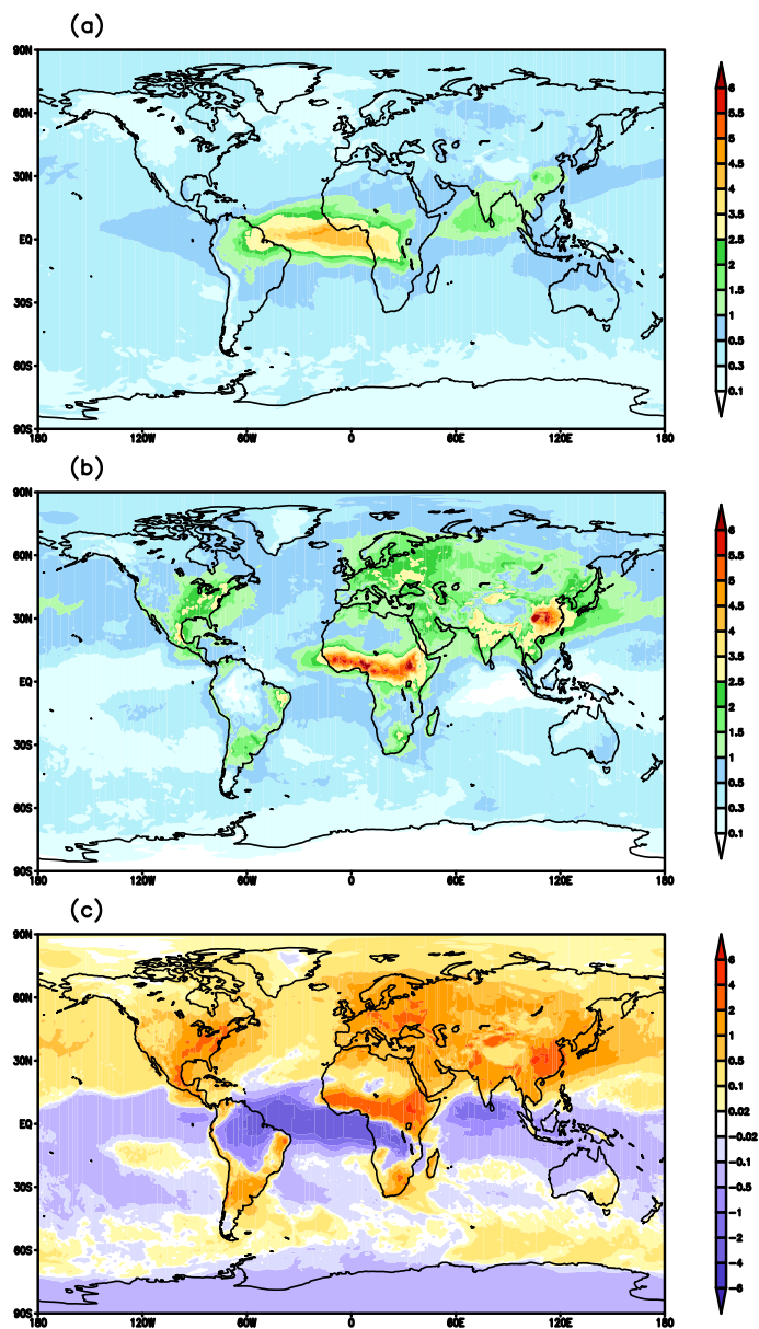
Figure 1. The 120-h forecast WFA number concentration ( 10^{+13} \text{ kg}^{-1} ) from (a) CTL, (b) EXP, and (c) EXP minus CTL.
