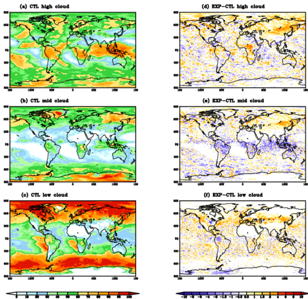
Figure 4. The 120-h averaged (a) high cloud, (b) mid cloud, and (c) low cloud fraction (%) from the CTL run, and the differences of (d) high cloud, (e) mid cloud, (f) low cloud fraction (%) between the EXP and CTL runs (EXP minus CTL).
