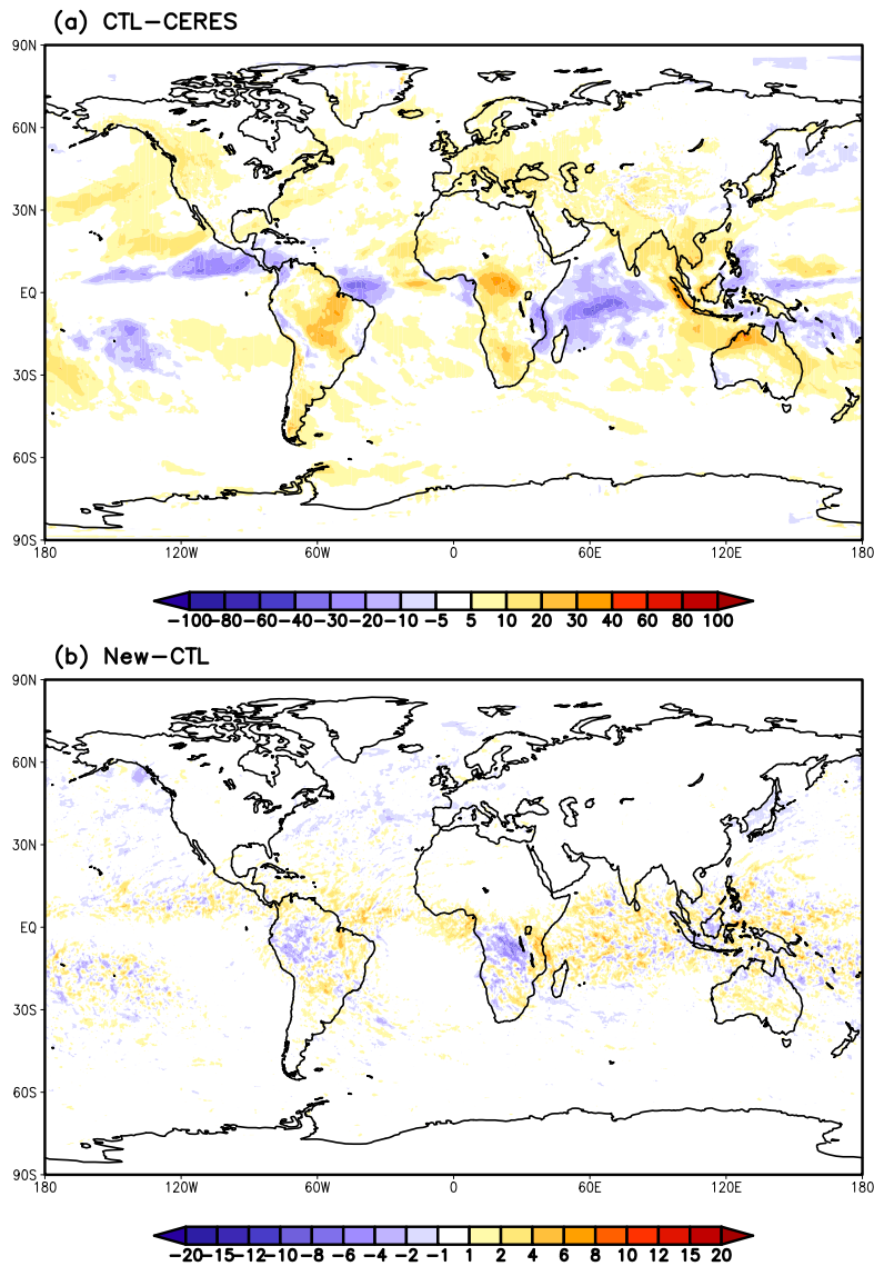
Figure 5. The 120-h averaged (a) OLR ( \text{W m}^{-2} ) bias from the CTL run against CERES observation, and (b) the difference between the EXP and CTL run (EXP minus CTL).
