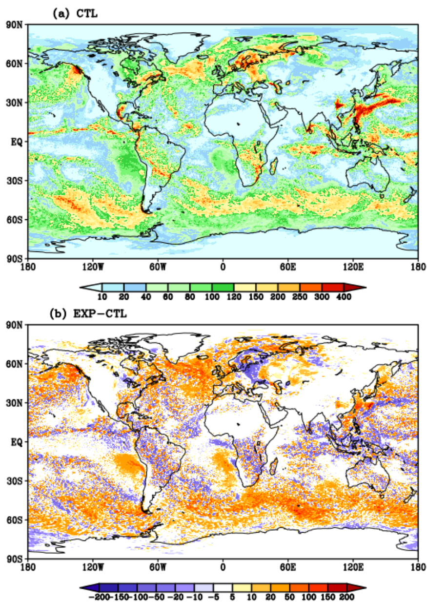
Figure 7. The 120-h forecast liquid water path (LWP, \text{g m}^{-2} ) from (a) CTL run, and (b) the difference between EXP and CTL (EXP minus CTL).
