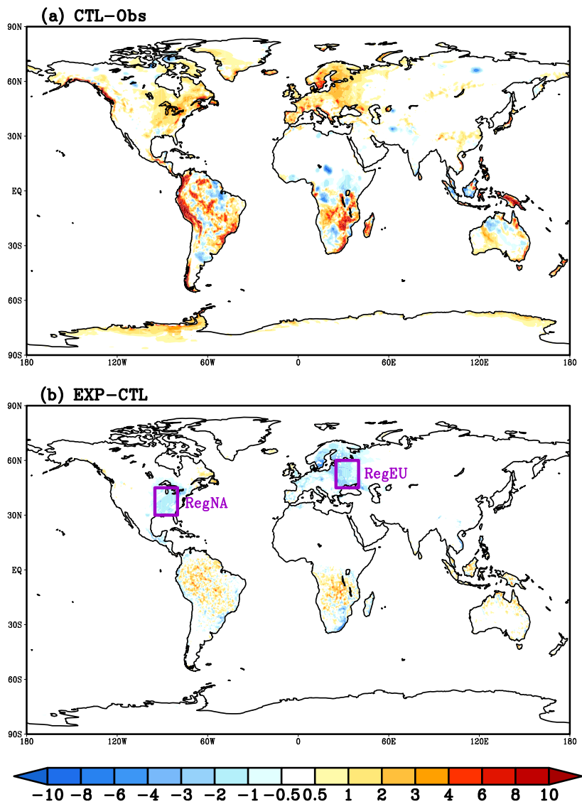
Figure 9. The 120-h averaged (a) total precipitation bias ( \text{mm day}^{-1} ) from the CTL run against CPC rain gauge observation, and (b) the difference ( \text{mm day}^{-1} ) between the EXP and CTL run (EXP minus CTL).
