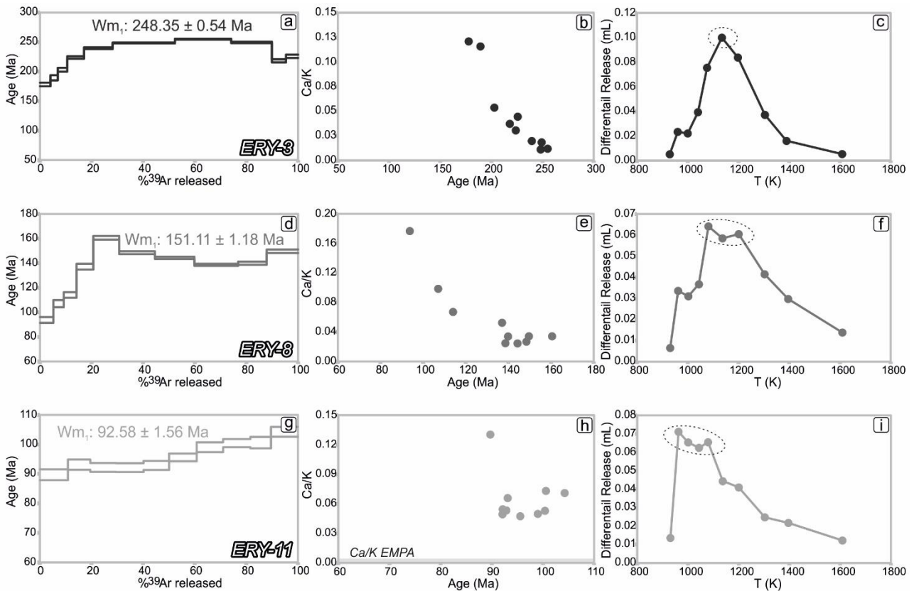
Figure 9: 40 Ar/ 39 Ar age spectra, Ca/K vs. age diagrams and Differential Release Plots for Eyr samples ERY-3 (a–c), ERY-8 (d–f) and ERY-11 (g–i). The dotted circles in the T vs. differential release plots (c, f, i) indicate the degassing steps selected for the age calculation.
