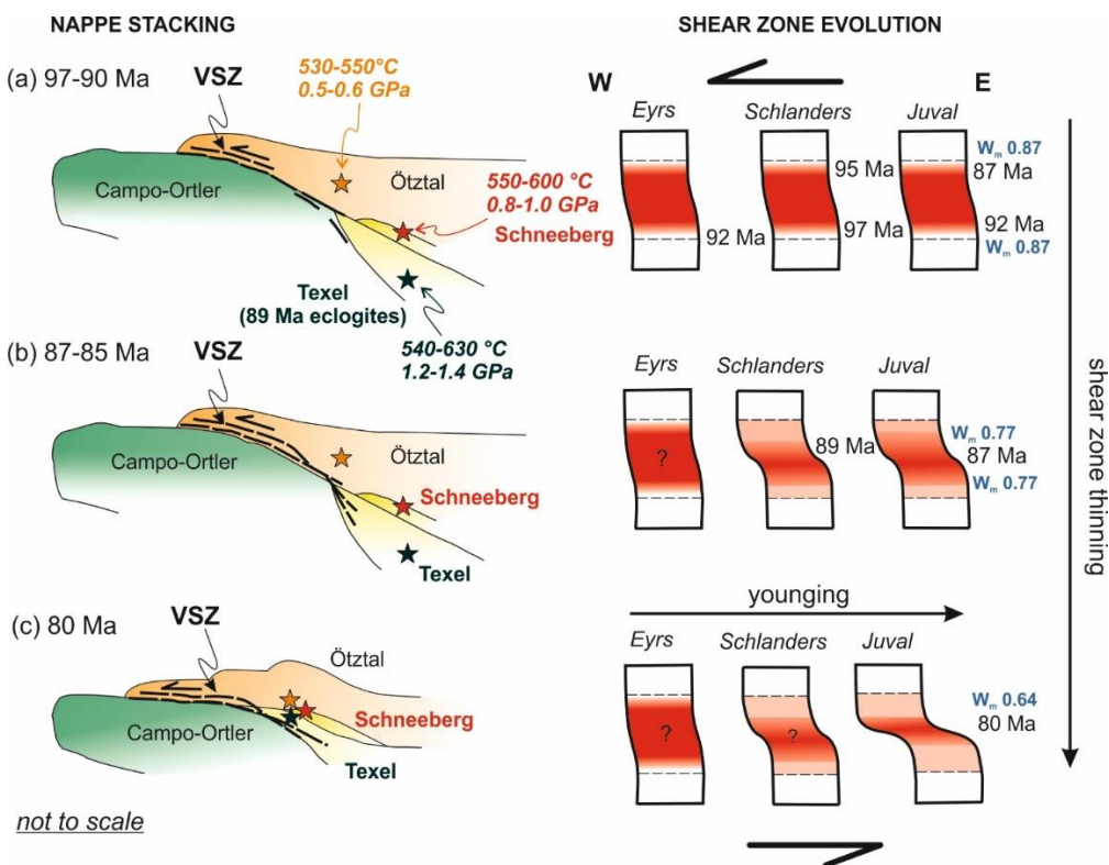
540 Figure 11: Evolution of the Vinschgau Shear Zone in the orogenic Eo-alpine wedge during the Late Cretaceous. Activation of the VSZ (a) in the time span 97-90 Ma affecting the Ötztal unit, (b) in 87-85 Ma the VSZ affected also the Texel unit and (c) during the late stage of shearing exhumed the Texel and Schneeberg units to Ötztal PT conditions. In (a) the PT conditions for Ötztal, Texel and Schneeberg units are reported. The dashed lines represent the thickness and length of the shear zone through time. The evolution of the VSZ in the studied transects in term of ages, finite-cumulative shear strain and kinematic vorticity is also shown.
