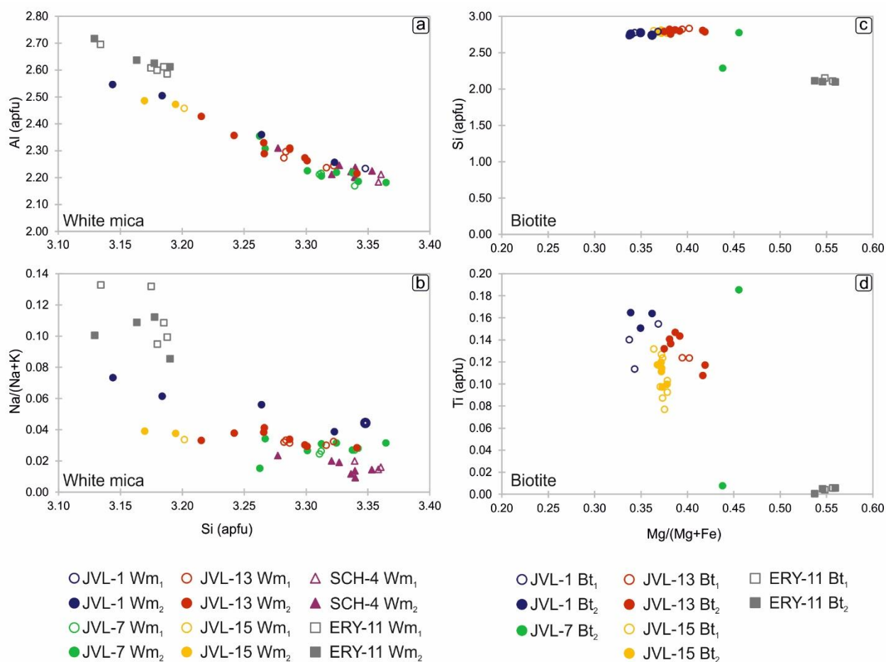
Figure 6: EPMA results showing compositional variation in muscovite-white mica (a-b) and biotite (c-d).
