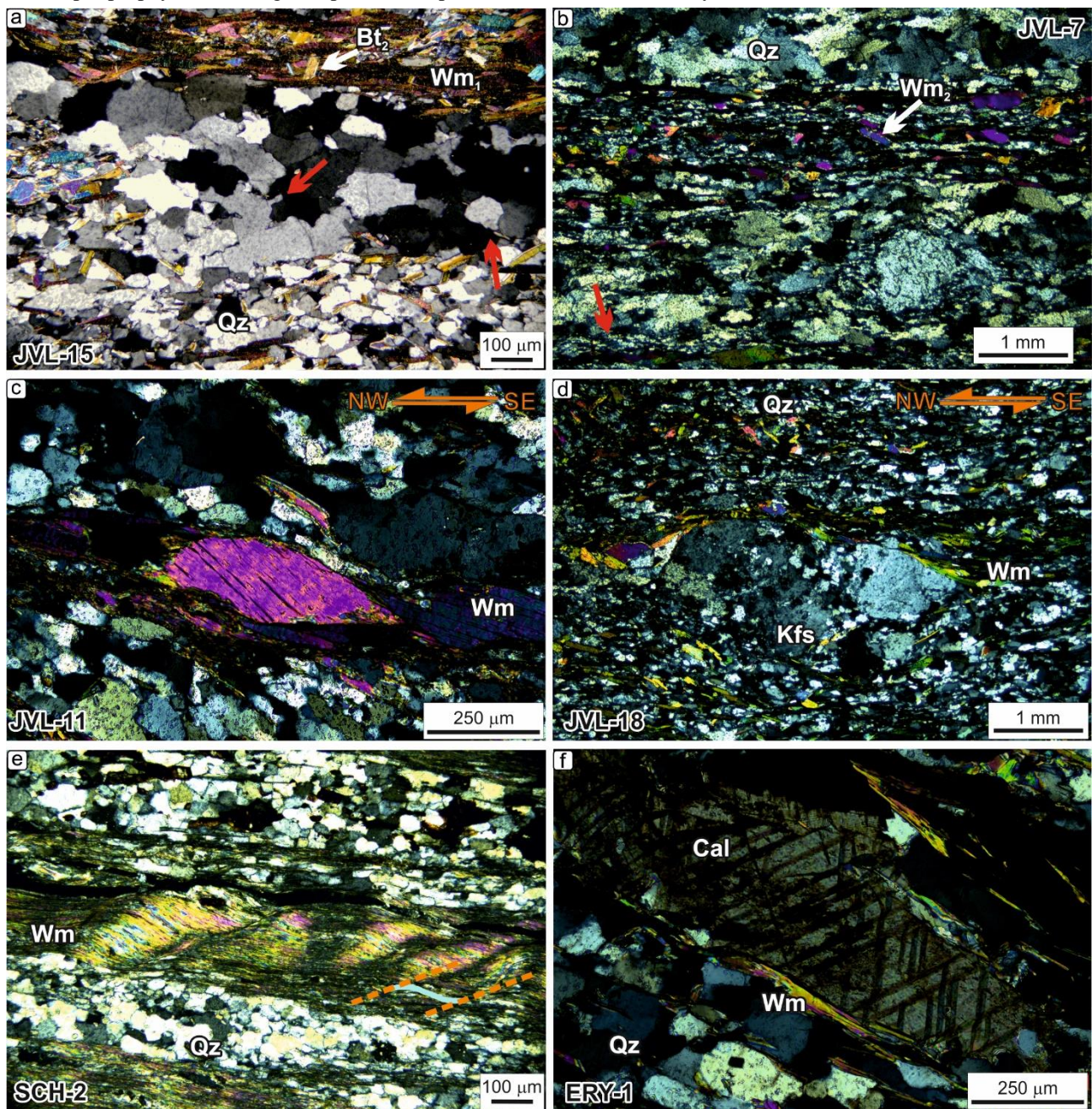
255 Figure 4: Representative photomicrographs from the VSZ, crossed polars. (a) Quartz recrystallized via bulging recrystallization mechanism (red arrows) in poorly deformed Partschinser orthogneiss. The white arrow points at Bt 2 ; (b) 260 Quartz recrystallized via subgrain rotation recrystallization mechanism (red arrows) and static white mica (Wm 2 , white arrow) growing on the main foliation (Wm 1 ) at high angle SCC' fabric together with asymmetric K-feldspar porphyroclasts point to a top-to-W shear sense ; close up on (c) group 5 mica fish according to the classification of Passchier and Trouw (2005) and (d) asymmetric K-feldspar porphyroclasts. (e) A well-developed crenulation cleavage in phyllonite, and (f) deformation twinning in calcite.
