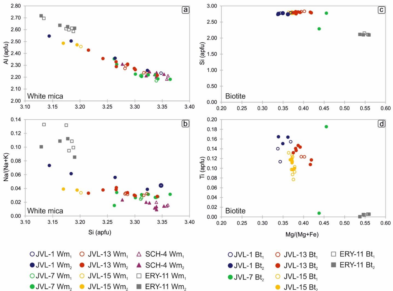
380 Figure 6: EPMA results showing compositional variation in muscovite-white mica (a-b) and biotite (c-d).
