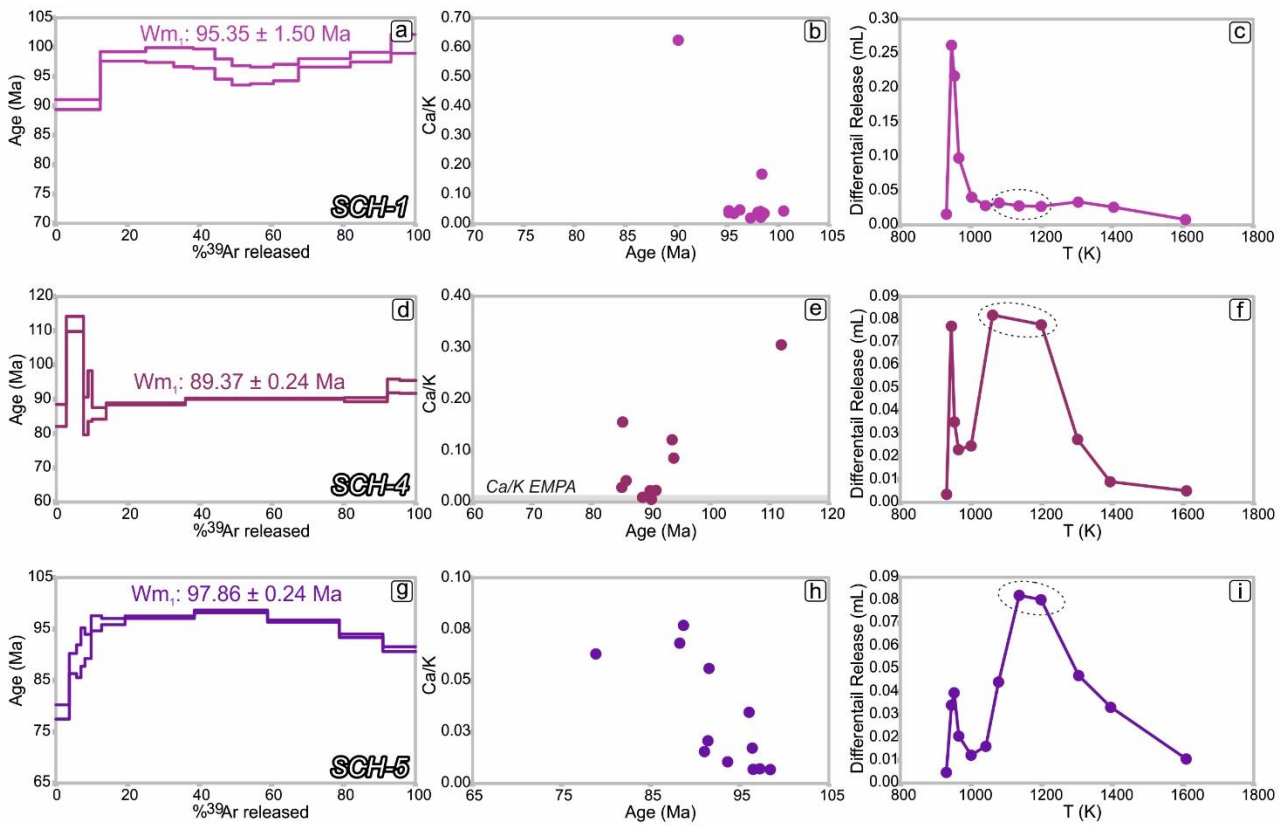
430 Figure 8: ^{40}\text{Ar}/^{39}\text{Ar} age spectra, Ca/K vs. age diagrams and Differential Release Plots for Schlanders samples SCH-1 (a–c), SCH-4 (d–f) and SCH-5 (g–i). The dotted circles in the T vs. differential release plots (c, f, i) indicate the degassing steps selected for the age calculation.
