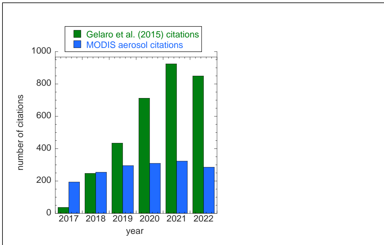
Figure 1. Number of citations received by Gelaro et al. (2015), the fundamental reference for the NASA MERRA2 assimilation system products (green) and the combination of citations received by Levy et al. (2013) and Hsu et al. (2013) representing the Dark Target and Deep Blue aerosol algorithm products for MODIS (blue). Source: Clarivate Web of Science data base. The point is to note the rapid acceleration of MERRA2 citations as an indicator of the speed of the research community's acceptance of assimilation products, while traditional retrieval products such as MODIS aerosol products maintain a consistent presence in the research community. We anticipate that over the next twenty years, assimilation product use will continue to grow while use of standard products will plateau and decrease.
