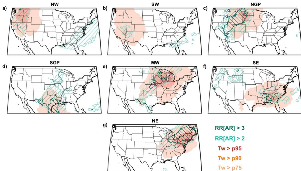
Figure 3: AR/humid-heat interaction maps
