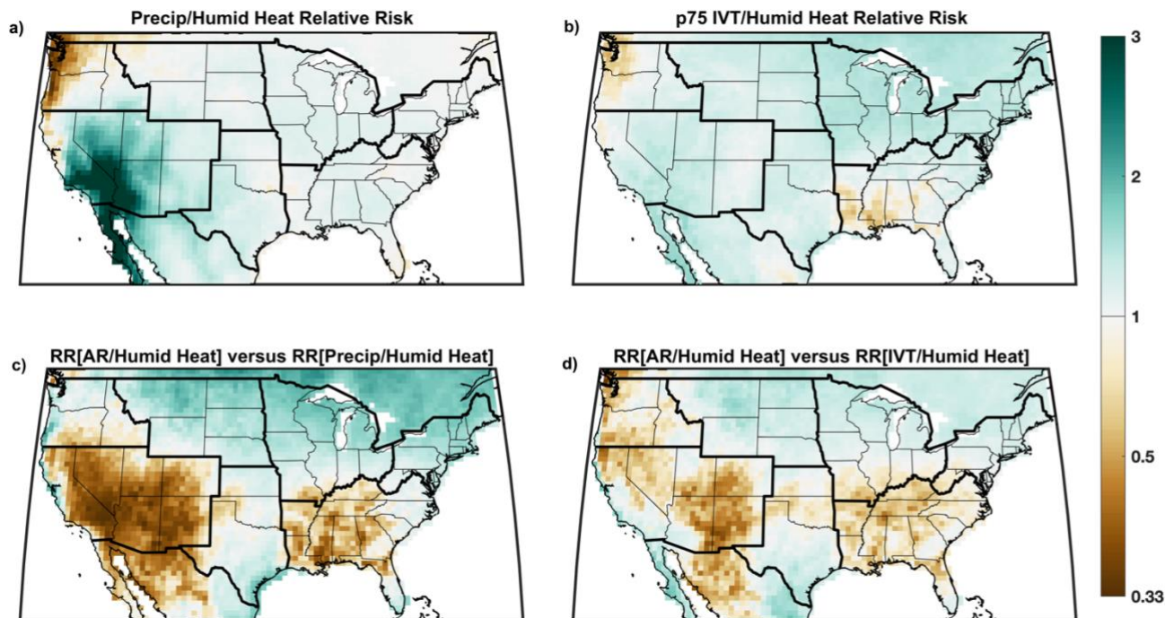
Figure 4: Relative risk of humid heat conditioned on precipitation and extreme IVT
