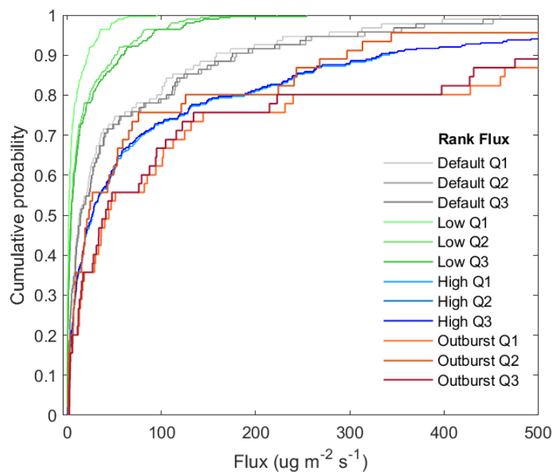
50 Figure 6: CDFs of emissions as a function of different rank ug\ m^{-2}\ s^{-1} . Rank and Q_i ( j=1, 2, 3 ), which are respectively defined and described in Sections 2.2 and Sect. 2.4.
