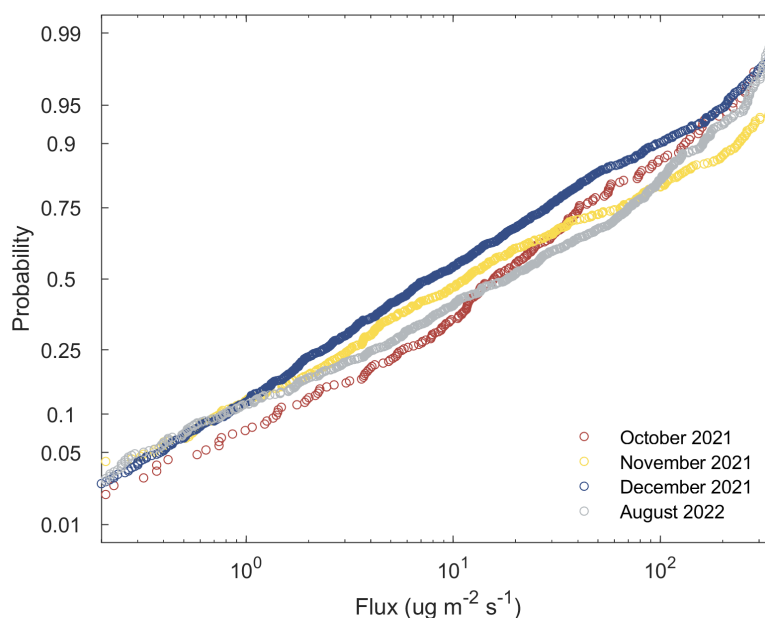
05 Figure 4: Cumulative probability distribution of 30-minute Eddy Covariance flux measurements ug m -2 s -1 , where: (red) is October 2021, (yellow) is November 2021, (blue) is December 2021, and (grey) is August 2022. All observations are included in this plot.
