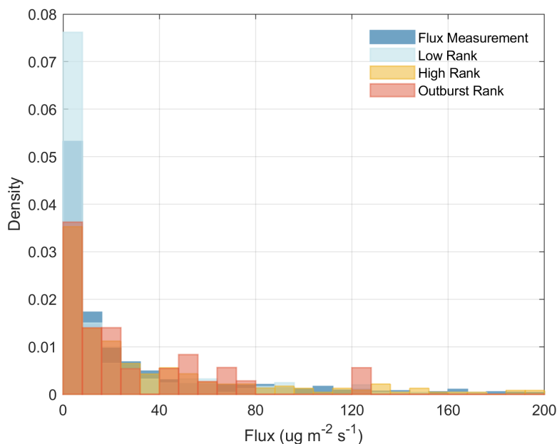
Figure 7: PDF of all calculated emissions fluxes across all mines, separated rank-by-rank in units of \text{ug m}^{-2} \text{s}^{-1} where: (light blue) is low rank, (yellow) is high rank, and (red) is outburst rank. PDF of flux observations less than 200 \text{ ug m}^{-2} \text{s}^{-1} are given in (dark blue).
