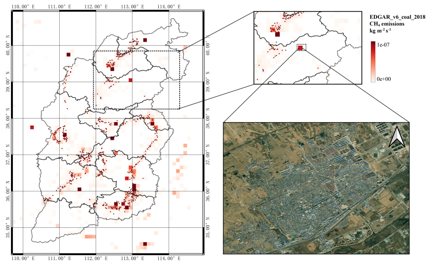
25 Figure 9: The mapped annual average emissions from EDGAR are overlapped with the locations of the mines used in this work. Note that the region located inside of the black dashed box is shown in more detail on the top right as an EDGAR CH 4 emissions hotspot. However, there are no actual coal mines anywhere in the box. This is supported by the RGB image (from ESRI) of the actual location, which shows a residential area.
