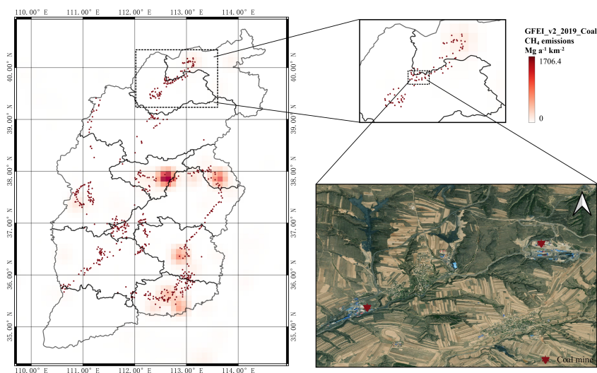
50 Figure 10: The mapped annual average emissions from GFEI are overlapped with the locations of the mines used in this work. Note that the region located inside of the black dashed box is shown in more detail on the top right as a region with almost zero emissions by GFEI \text{CH}_4 emissions. However, there actual location contains multiple coal mines. For ease of viewing, only 2 of the 25 coal mines are shown on the map (from ESRI).
