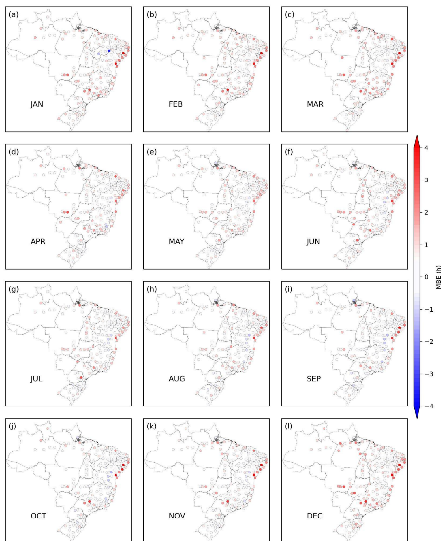
Figure 1: Spatial distribution of monthly MBE (h) between daily CMSAF's SDU estimates and in situ data for the period of 2013-2017.
