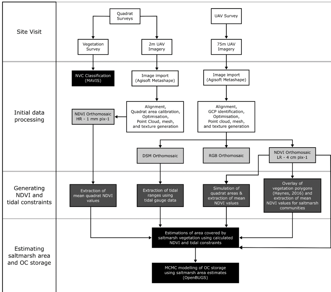
185 Figure 2: Workflow schematic for this study. Light grey colouring represents initial map outputs. Dark grey colouring represents points where key data were extracted for use in additional analyses. Black colouring represents final data outputs.
