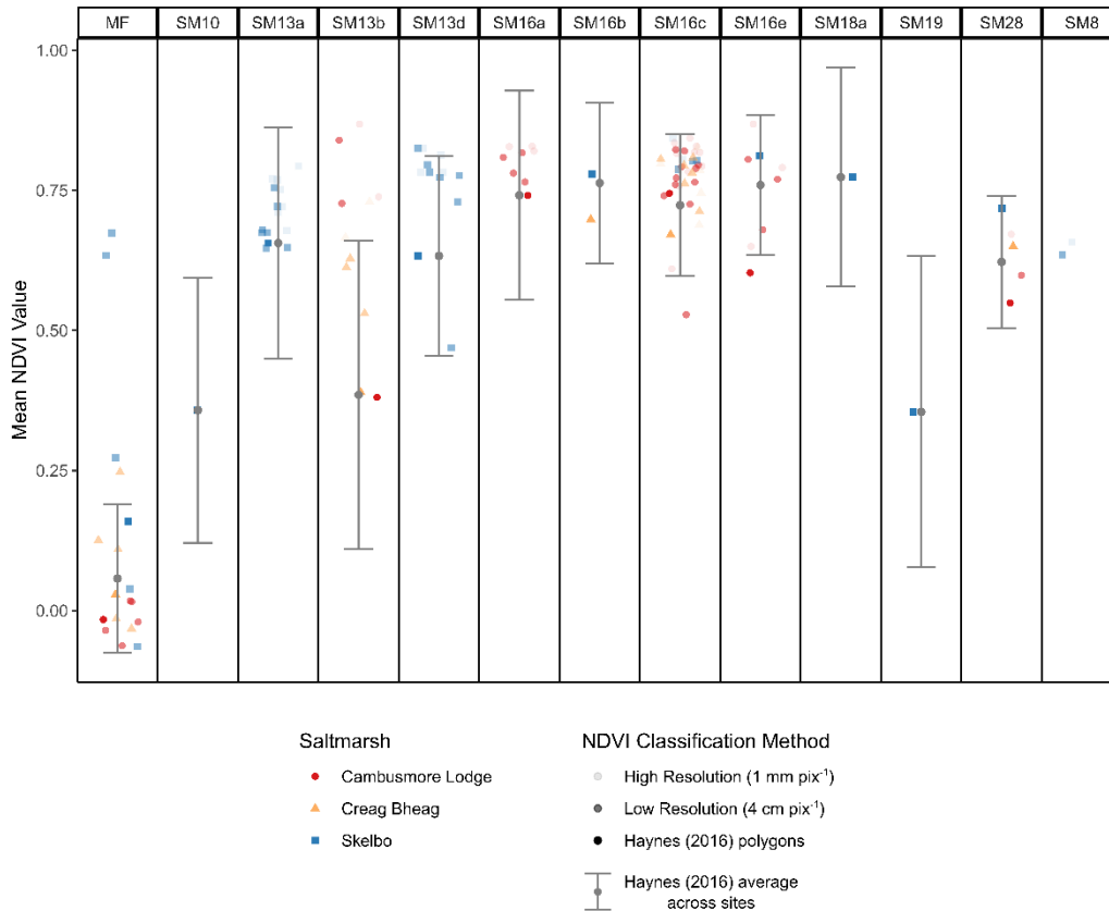
330 Figure 5: NDVI values extracted from our quadrats and extracted from polygons from the existing 2011 survey (Haynes, 2016). Where in the 2011 survey the same saltmarsh community is present at multiple sites, these data have been combined and the mean and 1SD range is shown with the grey point and error bar. MF = Mudflat
