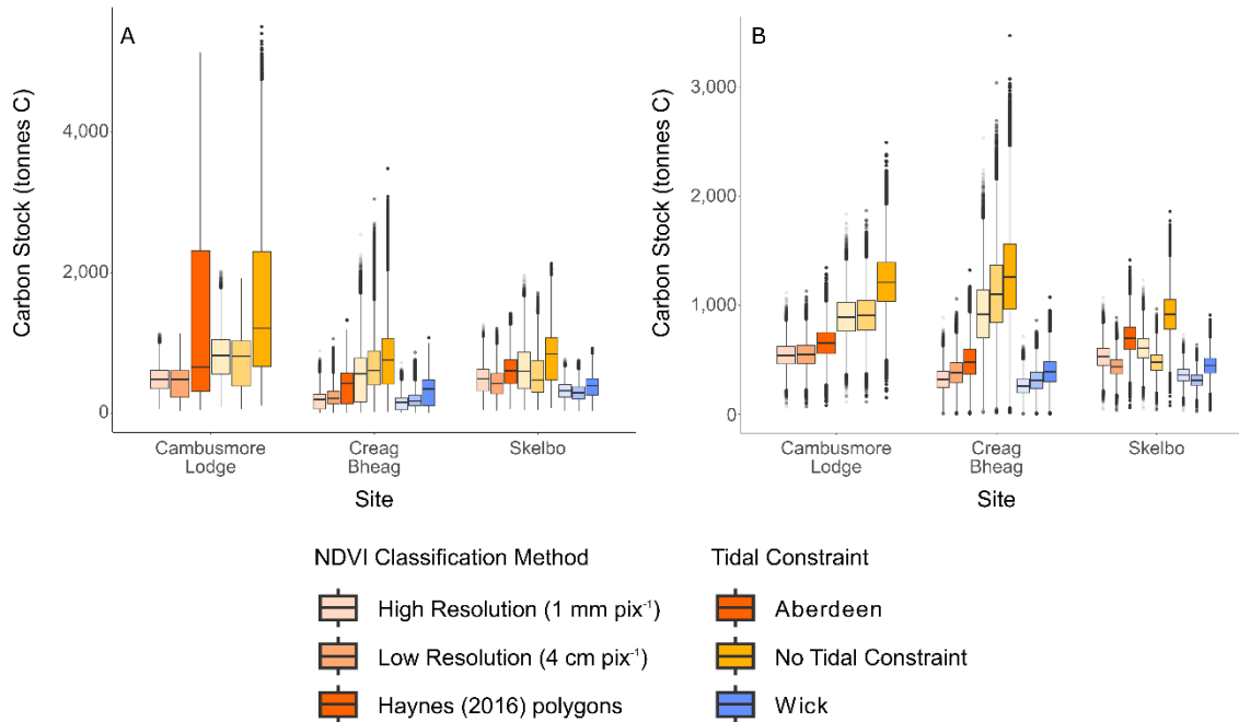
395 Figure 7: Estimates of OC stocks generated from the MCMC OC models. A) Data include all range estimates (Mean, 1SD, and 2SD NDVI ranges); B) Data for the 1SD range only.
