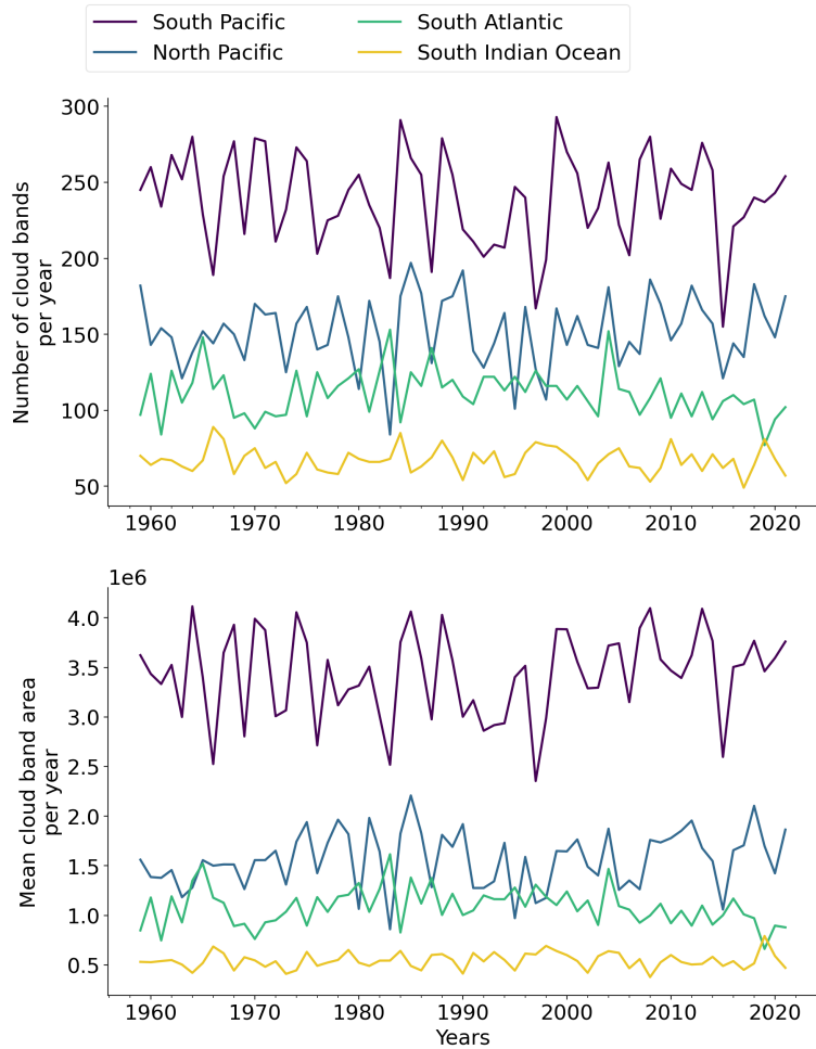
Figure 8. Time series of a) the number of cloud bands per day-year for each domain defined in Figure 2, and b) of the mean cloud band area per year (expressed in \text{km}^2 ) .
