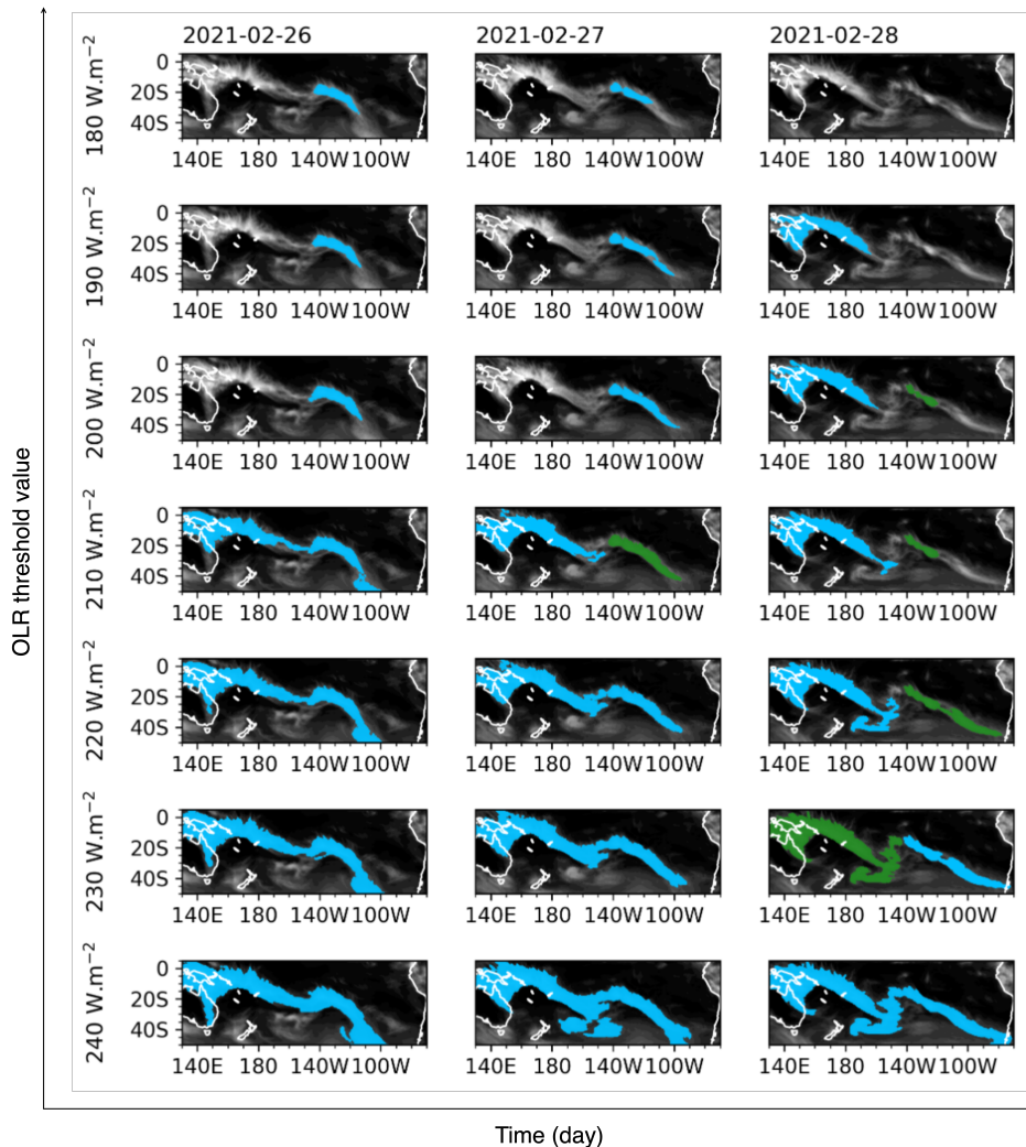
Figure B1. Sensitivity test case illustrating the detection of cloud bands in relation to the OLR threshold, ranging from 180 to 240 \text{W.m}^{-2} with an interval of 10 \text{W.m}^{-2} , from February 26 to 28, 2021, in the South Pacific.
