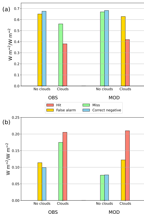
Figure 13. (a) Mean annual transmittance for each case in the model and in the observations during the year 2020 and (b) standard deviation of transmittance for each case in the model and in the observations during the year 2020. Transmittance is the SWD normalized by the SWD at the top of the atmosphere.
