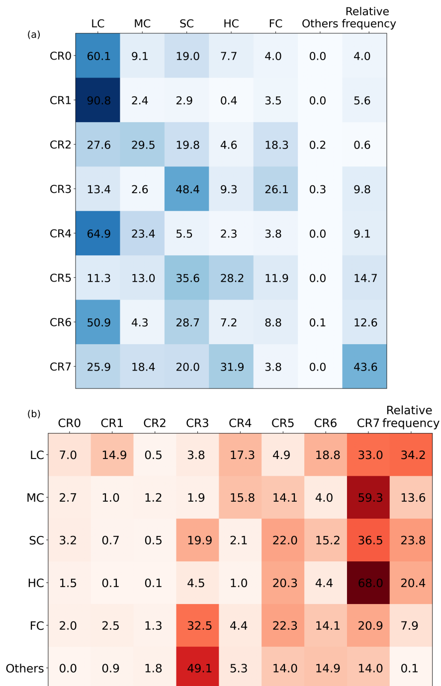
Figure 14. Cross-comparison of cloud regime/cloud type (in %) in hit cases. (a) For each CR, the relative frequency of each CT. The last column is the relative frequency of each CR for all hits in overcast situations. The sum of each row is equal to 1. (b) For each CT, the relative frequency for each CR. The last column is the relative frequency of each CT over all hits in overcast situations. The sum of each row is equal to 1.
