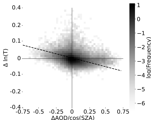
Figure 6. \ln(\text{Transmittance (SWD/SWD}_{TOA})) errors as a function of AOD errors with the fit line during clear skies in year 2020 when the SZA is less than 70^\circ
