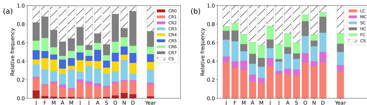
Figure 3. Monthly relative frequency for each (a) cloud regime in AROME and clear skies (CS), (b) cloud type in the satellite images and clear skies (CS), over 2020 for the pixels including the pyranometers.
