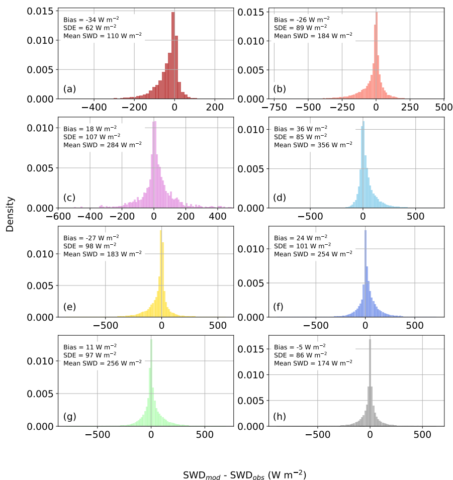
Figure 12. Distribution of SWD errors (bias and SDE indicated) for (a) CR0, (b) CR1, (c) CR2, (d) CR3, (e) CR4, (f) CR5, (g) CR6, (h) CR7 cloud regimes in overcast situations.
