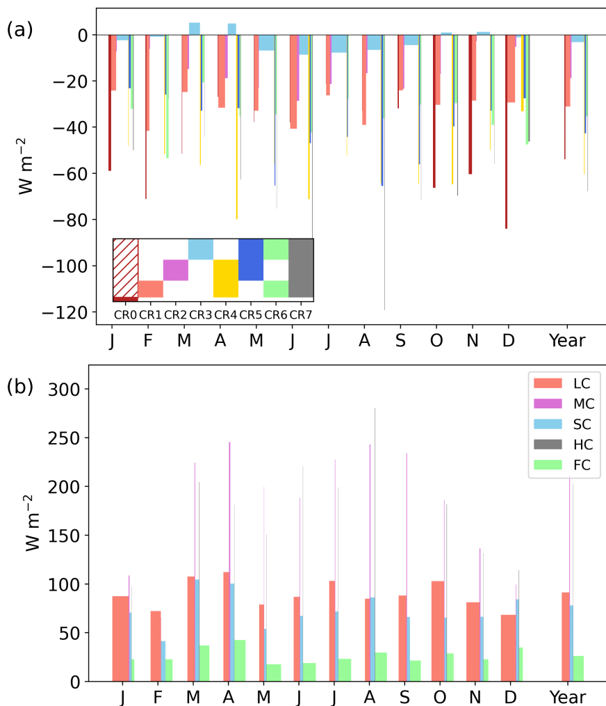
Figure 7. Monthly relative bias (bar height) and frequency (bar width) for (a) each cloud regime for the false alarm cases, (b) each cloud type for the miss cases. The vignette of the cloud regimes is inserted to facilitate the reading.
