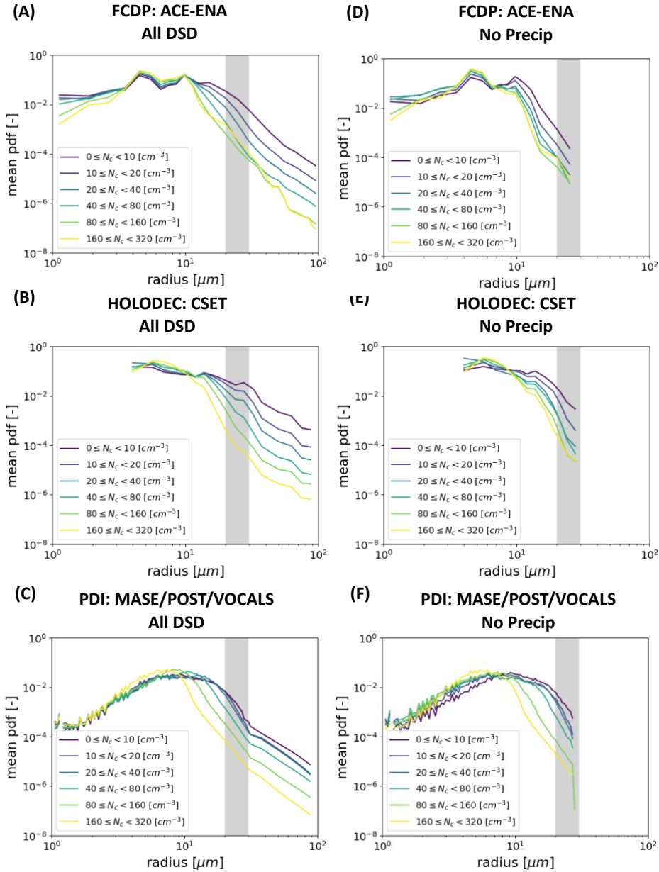
210 Figure 3: The mean probability density function (pdf) of the drop concentration sorted by the cloud mode drop number concentration for the three datasets. Panels A-C show results for all DSDs and panels D-F shows results filtered for DSDs with no precipitation water. The parameter k is calculated using only the cloud-sized drops even when precipitation is present in the DSD. The grey bar shows a notional range of radius 20-30 \mu\text{m} separating cloud from precipitation sized drops.
