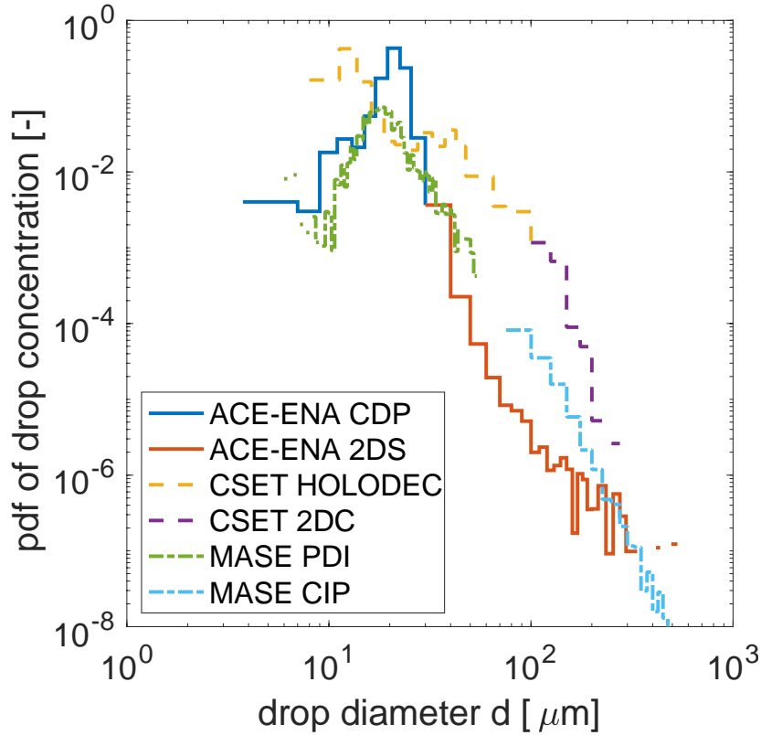
125 Figure 1: An example of merged drop size distributions from each campaign.
