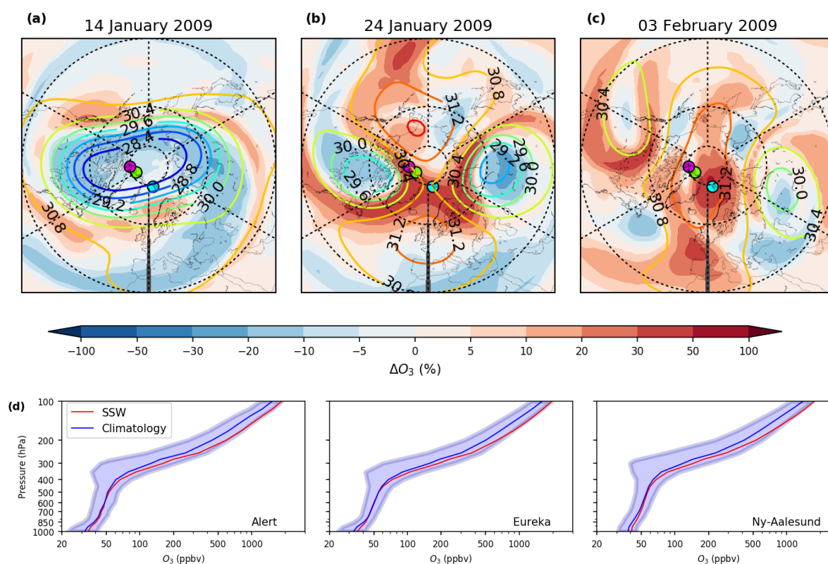
915 Figure 1: 10 hPa geopotential height (km) (contours) and deseasonalised ozone percentage anomalies (shading) over the Northern Hemisphere for (a) 10 days before, (b) the SSW central warming date and (c) 10 days after a split vortex, PJO-type SSW event (January 2009) from the CAMS atmospheric composition reanalysis. Ozone anomalies are calculated with respect to the 2005–2013 baseline period. Contour intervals are 0.4 km. (d) Ozone-sonde (100–1000 hPa) climatology (November–May) and SSW composite profiles for three long-running Arctic sites: Alert (green circle), Eureka (violet circle) and Ny-Ålesund (cyan circle) as marked on each map in (a–c). Mean SSW profiles were composited from all profiles within -20 to +70 days of an SSW central warming date with all remaining profiles used in compositing a mean climatology profile during the stratosphere dynamically active season (November–May). Blue shaded region represents 1 \sigma around the climatological mean. The climatology is constructed excluding SSW events in each case. 920
