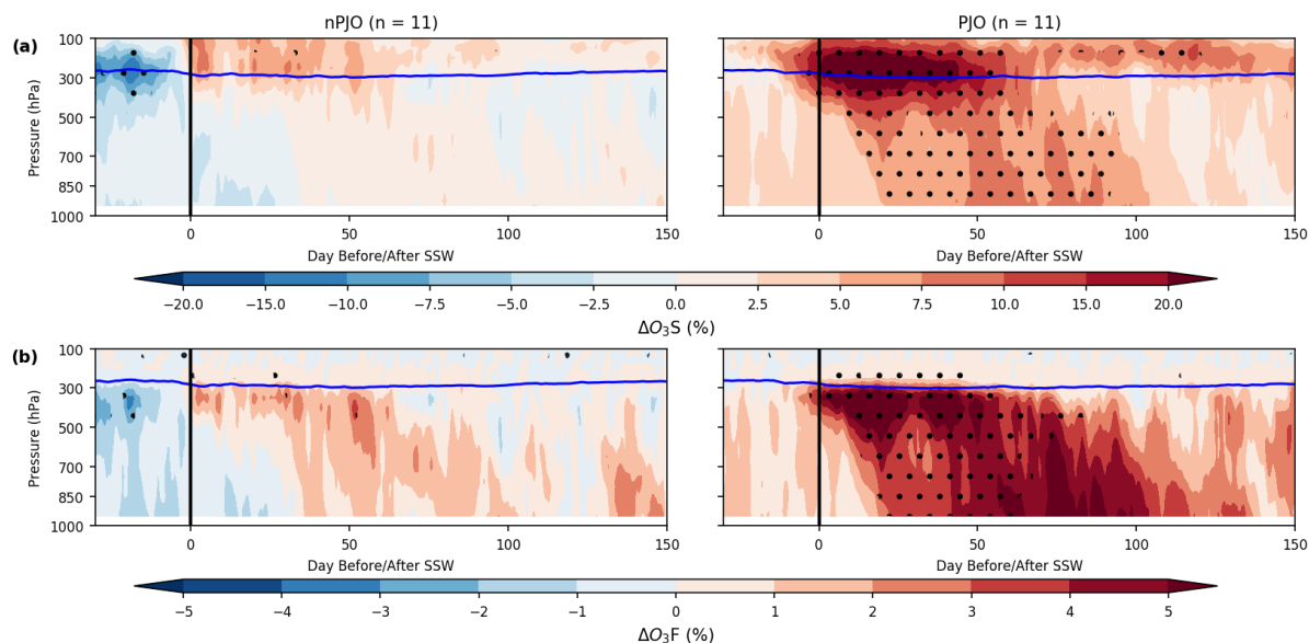
Figure 5: As Fig. 4 but for (a) ozone of stratospheric origin (O 3 S) and (b) the fraction of ozone of stratospheric origin (O 3 F = O 3 S/O 3 × 100) deseasonalised anomalies (%) evolution for nPJO-type SSWs ( n = 11 ) and PJO-type SSWs (1980-2013) from EMAC for the time period 1980–2013.
