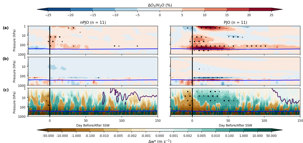
Figure 4: Vertical-time composites of polar-cap (60–90° N) averaged (a) ozone (O 3 ), (b) water vapour (H 2 O) and (c) residual vertical velocity ( \bar{w}^* ) deseasonalised anomalies (%) for nPJO-type and PJO-type SSWs (each of which with n = 11 events) from EMAC for the time period 1980–2013. The anomalies are expressed as percentages, with the exception of the residual vertical velocity ( \bar{w}^* ) anomalies which are given in units of \text{m s}^{-1} (zero contour represented by purple solid line). Statistical significance at the 95 % level is indicated by stippling. The World Meteorological Organization (WMO) defined thermal tropopause is displayed for reference in each panel (blue solid line).
