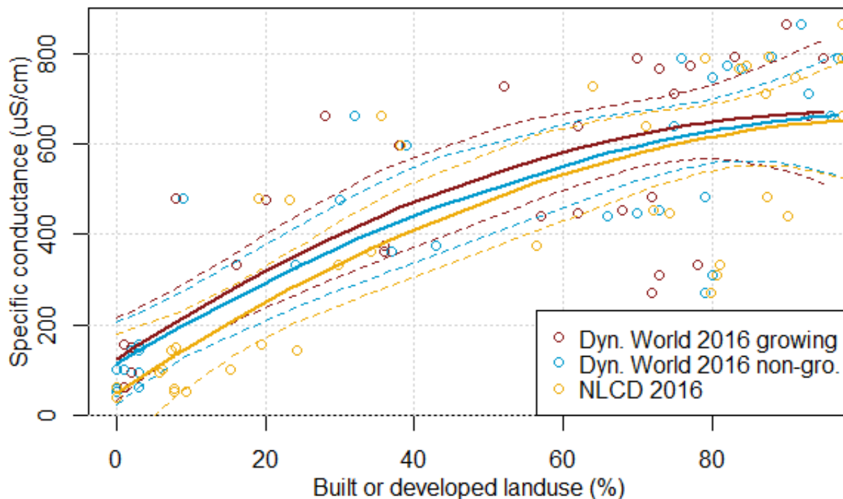
230 Figure 4: Modeled median specific conductance (SC) for 37 watersheds comparing Dynamic World 2016 growing and non-growing season built and NLCD 2016 developed LULC, with 95% confidence intervals as dashed lines.
