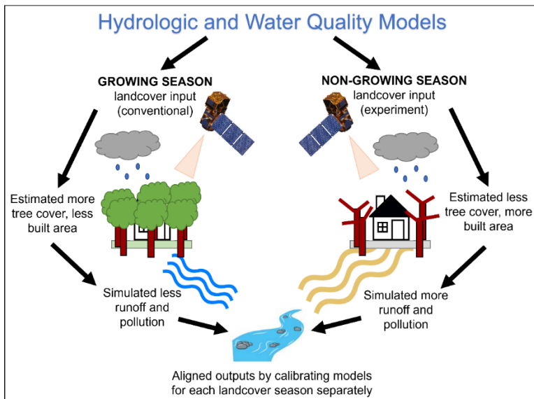
365 Figure 8: Conceptual diagram of the conclusions of the study in temperate watersheds of the eastern United States.
