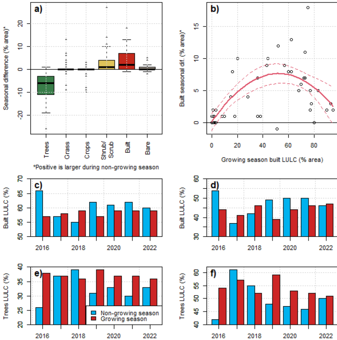
180 Figure 3: All using Dynamic World 2016: a) Difference between growing and non-growing season LULC for 55 watersheds (classes of water, flooded vegetation, barren, and snow/ice were approximately 1% of watershed area so omitted; boxplots show median, interquartile range (IQR), b) Quadratic relationship between built area and the seasonal difference in built area for 55
