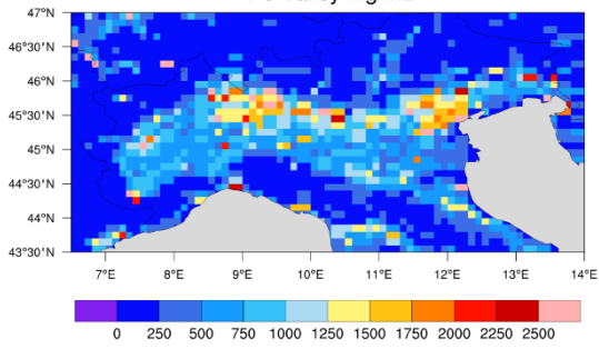
PM25 total emissions EDGAR Po Valley mg/m2
