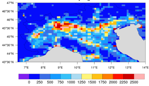
PM25 total emissions CAMS221 Po Valley mg/m2
