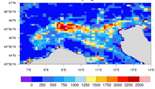
PM25 total emissions CAMS42C Po Valley mg/m2
