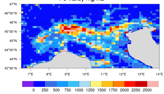
PM25 total emissions EMEP-GNFR Po Valley mg/m2
