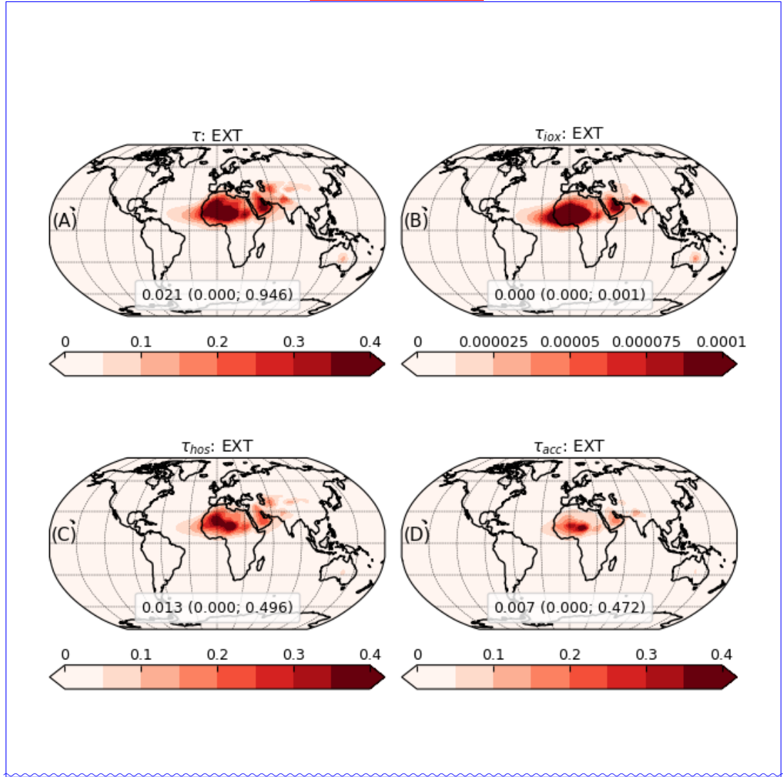
Figure 10. Annual mean dust optical depth ( \tau ) from the mineral experiment with external mixing configuration (EXT; A), decomposed into free iron oxides ( iox ; B), host amalgam ( hos ; C) and static accretion ( acc ; D). The optical depth is averaged over the spectral band of ModelE2.1 covering ultra-violet and visible wavelengths ( 0.30 - 0.77 \mu\text{m} ). The extremes of the color bars are set to include 1 st and 99 th percentiles of the mapped variables. Global average along with minimum and maximum (within parentheses) are also reported.
