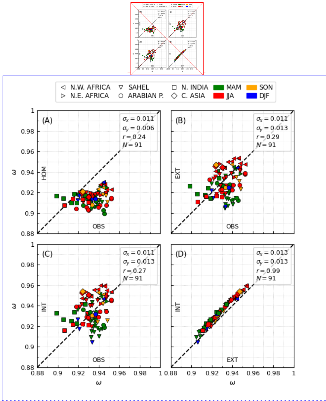
Figure 12. Monthly Climatological monthly mean single scattering albedo ( \omega ) from model experiments compared to AERONET monthly retrievals at the selected stations and months from the AeroTAU4 data set , labeled by region (Figure 5) and season (Northern Hemisphere spring: MAM, summer: JJA, autumn: SON, winter: DJF). The single scattering albedo is averaged over the spectral band of ModelE2.1 covering ultra-violet and visible wavelengths ( 0.30 - 0.77 \mu\text{m} ). AERONET monthly means (OBS) are separately compared to the control run with homogeneous composition (HOM; A), and the mineral experiments with external (EXT; B) and internal (INT; C) mixing configuration; the two mineral experiments are also directly compared (D). Standard deviation of the monthly means ( \sigma ), Pearson correlation coefficient ( r ) and number of monthly values ( N ) are also reported.
