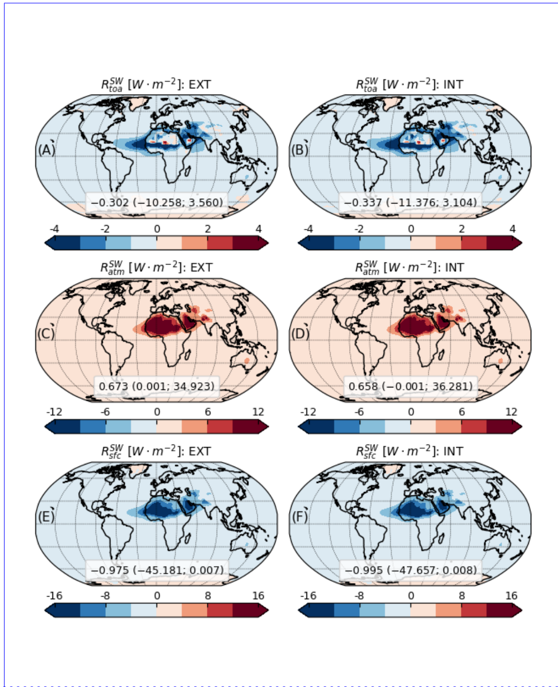
Figure S1. Annual mean direct radiative effect at the top of atmosphere ( R_{toa}^{SW} ), in the atmosphere ( R_{atm}^{SW} ) and at surface ( R_{sfc}^{SW} ), from the mineral experiments with external (EXT; A, C and E, respectively) and internal (INT; B, D and F, respectively) mixing configuration. The direct radiative effect is relative to the entire shortwave spectrum (0.30 – 4 \mu m ). The extremes of the color bars are set to include 1 st and 99 th percentiles of the mapped variables. Global average along with minimum and maximum (within parentheses) are also reported.
