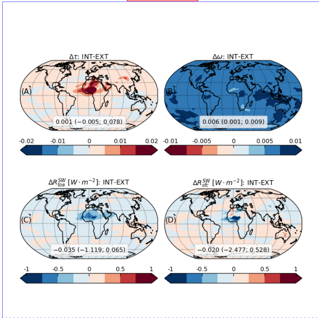
Figure 11. Same as Figure 6 but showing the contrast between the mineral experiments with internal (INT) and external (EXT) mixing configuration. Note that the color mapping for single scattering albedo (panel B) indicates positive variations (i.e. increased /decreased scattering) with blue/red, and vice versa.
