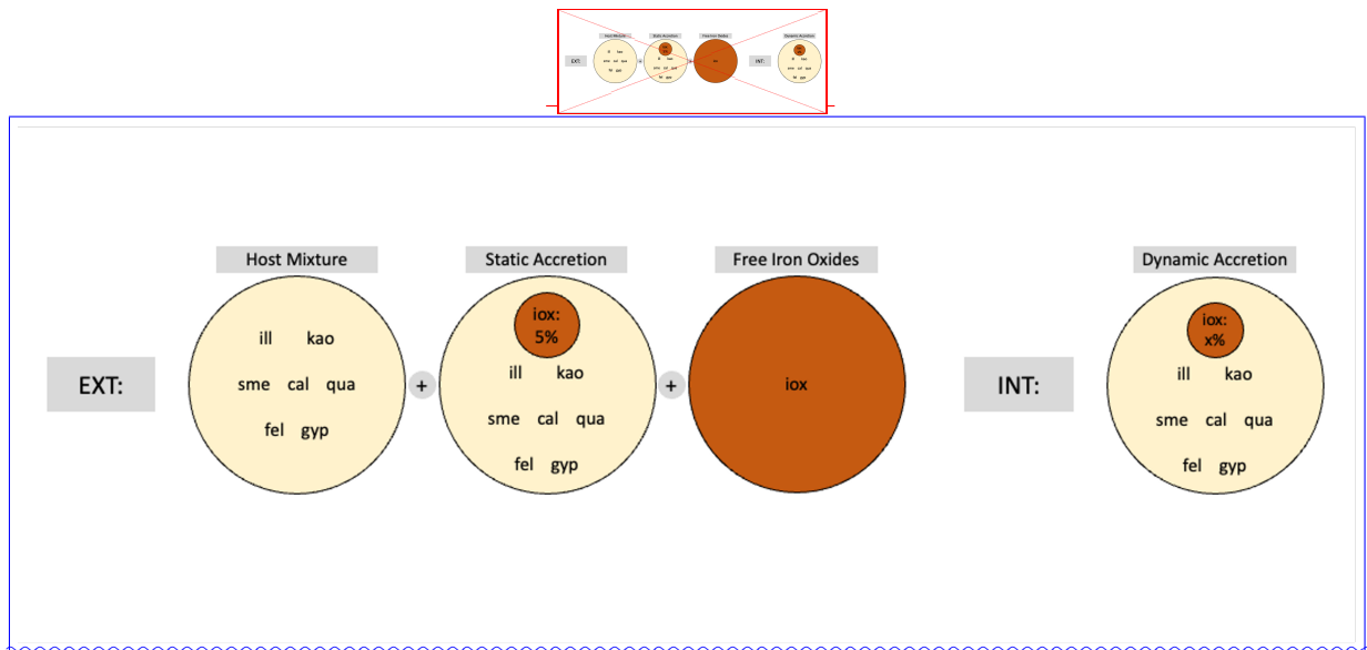
Figure 1. Schematic cartoon of the mixing state of minerals, assumed for optical-radiative calculations, in the coupling schemes with external (EXT) and internal (INT) mixing configuration. The EXT scheme assumes external mixing of three mineral components, whose size-resolved proportions vary in space and time: 1) a homogeneous amalgam of non iron-oxide minerals (host mixture), 2) a two-component mixture of the host amalgam and a fixed 5% mass fraction of iron oxides (static accretion), and 3) free iron oxides. In the INT scheme, the fifteen mineral tracers are re-arranged to form a single size-resolved internal mixture of the host amalgam with a mass fraction of iron oxides that varies at each grid box and time step (indicated as x\% ). The acronyms for minerals indicate: illite ('ill'), kaolinite ('kao'), smectite ('sme'), calcite ('cal'), quartz ('qua'), feldspar ('fel'), gypsum ('gyp') and iron oxides ('iox').
