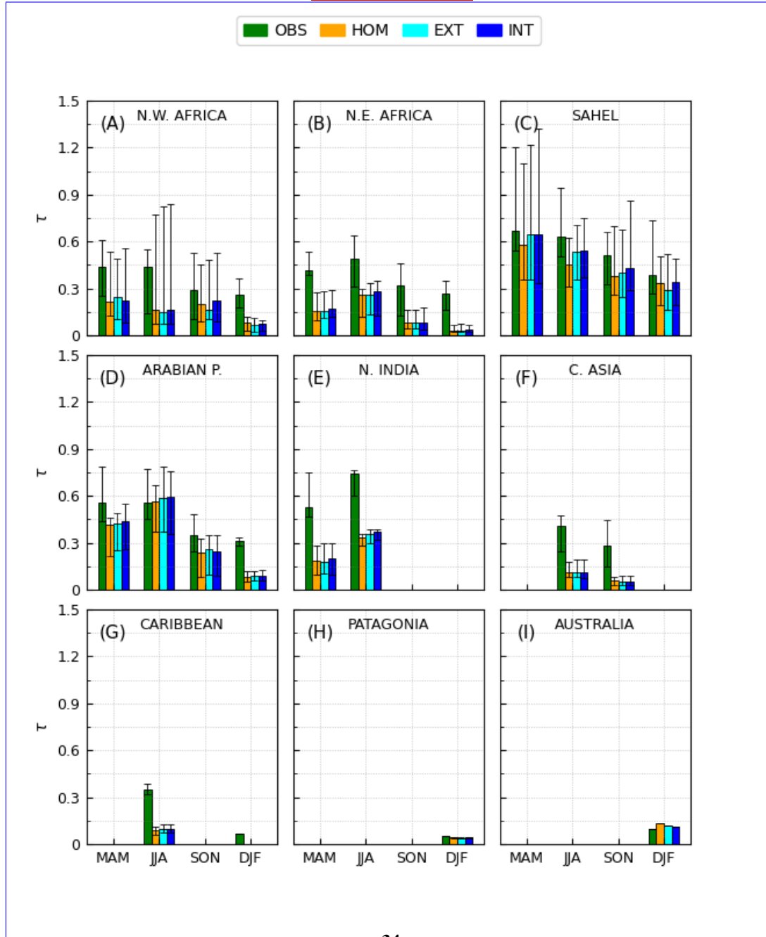
Figure 14. Same as Figure 13 but showing the comparison between model and AERONET dust optical depth ( \tau ), at the selected stations and months from the AeroTAU0 data set.
