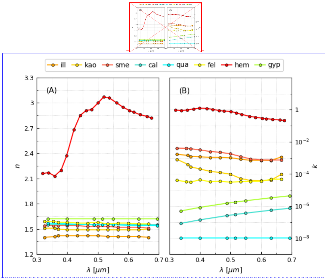
Figure 2. Real ( n ; A) and imaginary ( k ; B) indices of single minerals at visible wavelengths ( \lambda ) as collected by Scanza et al. (2015): illite ('ill'), kaolinite ('kao'), smectite ('sme'), calcite ('cal'), quartz ('qua'), feldspar ('fel'), hematite ('hem') and gypsum ('gyp').
