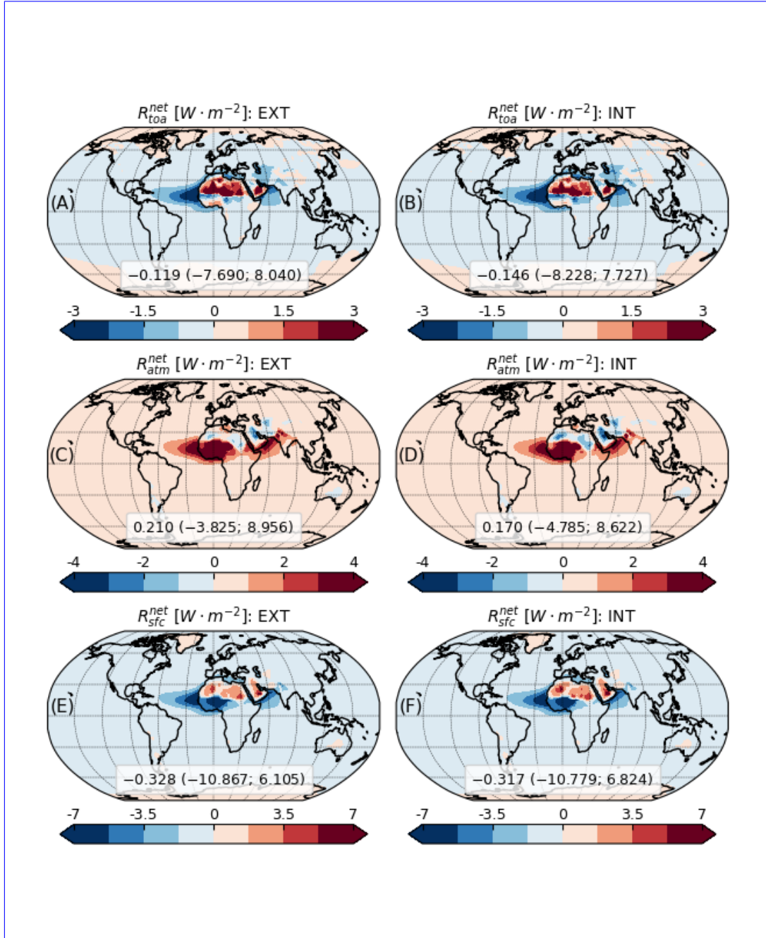
Figure S3. Same as Figure ??-S1 but showing the net direct radiative effect (sum of shortwave and longwave contributions): R_{toa}^{net} , R_{atm}^{net} and R_{sfc}^{net} , at the top of atmosphere, in the atmosphere and at surface, respectively), calculated as the sum of shortwave and longwave contributions.
