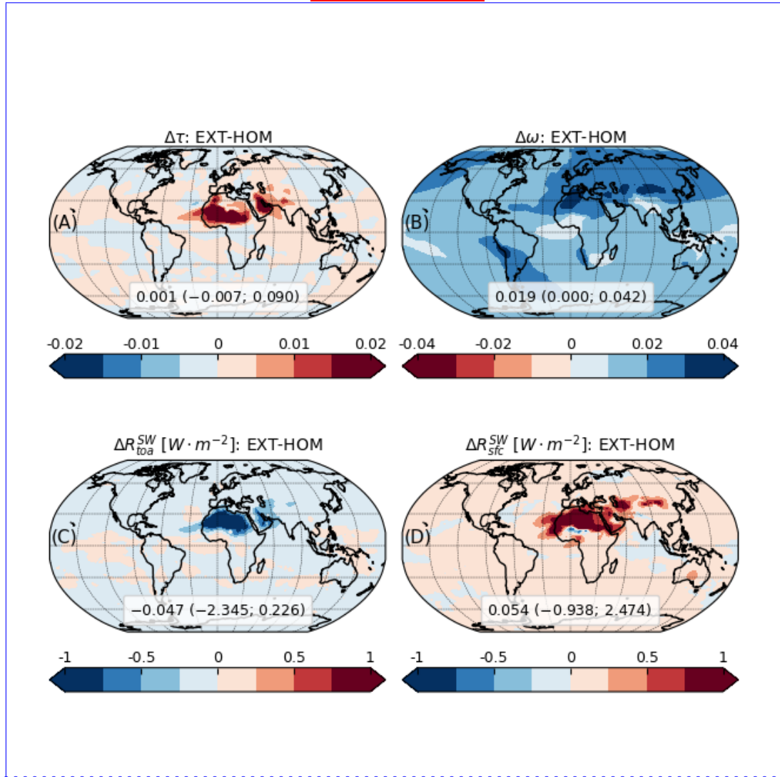
Figure 8. Same as Figure 6 but showing the contrast between the mineral experiment with external mixing configuration (EXT) and the control run with homogeneous composition (HOM). Note that the color mapping for single scattering albedo ( panel B ) indicates positive variations (i.e. increased /decreased-scattering) with blue/red, and vice versa.
