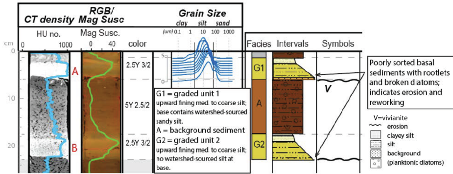
Figure 7. Deposit types A and B in the surface core SQBss (the surface sample at the location of cores SQB1 and SQB2). Facies types G1 and G2 are very similar, other than the presence of a thin layer of sandy silt at the base of deposit A. The bases of each deposit are poorly sorted and coarse-grained, containing rootlets and broken diatoms, indicative of erosion and reworking. Deposits are upward fining, with a clayey silt cap.
