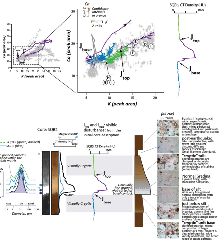
Figure 20. Deposit J is a complex sequence with cryptic components. Upper panel: The gap that exists between the initial and final ratios in the XRF scatterplot for deposit J can be filled in by including the sediment below (shown in blue) and by interpreting the upper portion to be a long tail (shown in green). XRF calcium and potassium confidence intervals (inset in blow-up of the scatterplot, centre top) were produced by repeatedly measuring the same section of core. The cryptic components of deposit J meet close to the initial positions of deposits G, H and I. The base of the visible silt unit is slightly enriched in calcium relative to background and is very well-sorted and fine-grained. This unit appears to "bleed down" from the clastic base into the very fine, organic-rich sediment below suggesting loading which can result when dense sediment
