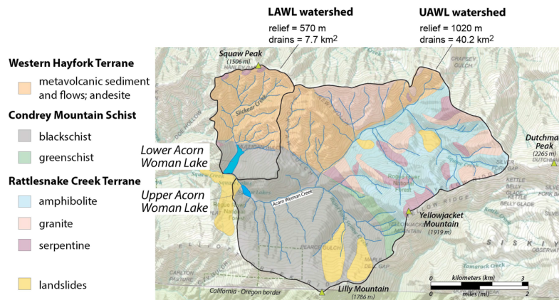
Figure 2. Geologic and Geomorphic Setting. Upper and Lower Acorn Woman Lakes are situated in the Condrey Mountain Schist; however, the bedrock of the lake catchments consists of distinctive metamorphic and plutonic lithologies. Note the large landslide responsible for lake creation. Geology from Donato, 1993.
